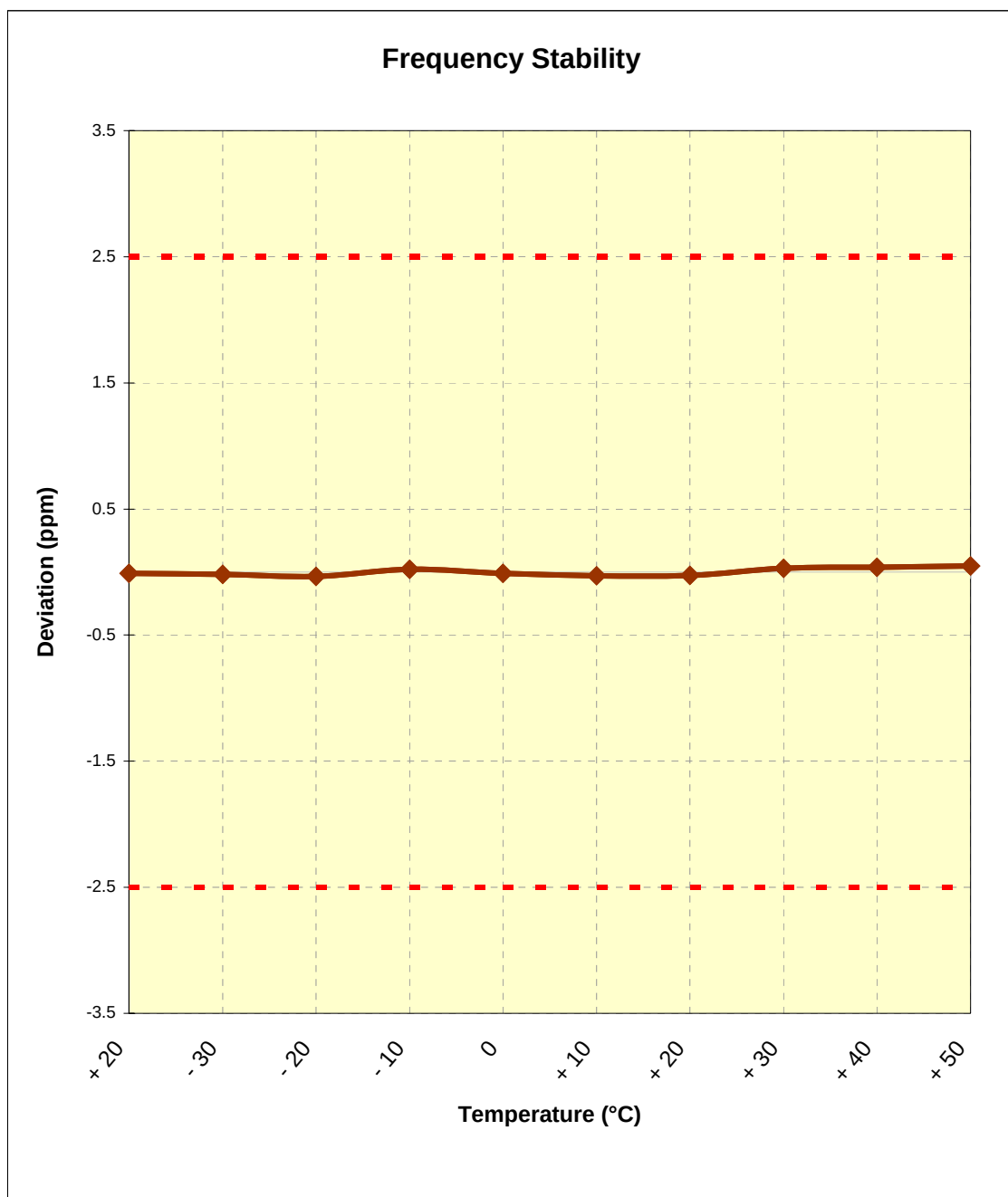
Figure 6-2. Frequency Stability Graph (Cellular GSM Mode – Ch. 190)
