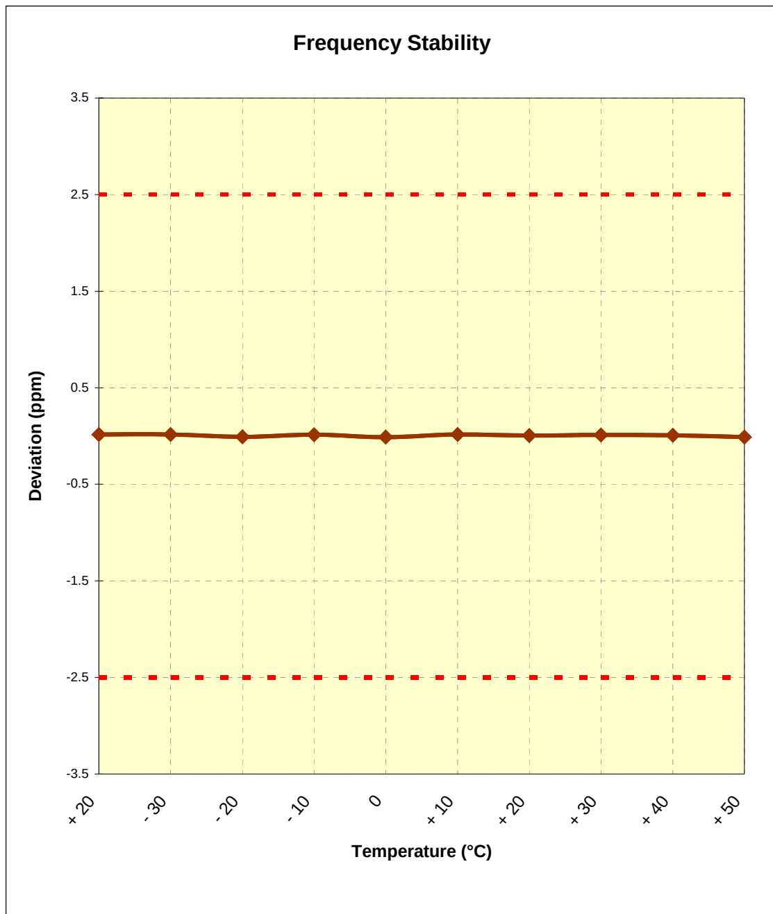
Figure 6-6. Frequency Stability Graph (PCS WCDMA Mode – Ch. 9400)
