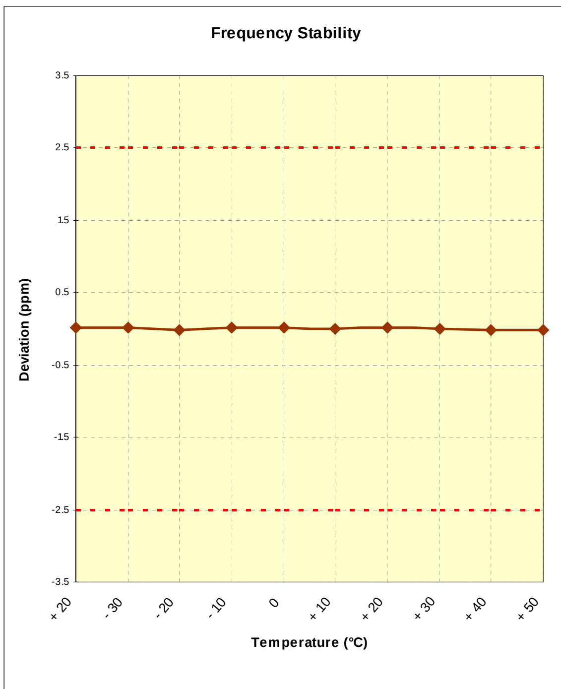
Figure 6-7. Frequency Stability Graph (PCS CDMA Mode – Ch. 600)
