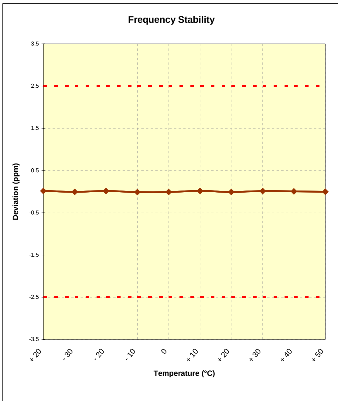
Figure 6-5. Frequency Stability Graph (PCS GSM Mode – Ch. 661)
