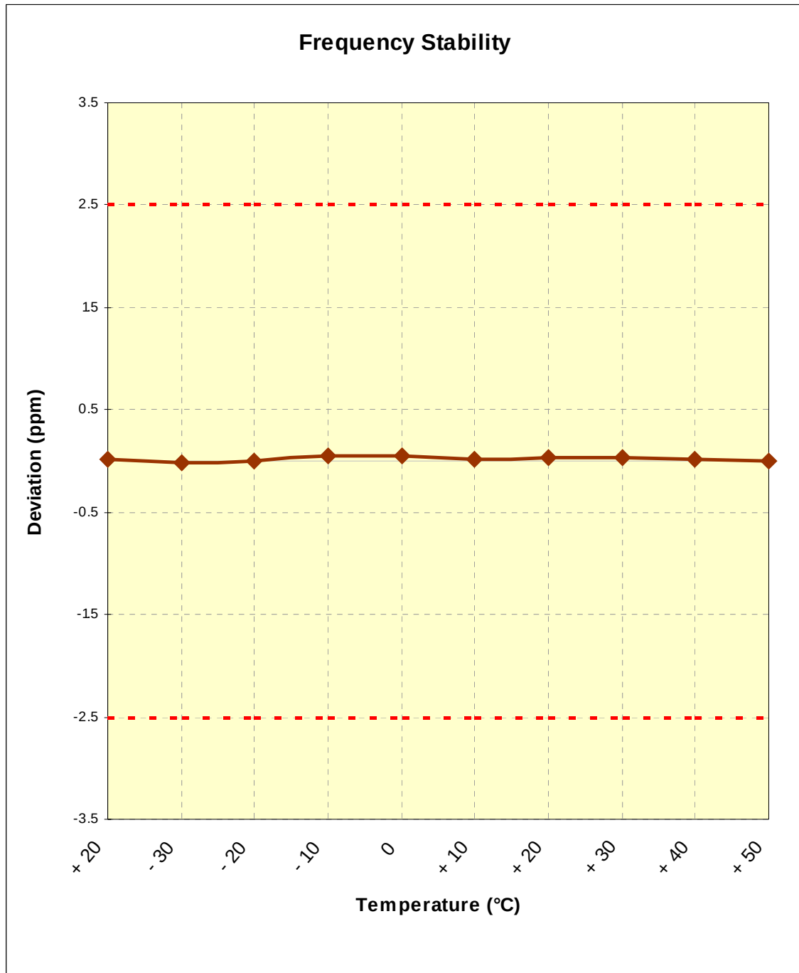
Figure 6-4. Frequency Stability Graph (Cellular CDMA Mode – Ch. 384)
