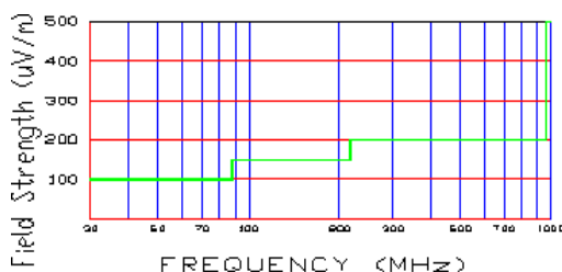
Figure 6-8. 3-Meter Limits
