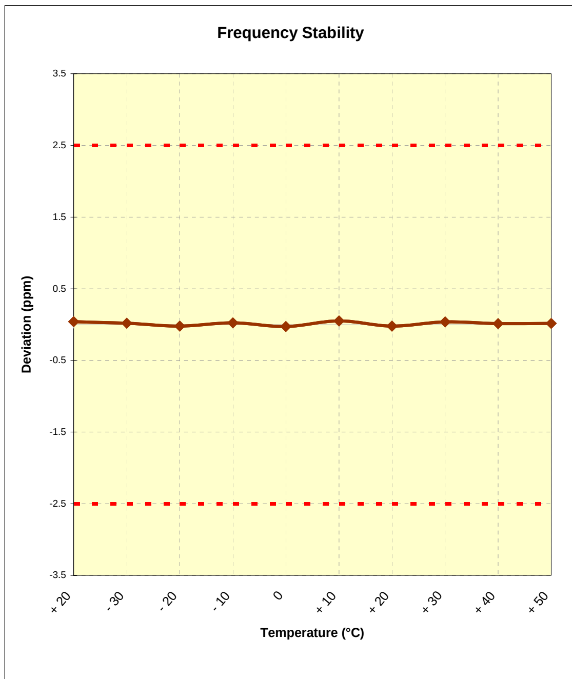
Figure 6-3. Frequency Stability Graph (Cellular WCDMA Mode – Ch. 4183)
