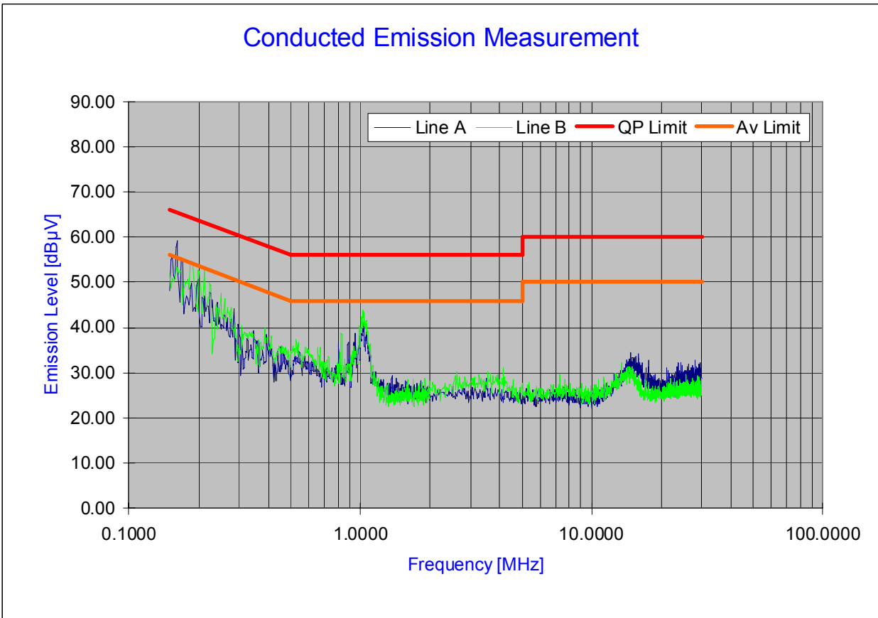
Plot 6-22. Line Conducted Plot with 802.11g
