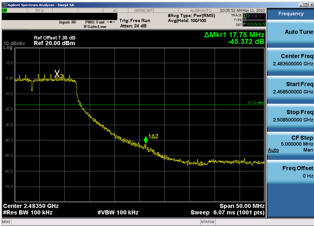
Plot 6-12. Band Edge Plot at 6.5/7.2Mbps (MCS0) (802.11n (20MHz) – Ch. 11)
