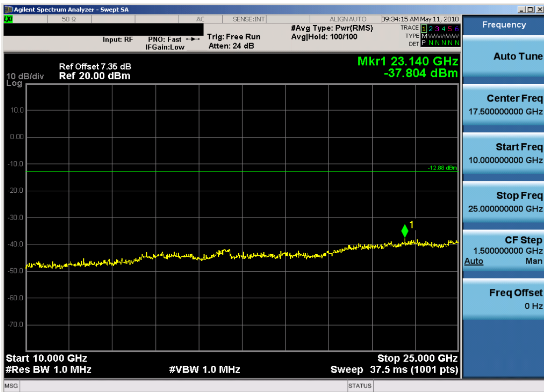
Plot 6-20. Conducted Spurious Plot at 2Mbps (802.11b – Ch. 11)
