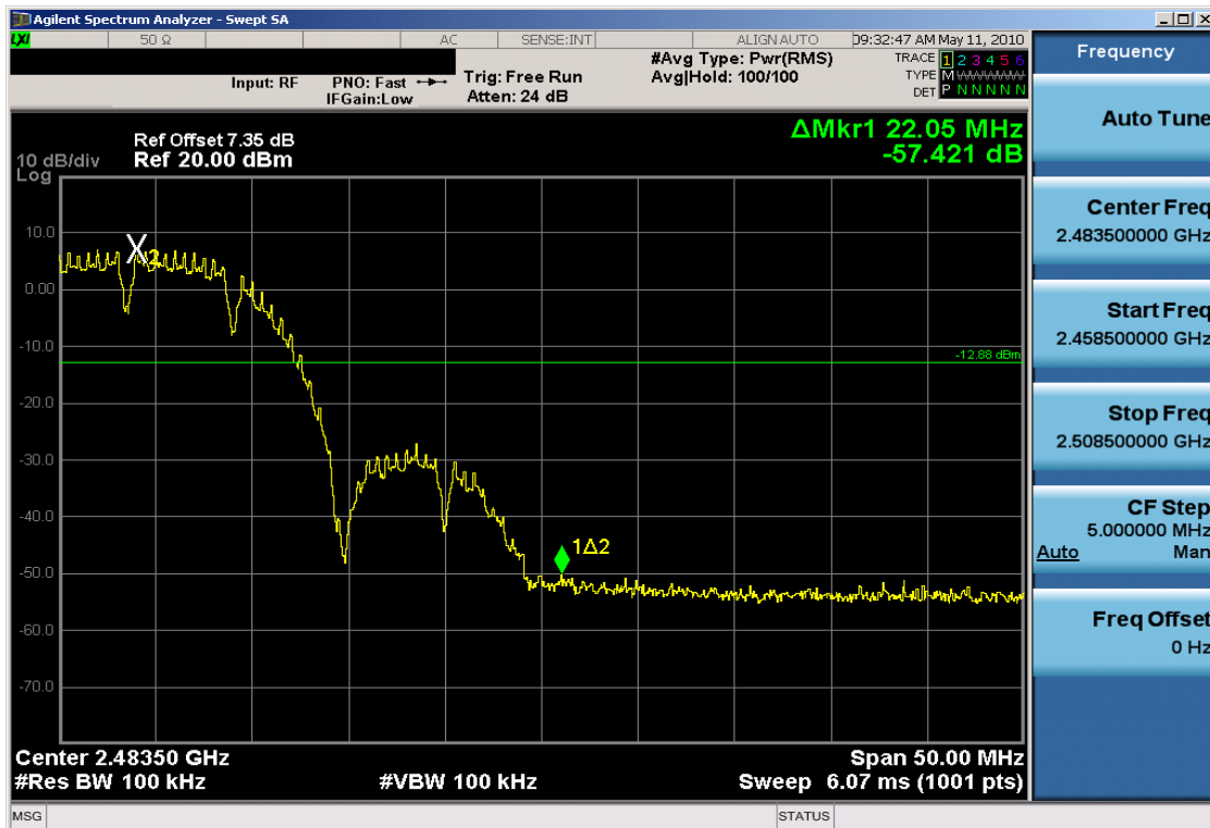
Plot 6-8. Band Edge Plot at 2Mbps (802.11b – Ch. 11)
