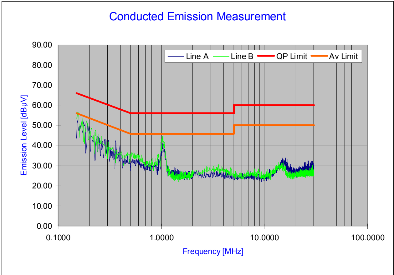
Plot 6-23. Line Conducted Plot with 802.11n
