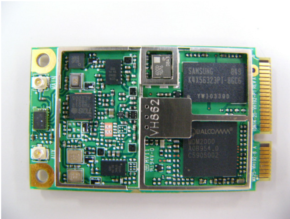
WWAN Module Interior Top View
