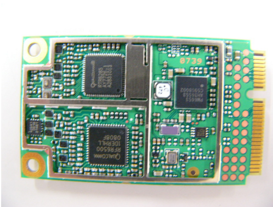
WWAN Module Interior Bottom View
