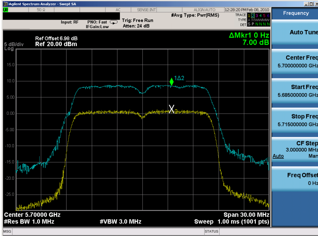
Plot 6-88. Peak Excursion Ratio Plot (802.11a (UNII) – Ch. 140) – Chain B
