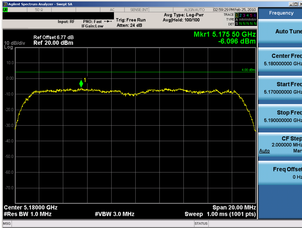
Plot 6-59. Peak Power Spectral Density (802.11a Dual Transmit Mode – Ch. 36) – Chain B
