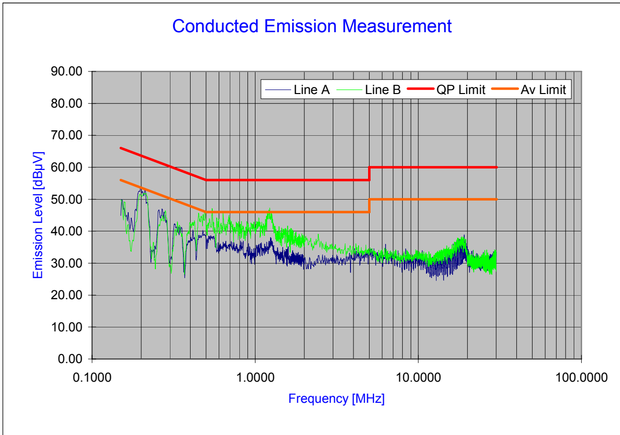
Plot 6-99. Line Conducted Plot with 802.11n (UNII Band I)
