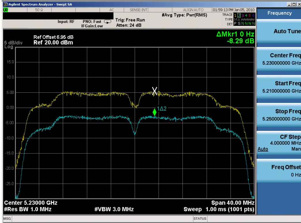
Plot 6-74. Peak Excursion Ratio Plot (802.11n (UNII) – Ch. 46) – Chain A
