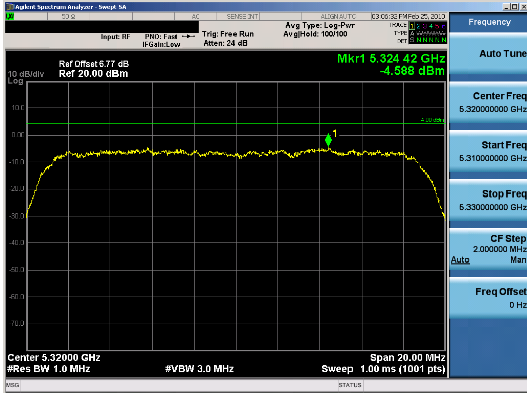
Plot 6-61. Peak Power Spectral Density (802.11a Dual Transmit Mode – Ch. 64) – Chain B
