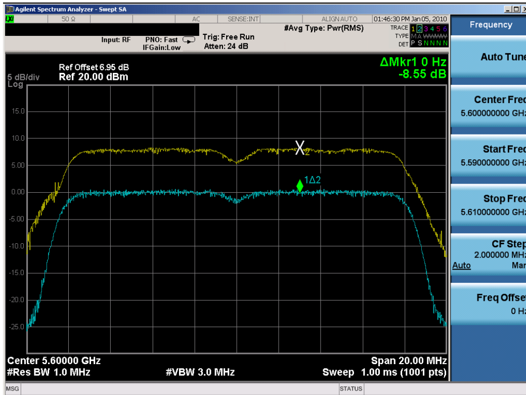
Plot 6-71. Peak Excursion Ratio Plot (802.11a (UNII) – Ch. 120) – Chain A
