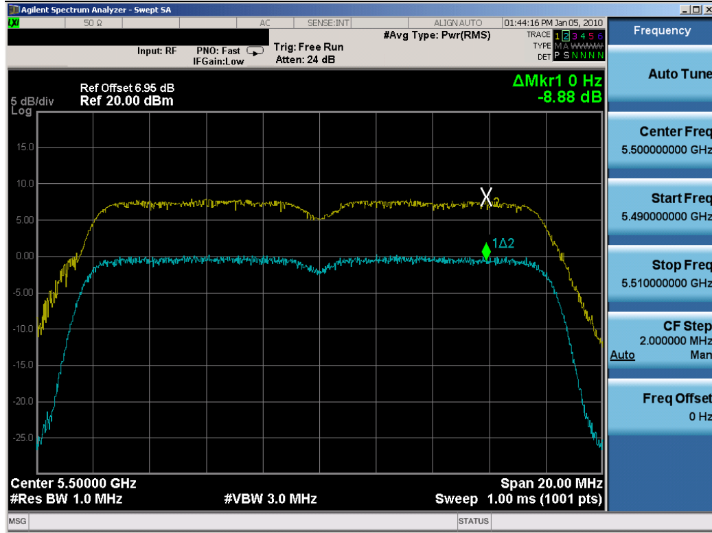
Plot 6-70. Peak Excursion Ratio Plot (802.11a (UNII) – Ch. 100) – Chain A
