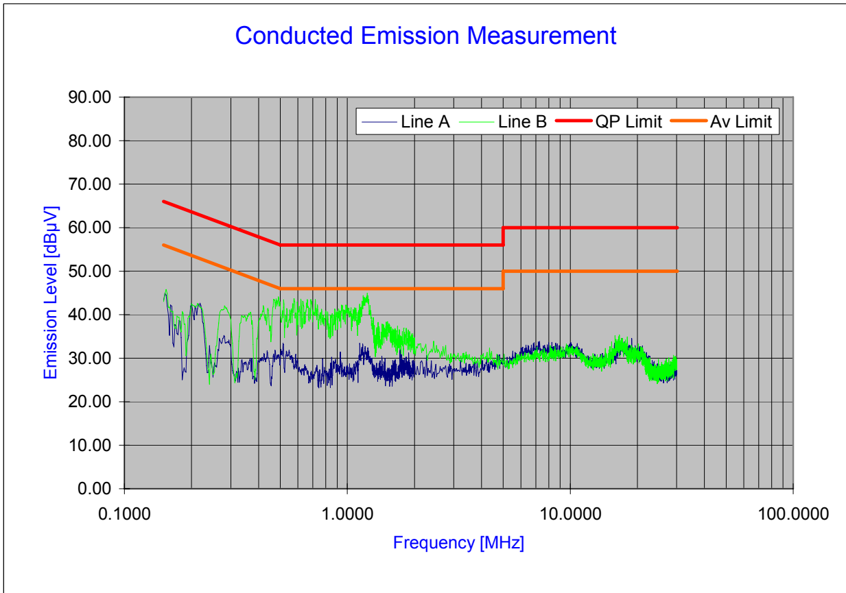
Plot 6-101. Line Conducted Plot with 802.11n (UNII Band III)
