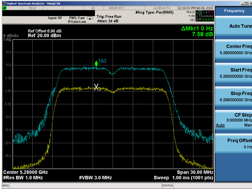
Plot 6-84. Peak Excursion Ratio Plot (802.11a (UNII) – Ch. 56) – Chain B
