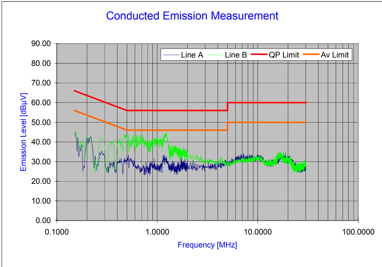
Plot 6-98. Line Conducted Plot with 802.11a (UNII Band III)
