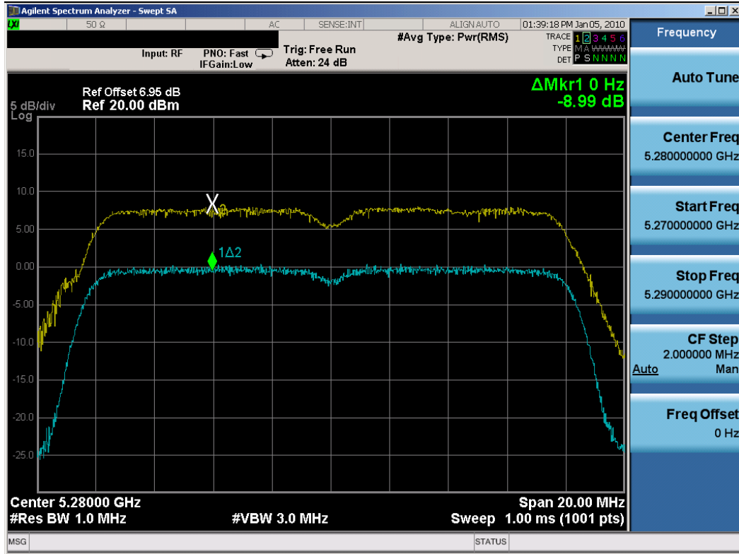
Plot 6-68. Peak Excursion Ratio Plot (802.11a (UNII) – Ch. 56) – Chain A
