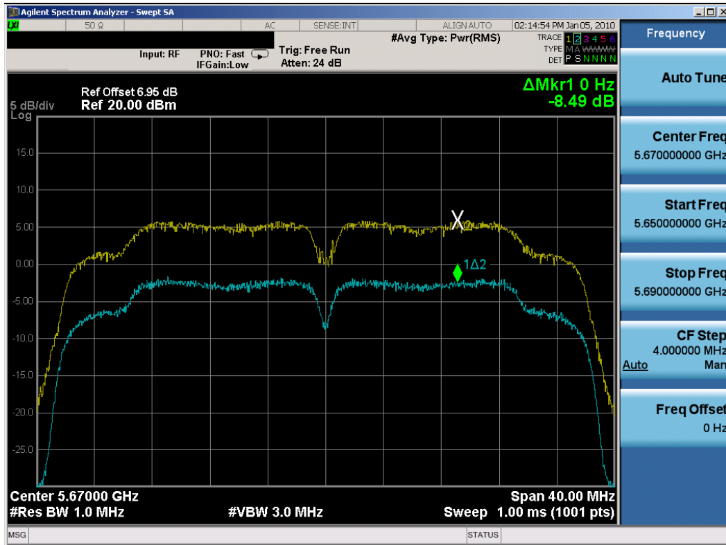
Plot 6-79. Peak Excursion Ratio Plot (802.11n (UNII) – Ch. 134) – Chain A
