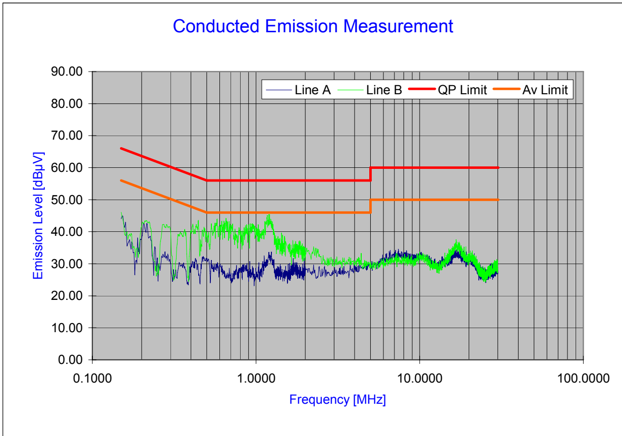
Plot 6-97. Line Conducted Plot with 802.11a (UNII Band II)
