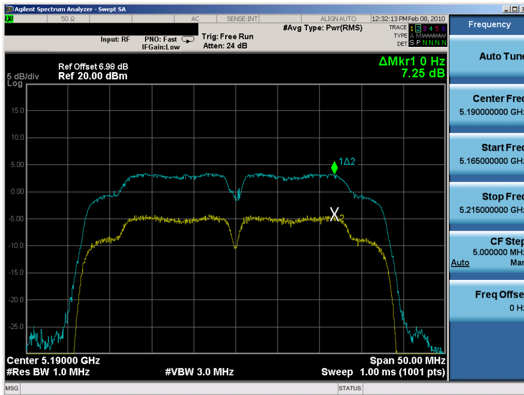
Plot 6-89. Peak Excursion Ratio Plot (802.11n (UNII) – Ch. 38) – Chain B
