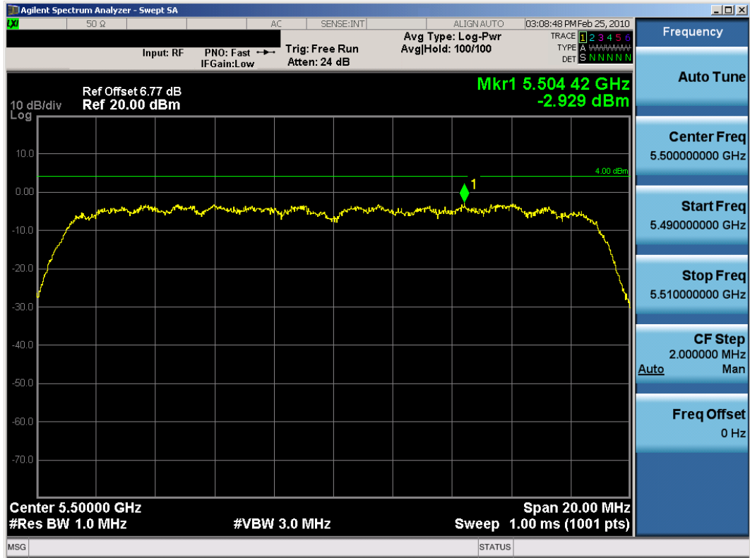
Plot 6-63. Peak Power Spectral Density (802.11a Dual Transmit Mode – Ch. 100) – Chain B
