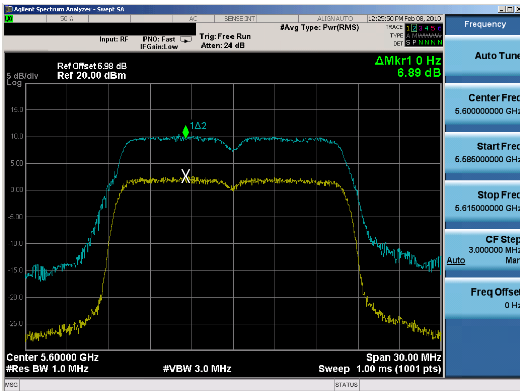
Plot 6-87. Peak Excursion Ratio Plot (802.11a (UNII) – Ch. 120) – Chain B
