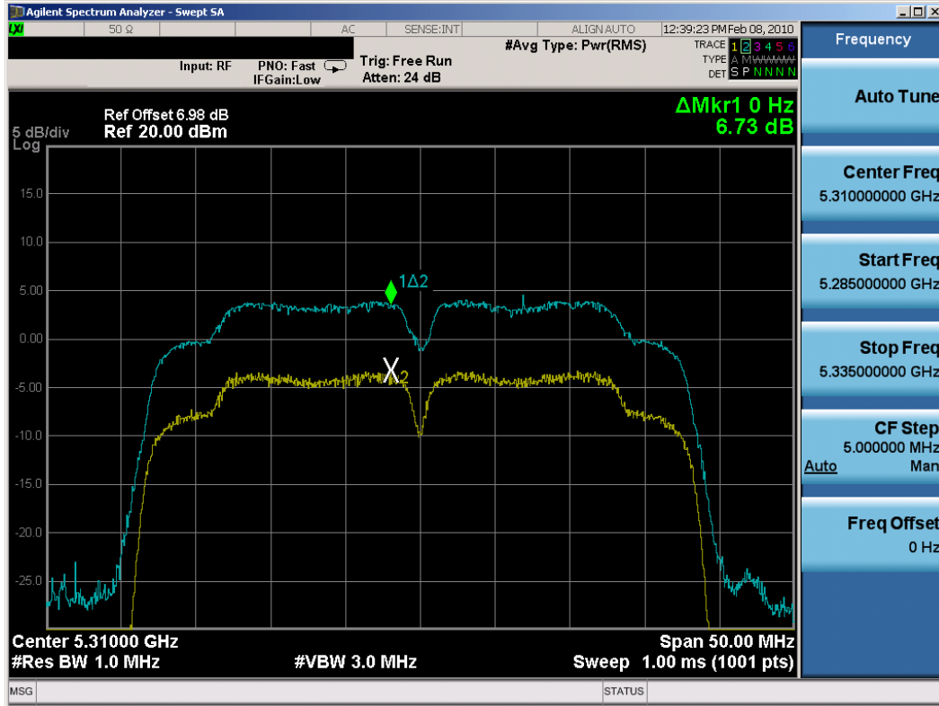
Plot 6-92. Peak Excursion Ratio Plot (802.11n (UNII) – Ch. 62) – Chain B
