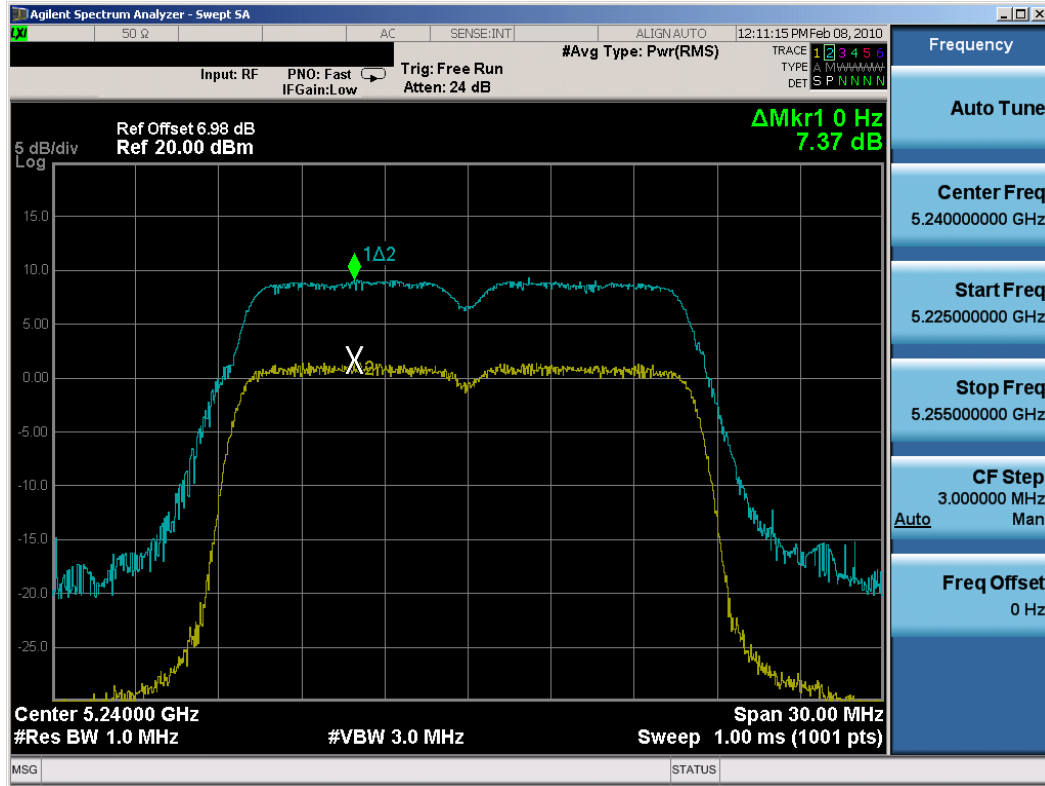
Plot 6-82. Peak Excursion Ratio Plot (802.11a (UNII) – Ch. 48) – Chain B
