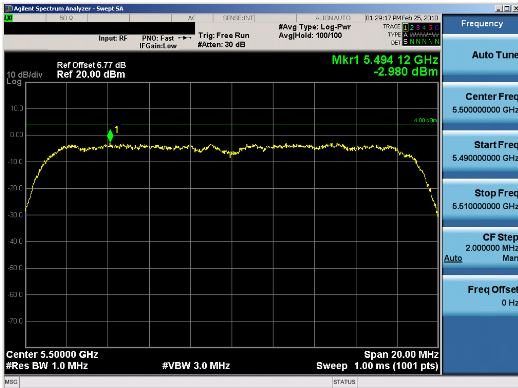
Plot 6-62. Peak Power Spectral Density (802.11a Dual Transmit Mode – Ch. 100) – Chain A
