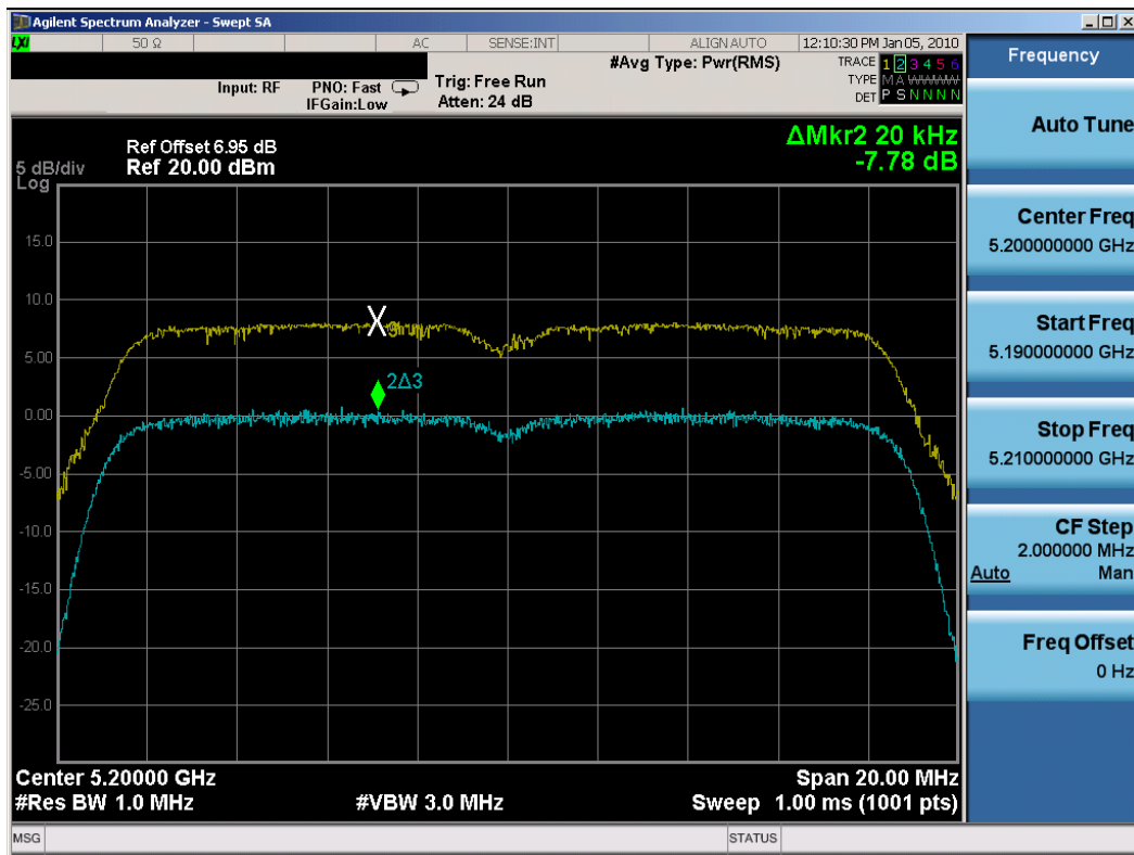
Plot 6-65. Peak Excursion Ratio Plot (802.11a (UNII) – Ch. 40) – Chain A
