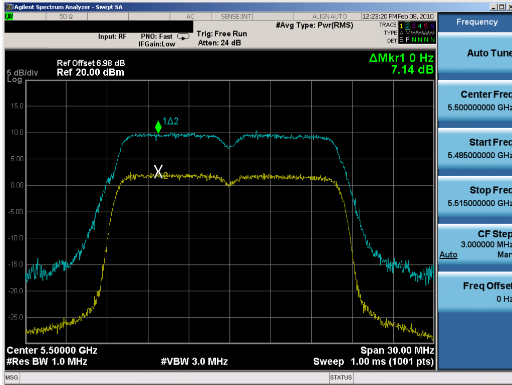
Plot 6-86. Peak Excursion Ratio Plot (802.11a (UNII) – Ch. 100) – Chain B
