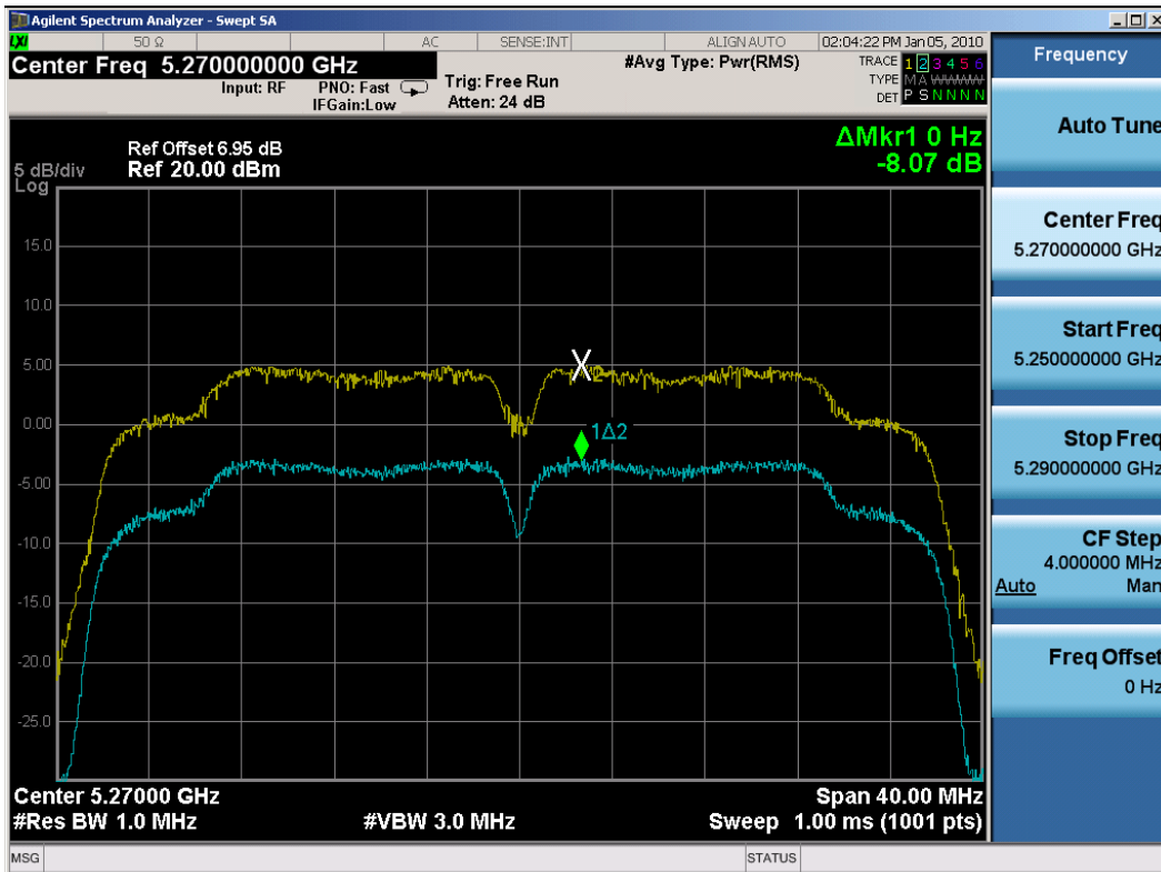
Plot 6-75. Peak Excursion Ratio Plot (802.11n (UNII) – Ch. 54) – Chain A
