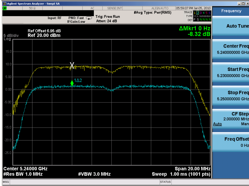
Plot 6-66. Peak Excursion Ratio Plot (802.11a (UNII) – Ch. 48) – Chain A
