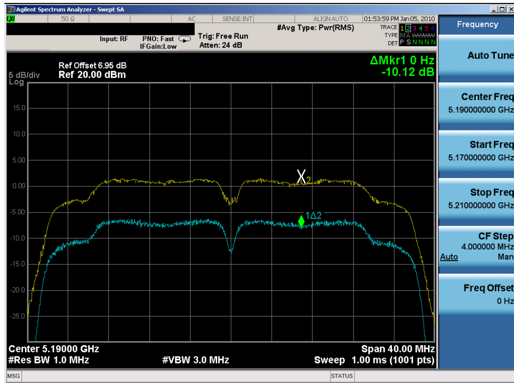
Plot 6-73. Peak Excursion Ratio Plot (802.11n (UNII) – Ch. 38) – Chain A
