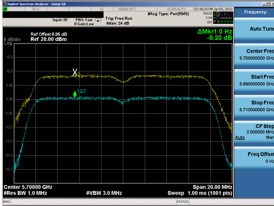
Plot 6-72. Peak Excursion Ratio Plot (802.11a (UNII) – Ch. 140) – Chain A
