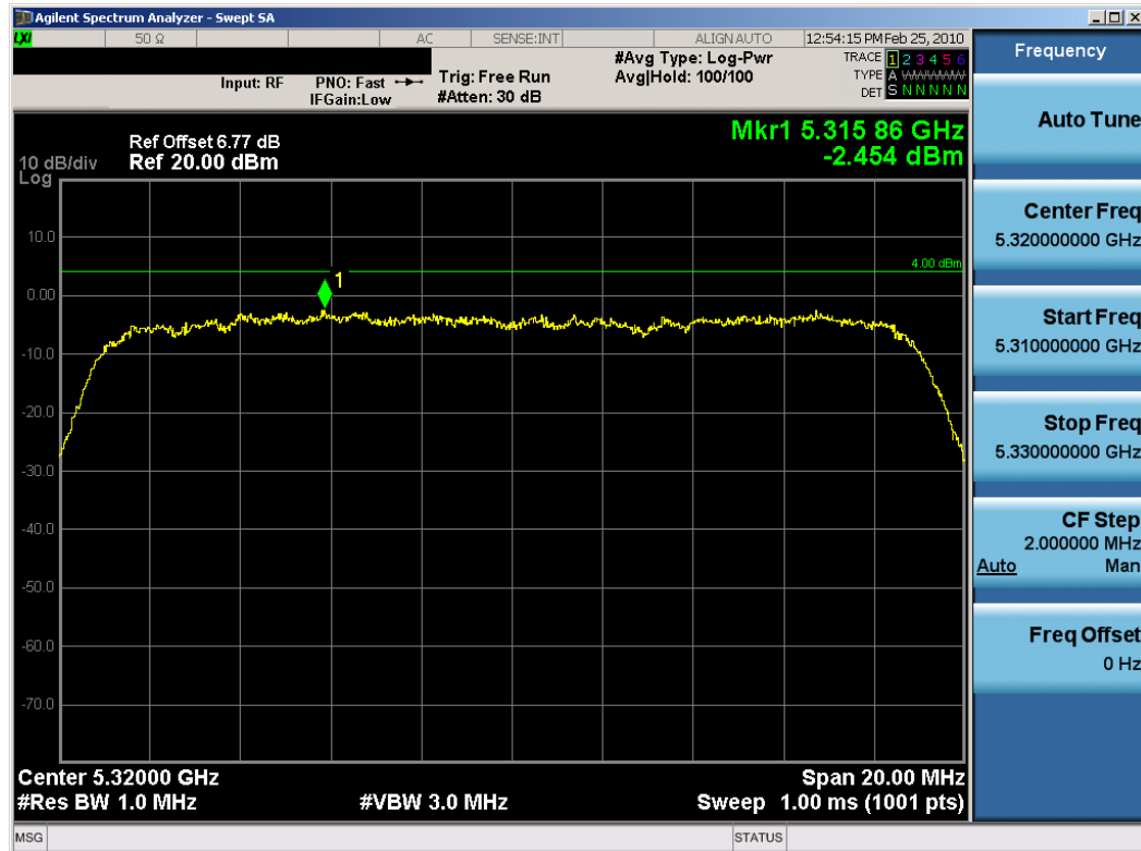
Plot 6-60. Peak Power Spectral Density (802.11a Dual Transmit Mode – Ch. 64) – Chain A
