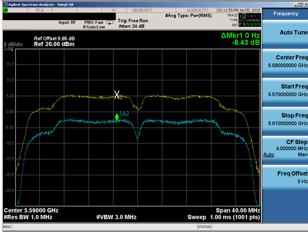
Plot 6-78. Peak Excursion Ratio Plot (802.11n (UNII) – Ch. 118) – Chain A
