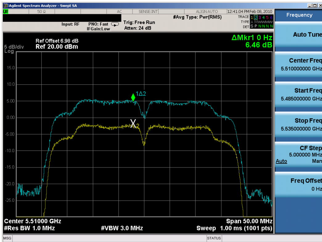
Plot 6-93. Peak Excursion Ratio Plot (802.11n (UNII) – Ch. 102) – Chain B
