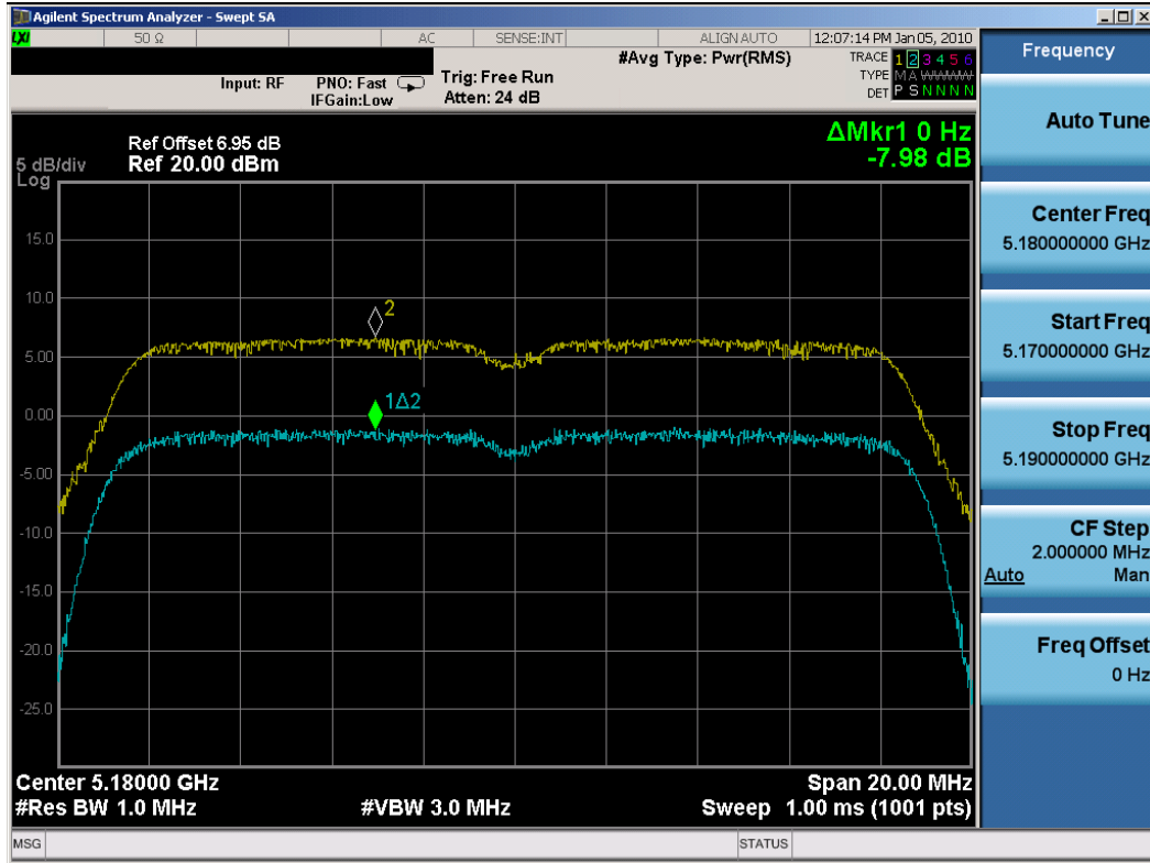
Plot 6-64. Peak Excursion Ratio Plot (802.11a (UNII) – Ch. 36) – Chain A
