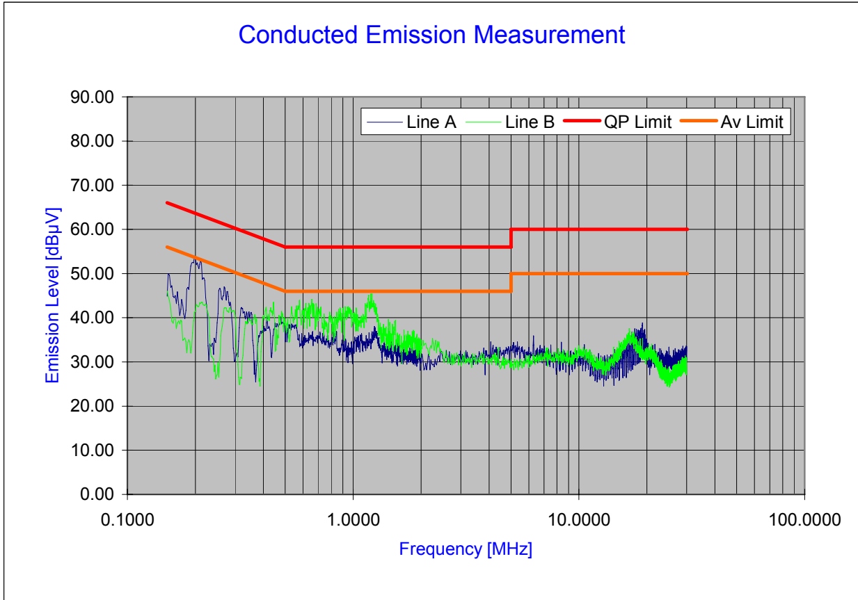
Plot 6-96. Line Conducted Plot with 802.11a (UNII Band I)
