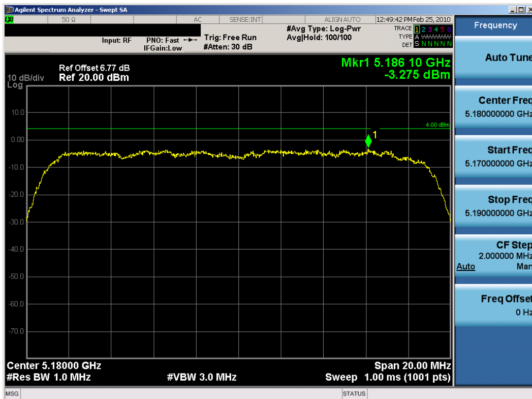
Plot 6-58. Peak Power Spectral Density (802.11a Dual Transmit Mode – Ch. 36) – Chain A
