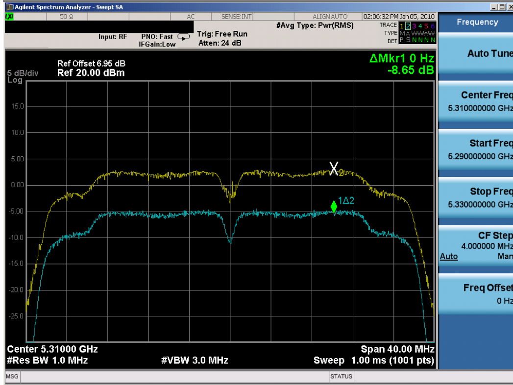
Plot 6-76. Peak Excursion Ratio Plot (802.11n (UNII) – Ch. 62) – Chain A
