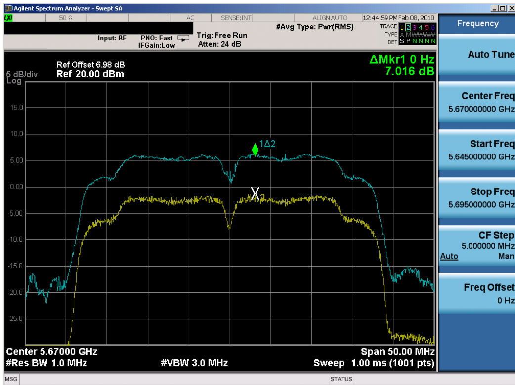
Plot 6-95. Peak Excursion Ratio Plot (802.11n (UNII) – Ch. 134) – Chain B
