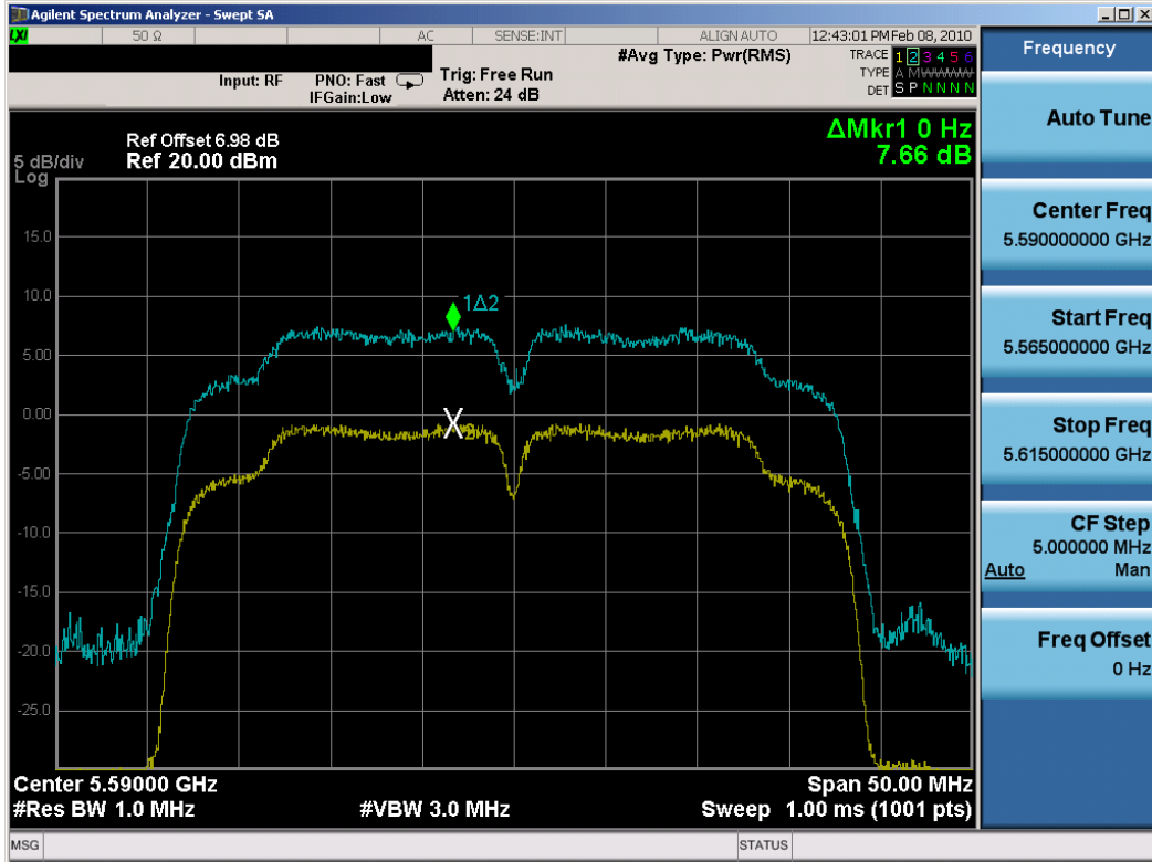
Plot 6-94. Peak Excursion Ratio Plot (802.11n (UNII) – Ch. 118) – Chain B
