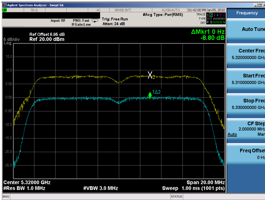
Plot 6-69. Peak Excursion Ratio Plot (802.11a (UNII) – Ch. 64) – Chain A
