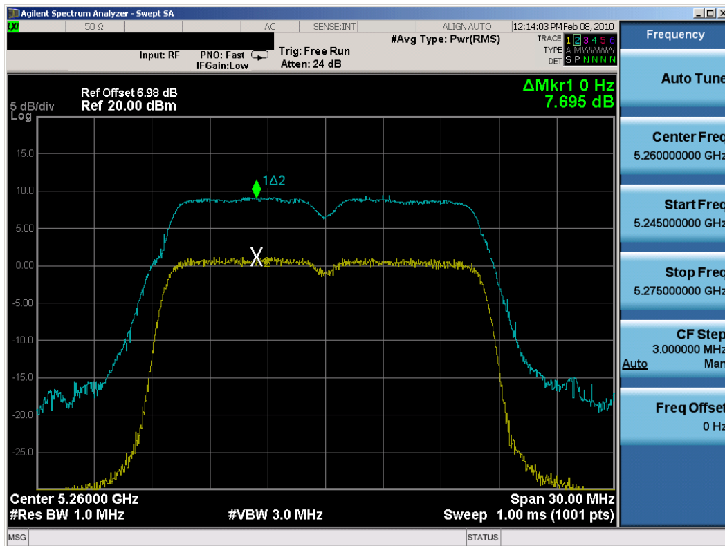
Plot 6-83. Peak Excursion Ratio Plot (802.11a (UNII) – Ch. 52) – Chain B
