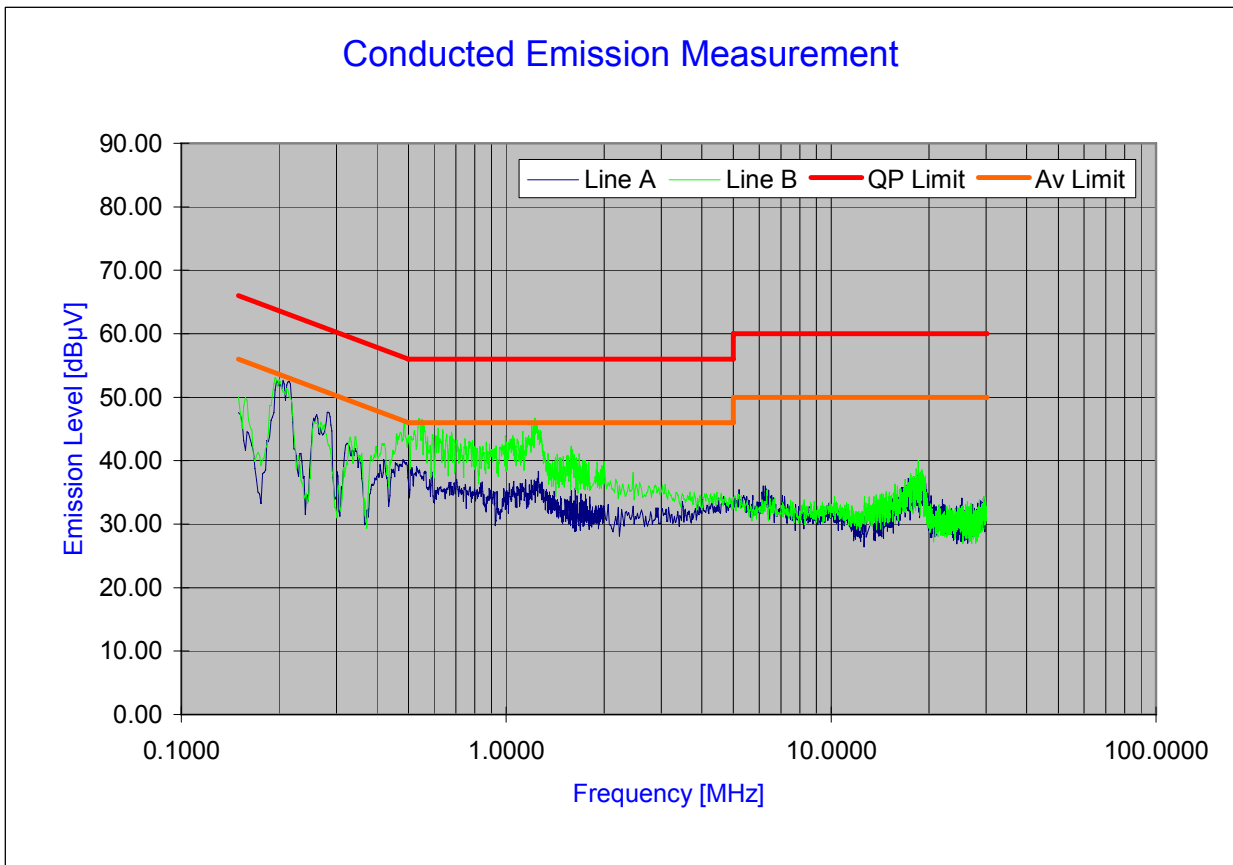
Plot 6-100. Line Conducted Plot with 802.11n (UNII Band II)
