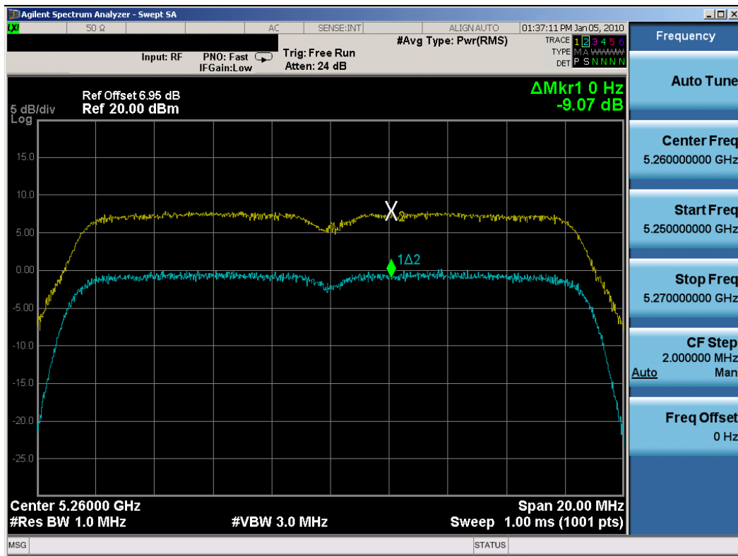
Plot 6-67. Peak Excursion Ratio Plot (802.11a (UNII) – Ch. 52) – Chain A
