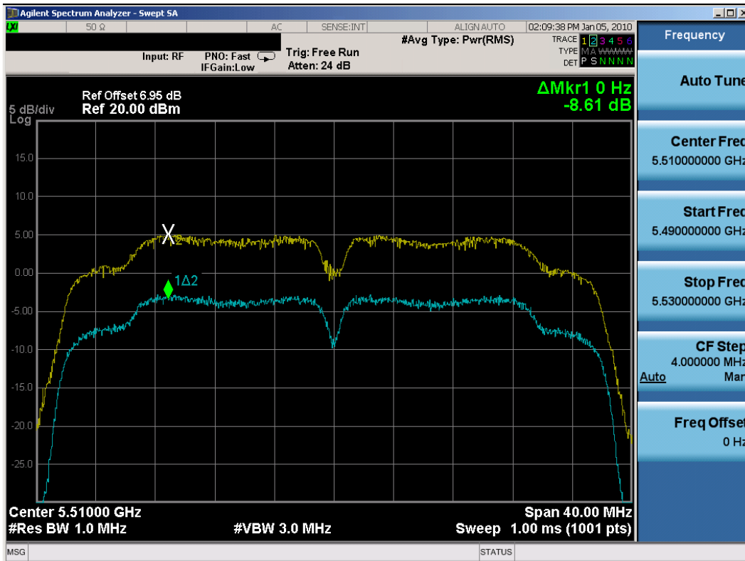
Plot 6-77. Peak Excursion Ratio Plot (802.11n (UNII) – Ch. 102) – Chain A
