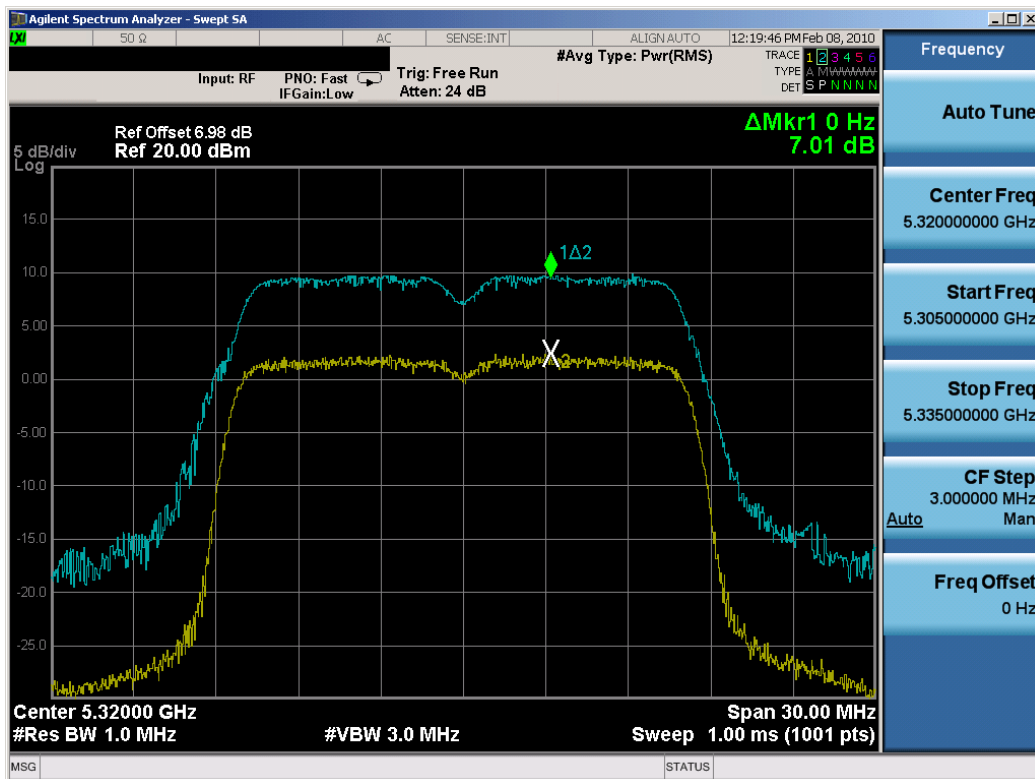
Plot 6-85. Peak Excursion Ratio Plot (802.11a (UNII) – Ch. 64) – Chain B
