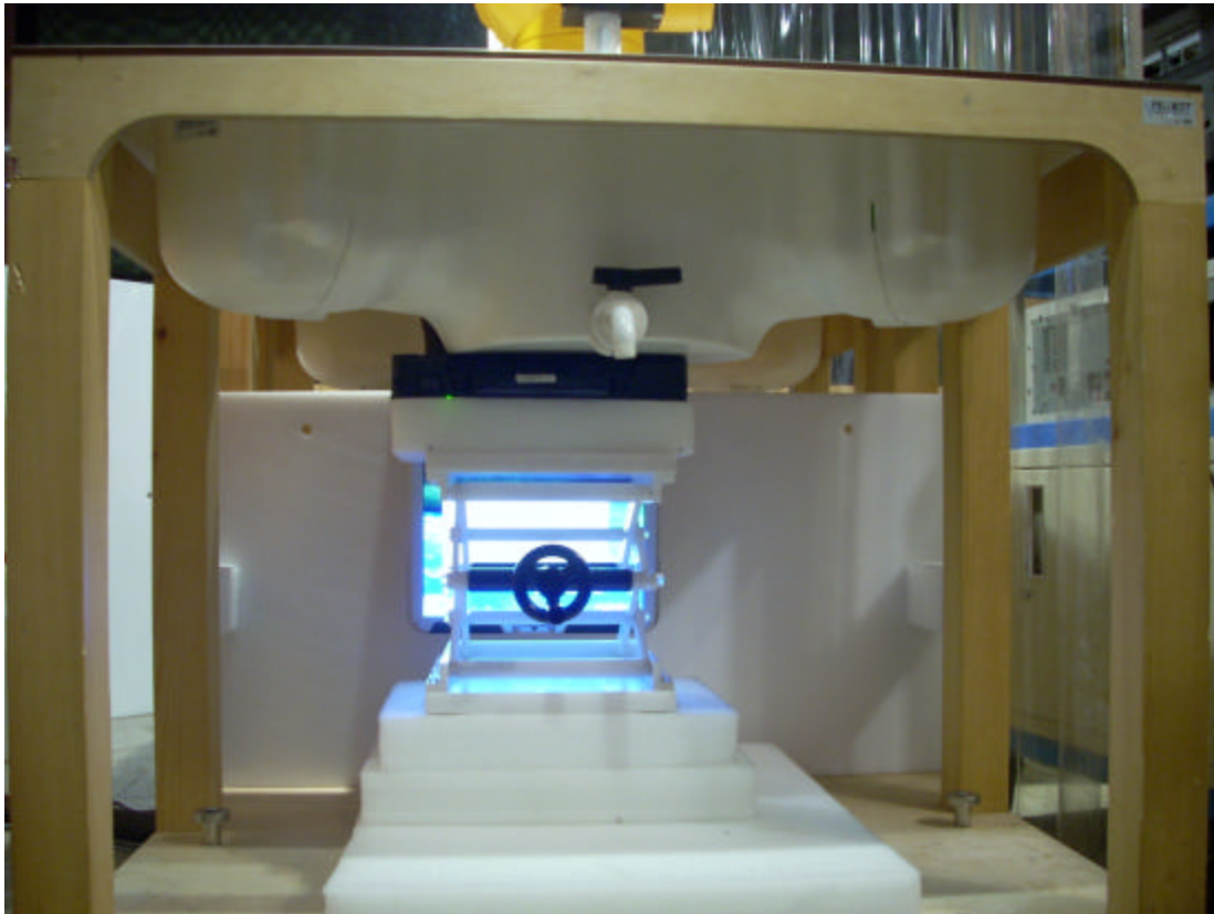
Figure 1: Body SAR – Lap Position
