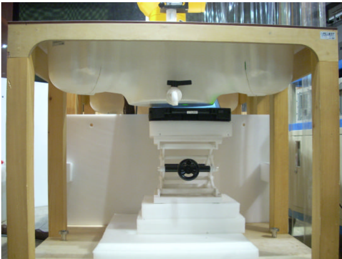
Figure 4: Body SAR- Top side with 1.0 cm space
