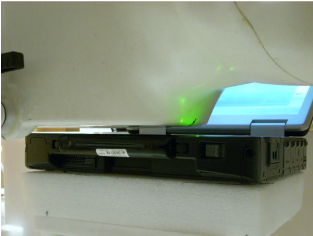
Figure 6: Top Position with 1.0 cm Space
