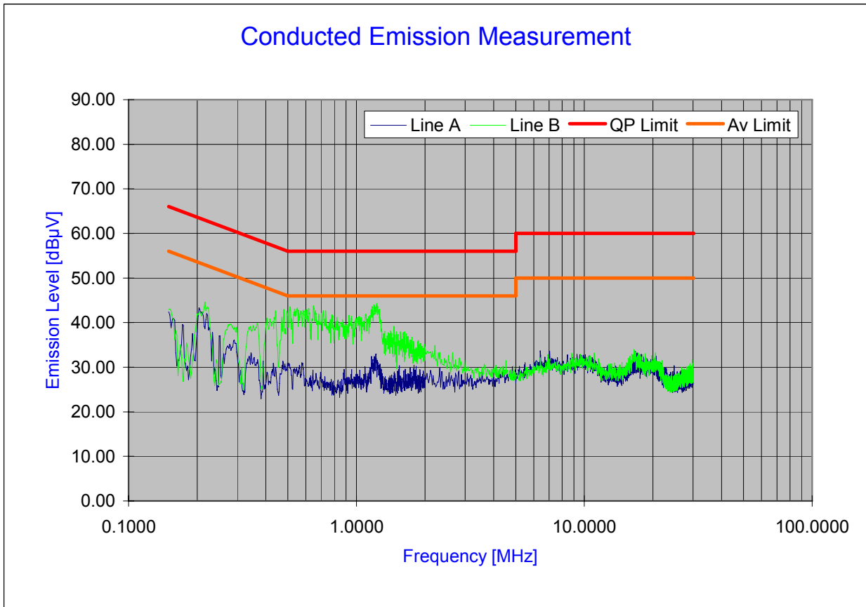
Plot 6-112. Line Conducted Plot with 802.11b
