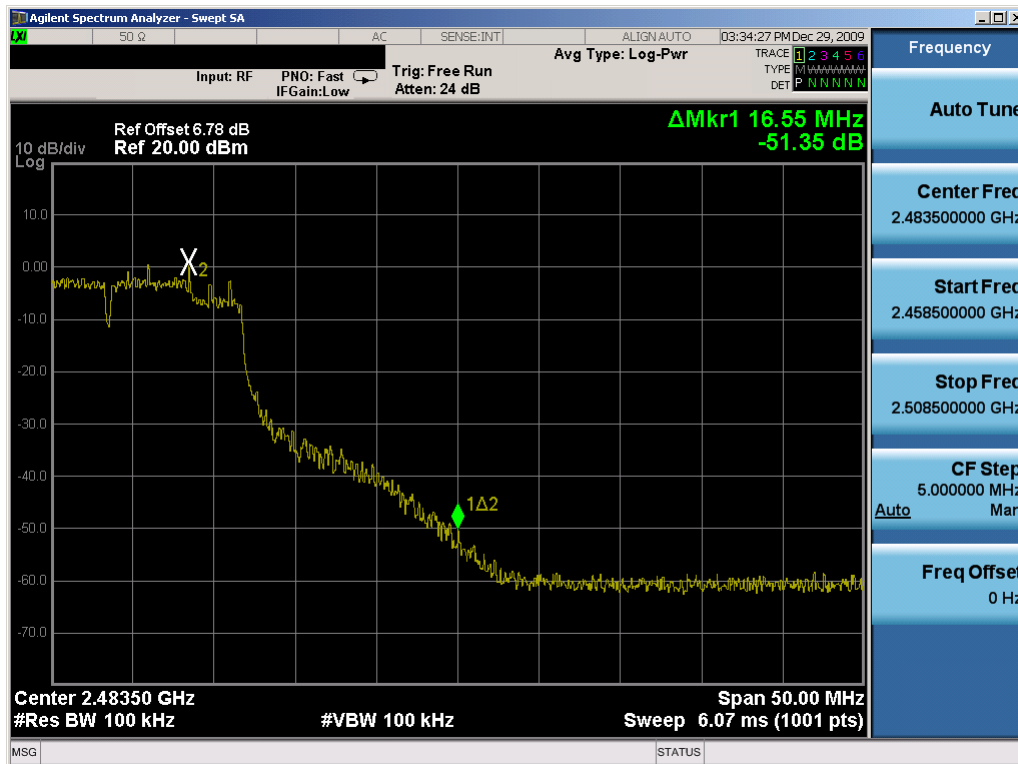
Plot 6-68. Band Edge Plot (802.11g – Ch. 11) – Chain A
