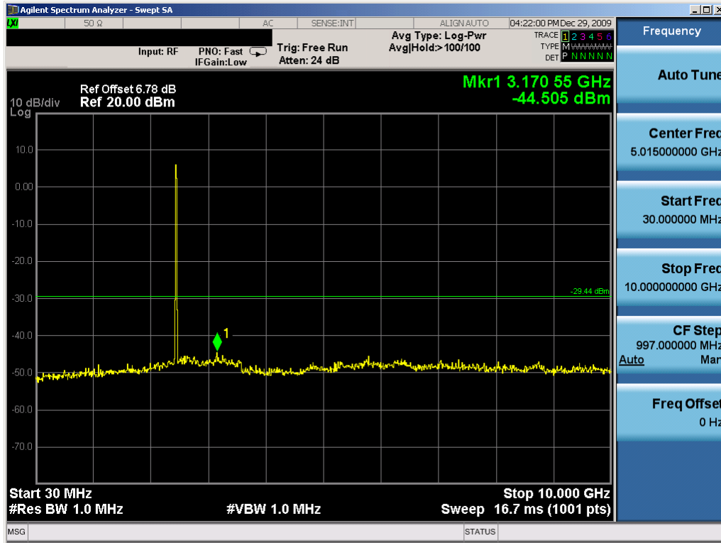
Plot 6-89. Conducted Spurious Plot (802.11b – Ch. 11) – Chain A
