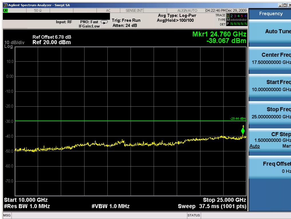
Plot 6-90. Conducted Spurious Plot (802.11b – Ch. 11) – Chain A
