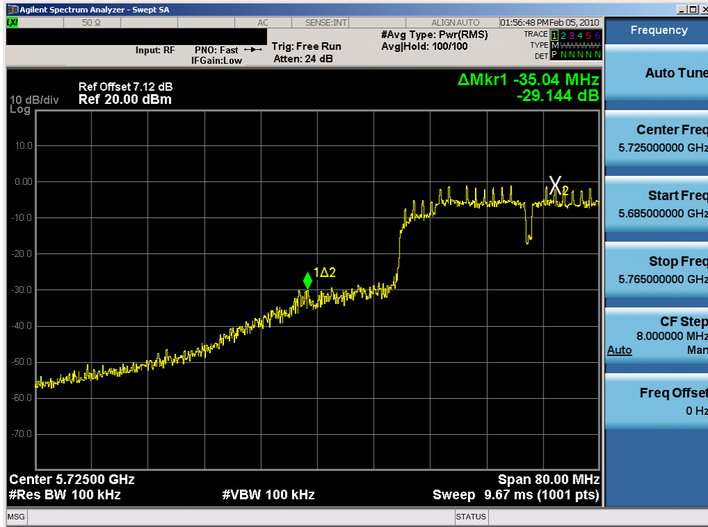
Plot 6-83. Band Edge Plot (802.11n (5.8GHz) – Ch. 151) – Chain B
