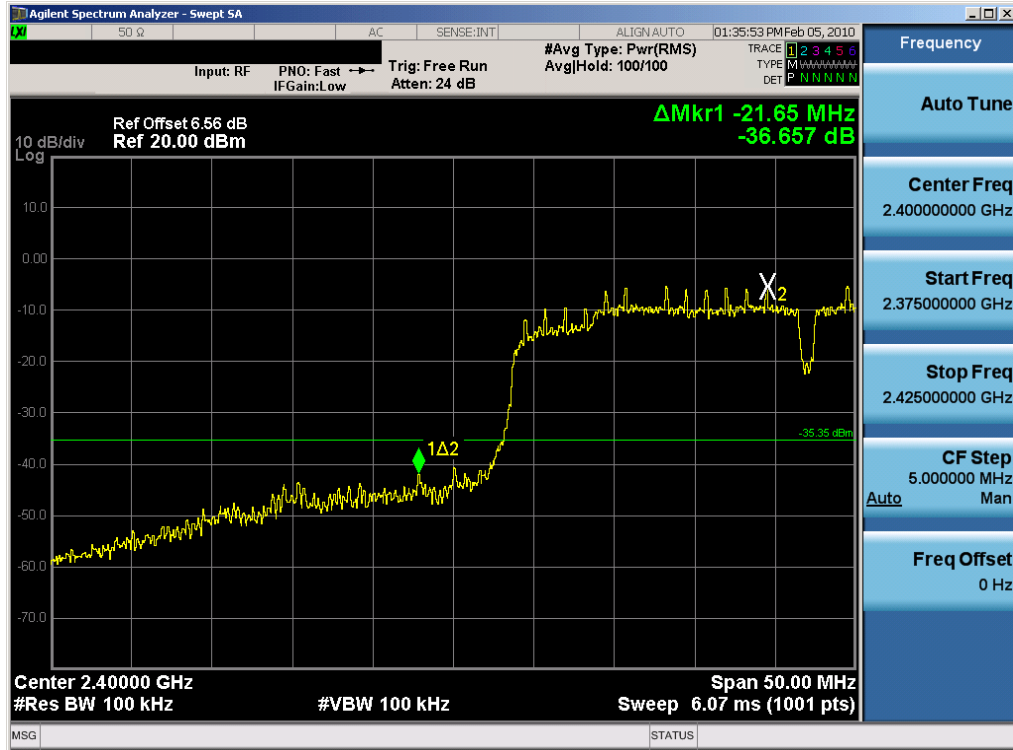
Plot 6-81. Band Edge Plot (802.11n (2.4GHz) – Ch. 3) – Chain B
