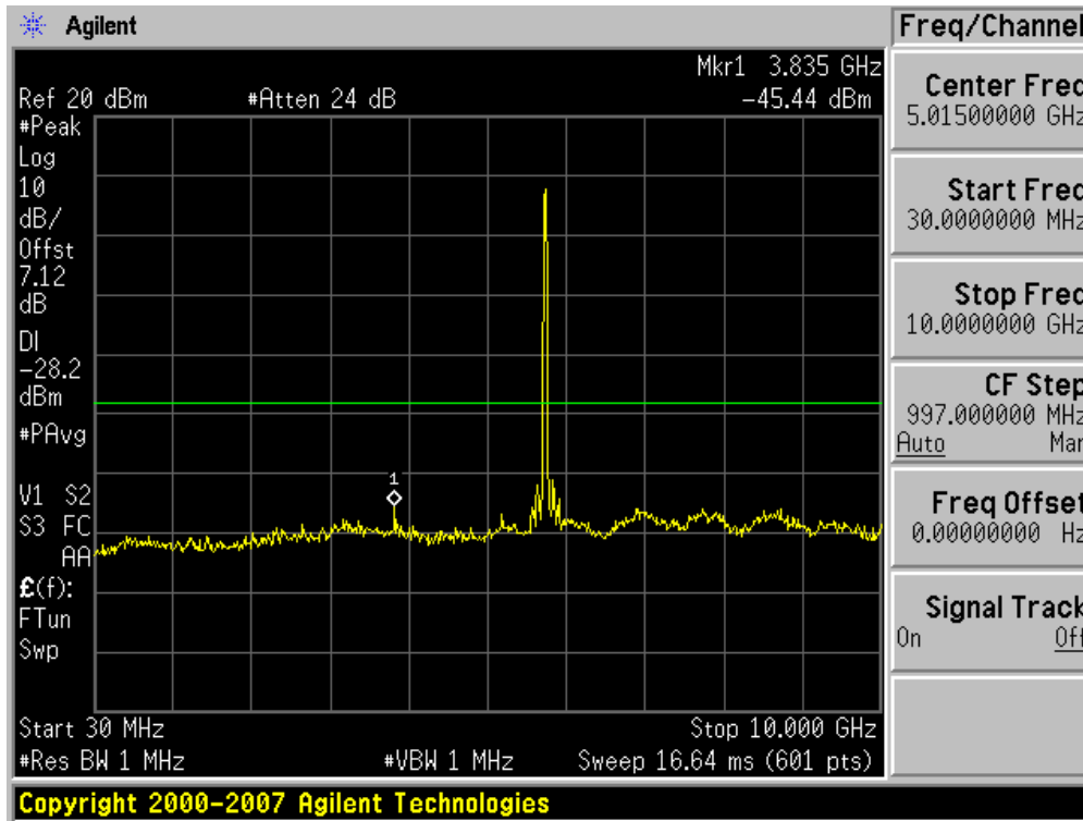
Plot 6-106. Conducted Spurious Plot (802.11a – Ch. 149) – Chain B
