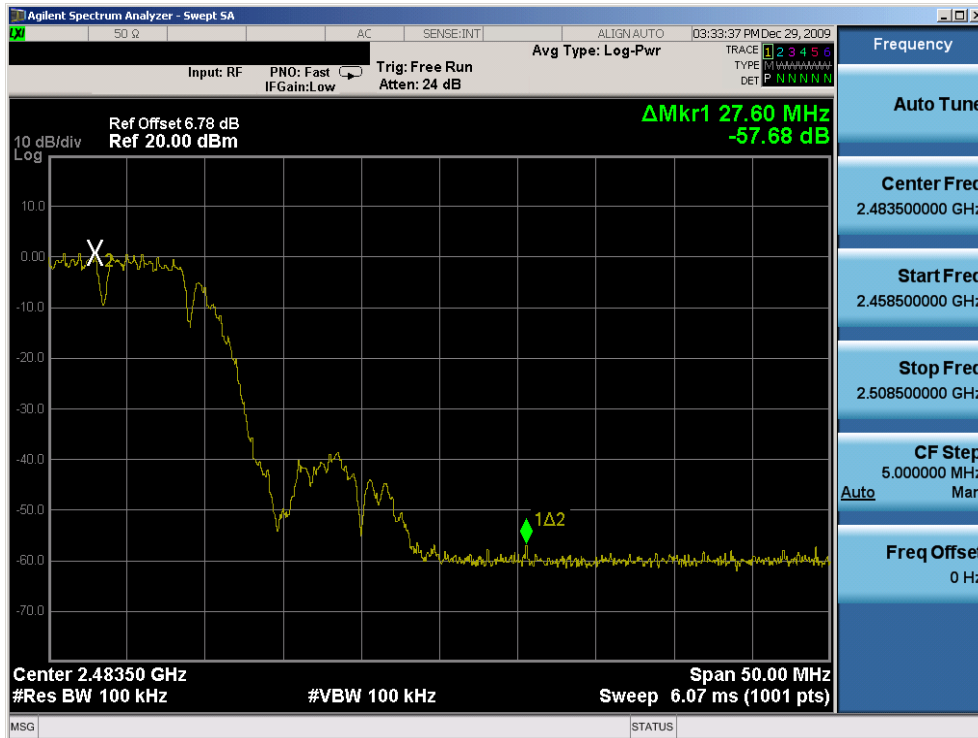
Plot 6-66. Band Edge Plot (802.11b – Ch. 11) – Chain A
