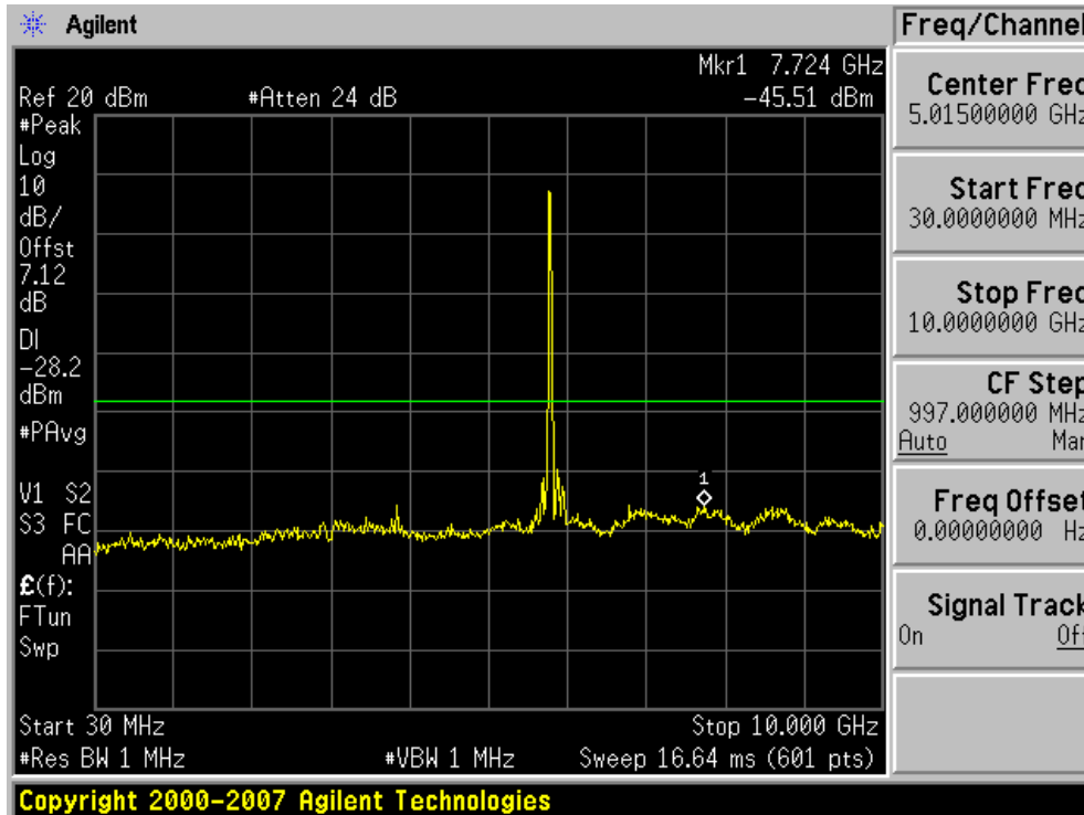
Plot 6-108. Conducted Spurious Plot (802.11a – Ch. 157) – Chain B
