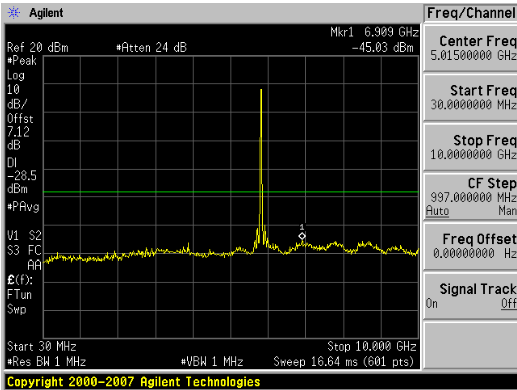
Plot 6-110. Conducted Spurious Plot (802.11a – Ch. 165) – Chain B
