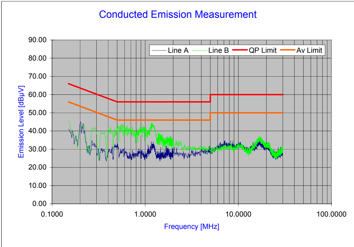
Plot 6-113. Line Conducted Plot with 802.11g
