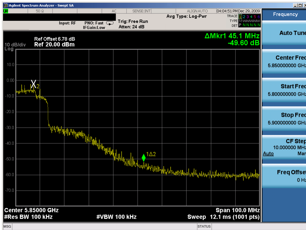
Plot 6-74. Band Edge Plot (802.11n (5.8GHz) – Ch. 159) – Chain A
