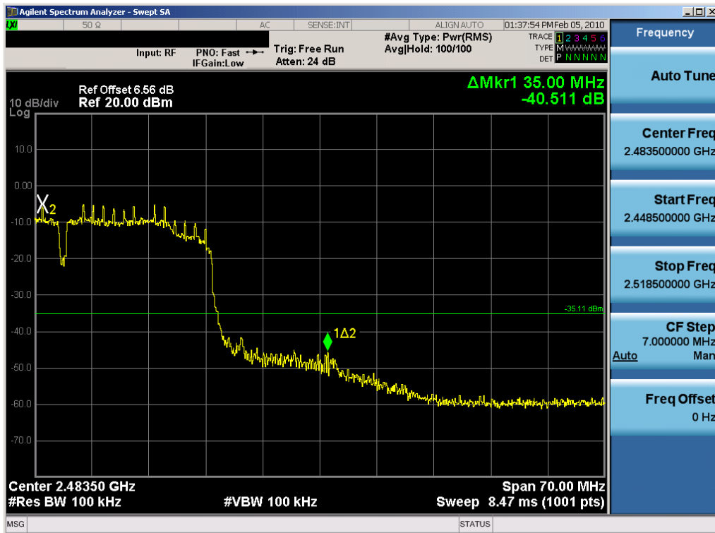
Plot 6-82. Band Edge Plot (802.11n (2.4GHz) – Ch. 9) – Chain B
