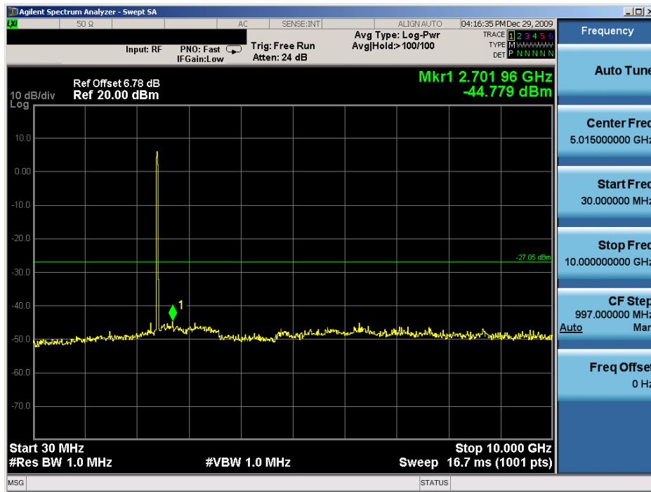
Plot 6-85. Conducted Spurious Plot (802.11b – Ch. 1) – Chain A
