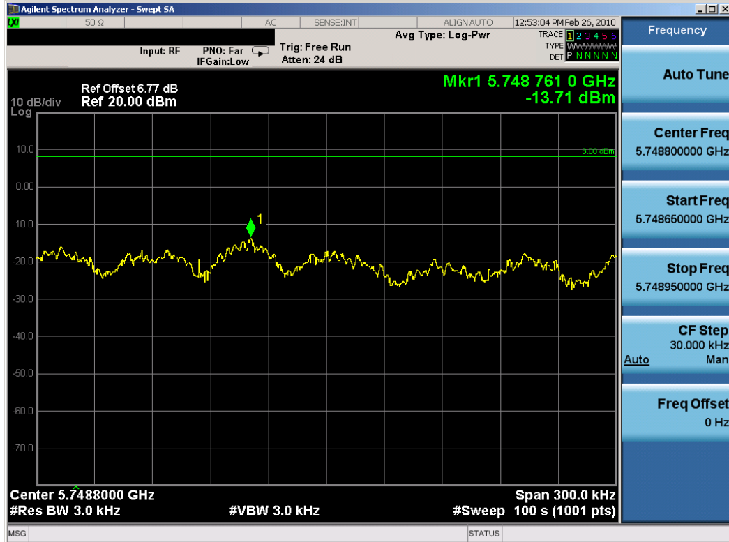
Plot 6-59. Power Spectral Density (802.11a Dual Transmit Mode – Ch. 149) – Chain A
