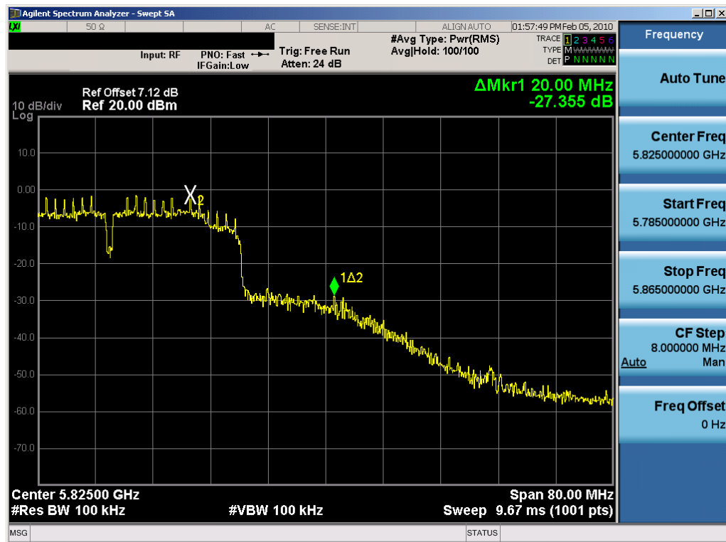
Plot 6-84. Band Edge Plot (802.11n (5.8GHz) – Ch. 159) – Chain B
