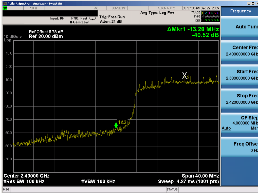
Plot 6-71. Band Edge Plot (802.11n (2.4GHz) – Ch. 3) – Chain A
