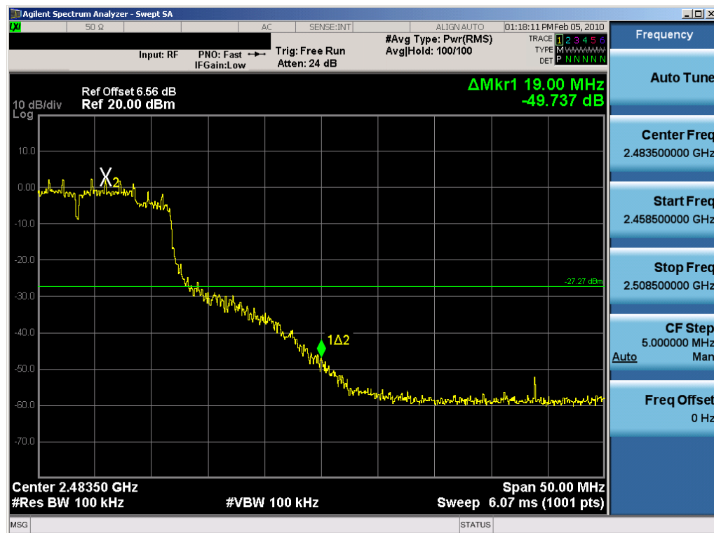
Plot 6-78. Band Edge Plot (802.11g – Ch. 11) – Chain B
