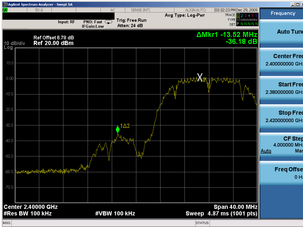
Plot 6-65. Band Edge Plot (802.11b – Ch. 1) – Chain A
