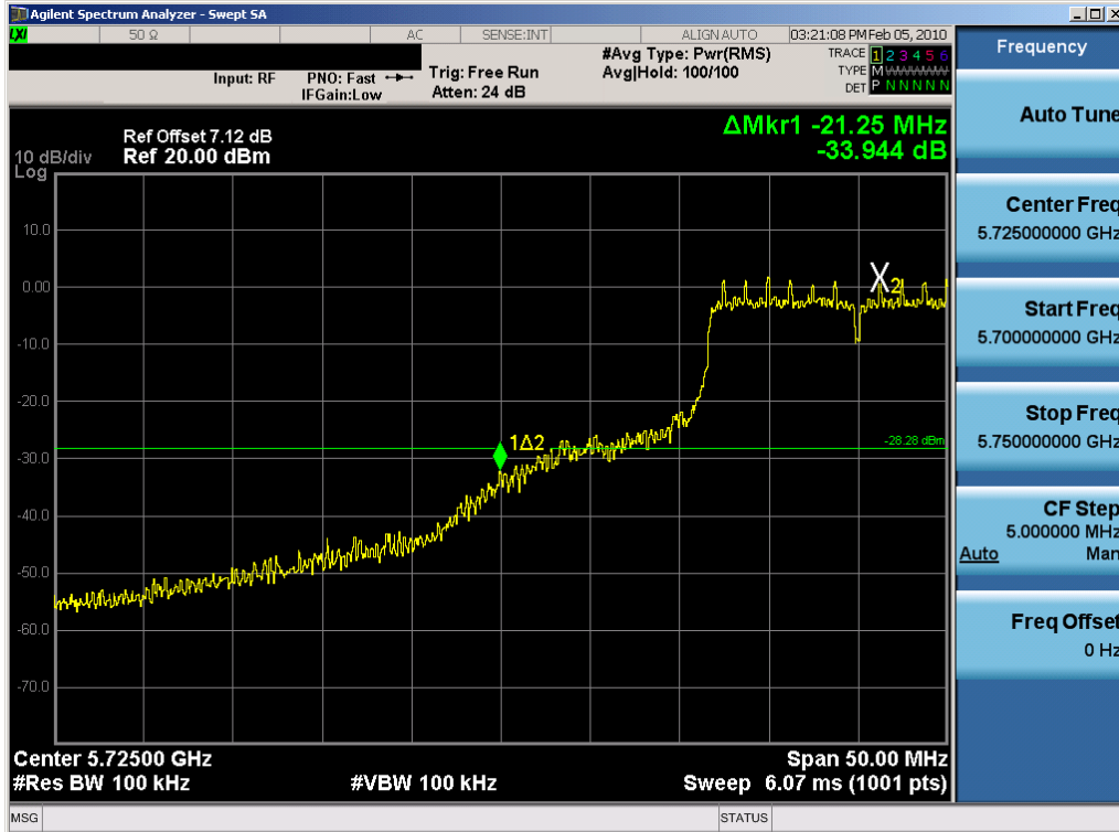
Plot 6-79. Band Edge Plot (802.11a – Ch. 149) – Chain B
