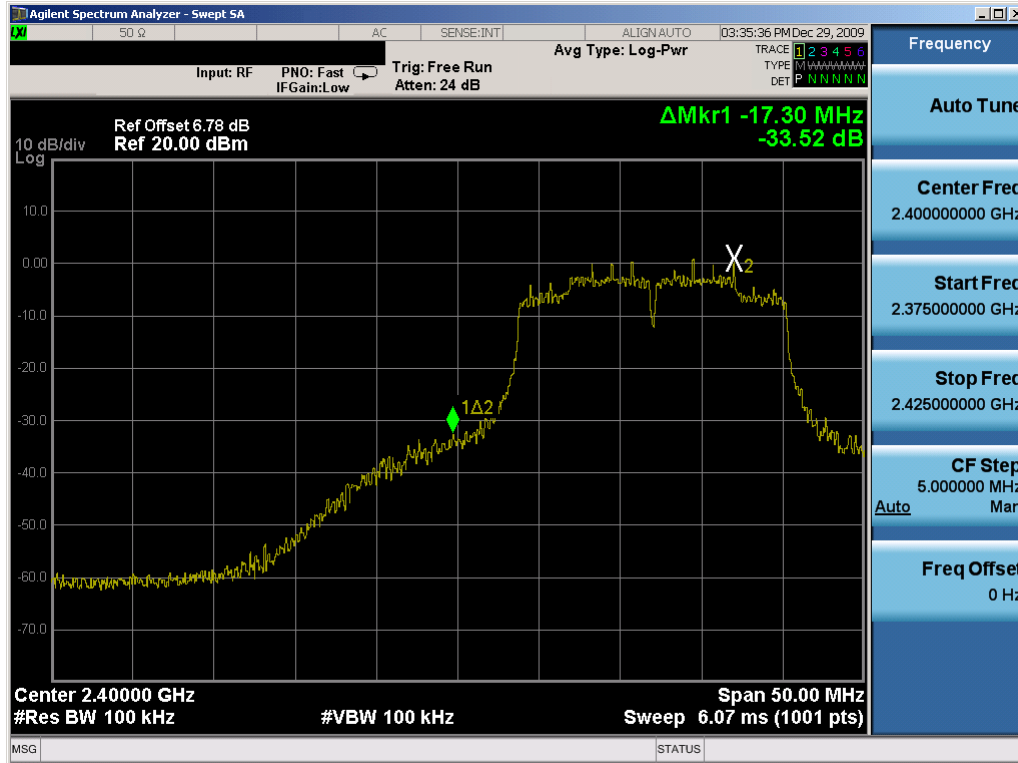
Plot 6-67. Band Edge Plot (802.11g- Ch. 1) – Chain A
