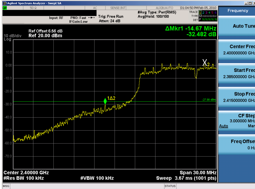
Plot 6-77. Band Edge Plot (802.11g – Ch. 1) – Chain B
