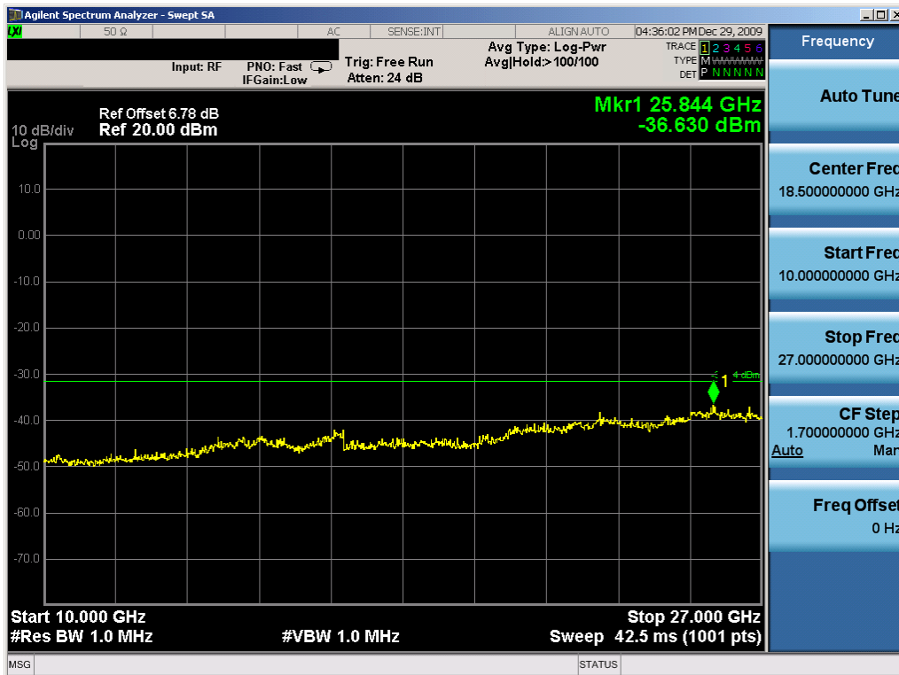
Plot 6-92. Conducted Spurious Plot (802.11a – Ch. 149) – Chain A
