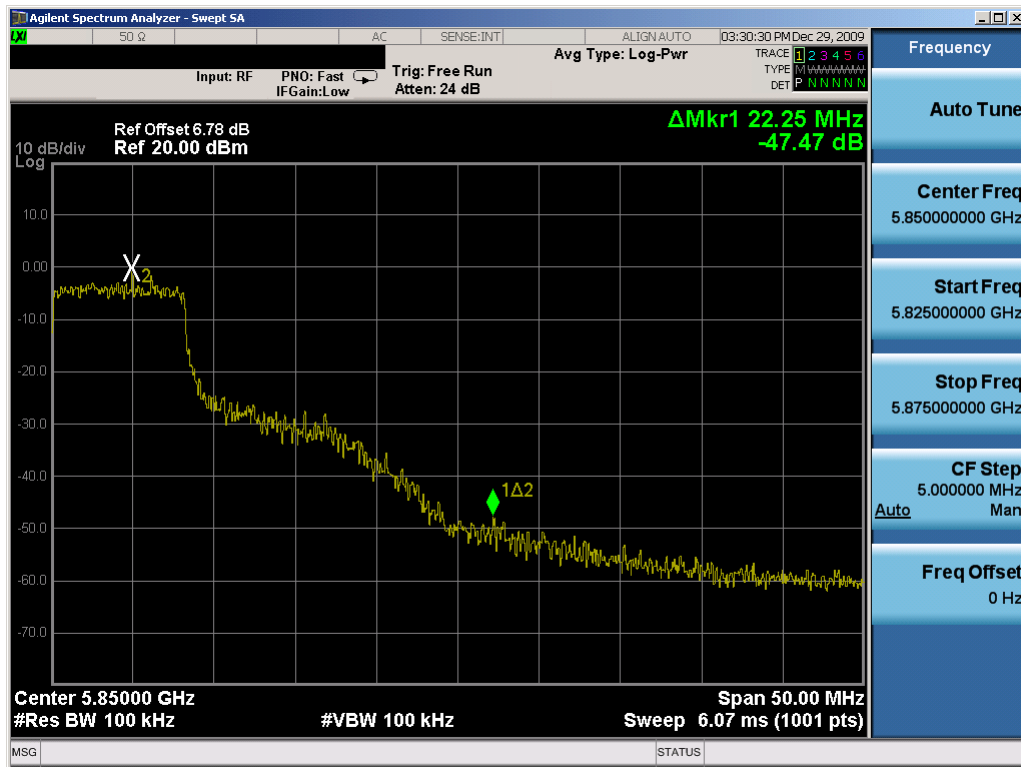
Plot 6-70. Band Edge Plot (802.11a – Ch. 165) – Chain A
