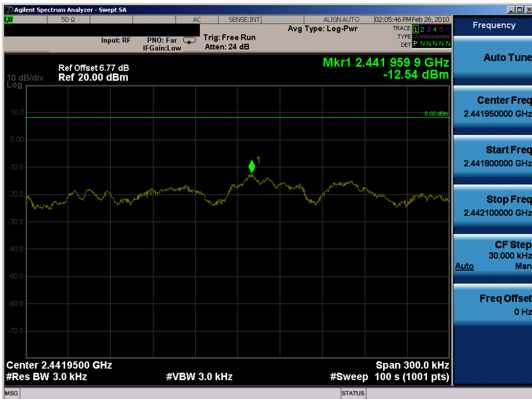
Plot 6-62. Power Spectral Density (802.11n (2.4GHz) Dual Transmit Mode – Ch. 6) – Chain B
