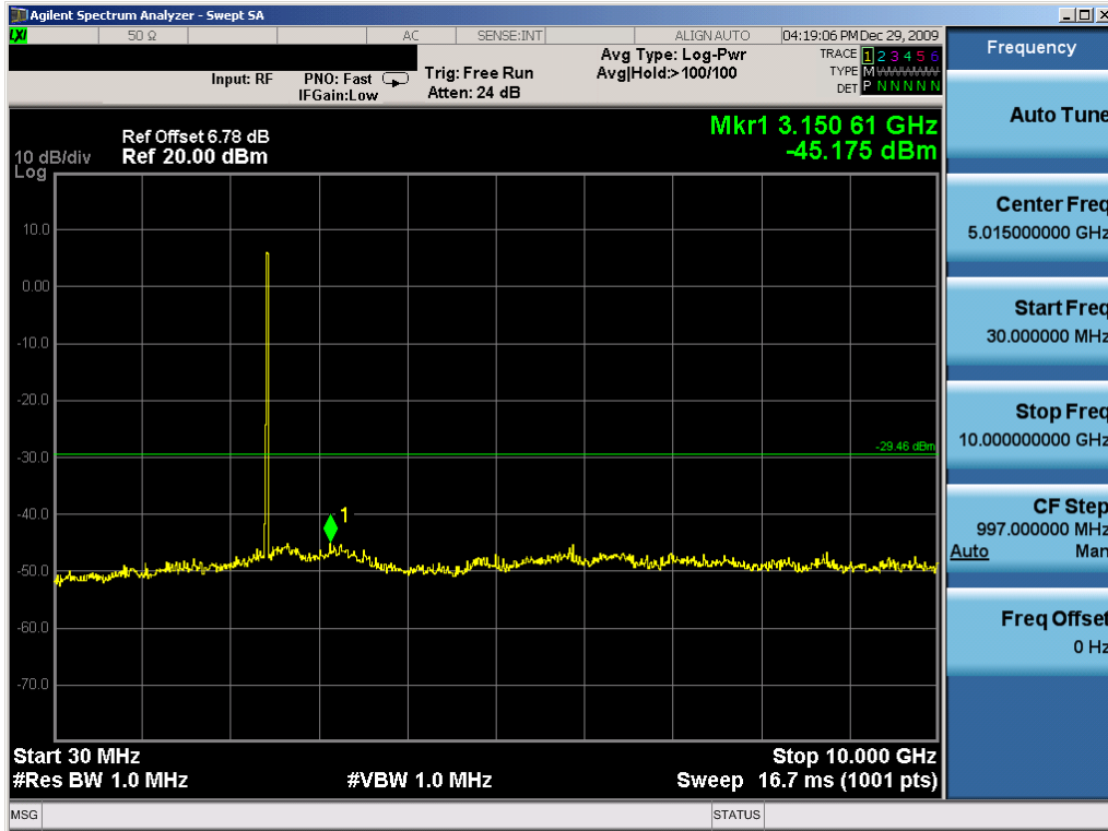
Plot 6-87. Conducted Spurious Plot (802.11b – Ch. 6) – Chain A
