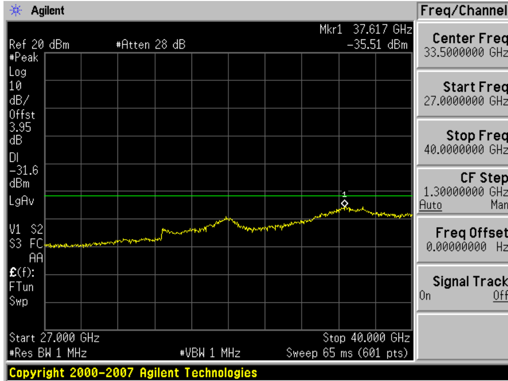
Plot 6-99. Conducted Spurious Plot (802.11a – Ch. 165) – Chain A
