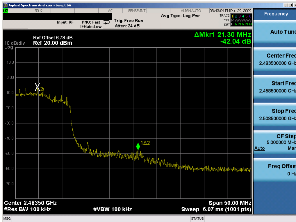
Plot 6-72. Band Edge Plot (802.11n (2.4GHz) – Ch. 9) – Chain A
