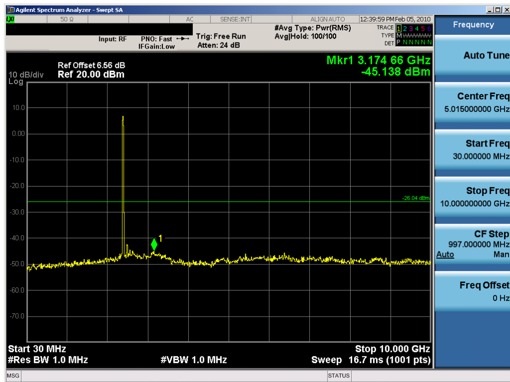
Plot 6-100. Conducted Spurious Plot (802.11b – Ch. 1) – Chain B
