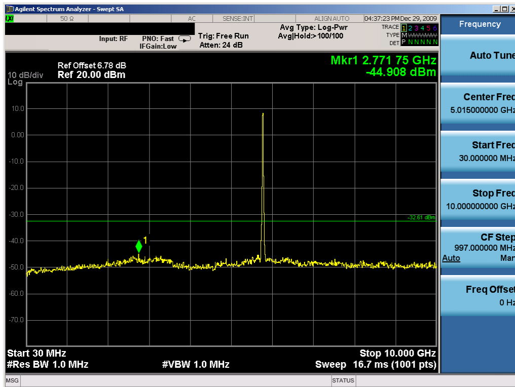
Plot 6-94. Conducted Spurious Plot (802.11a – Ch. 157) – Chain A
