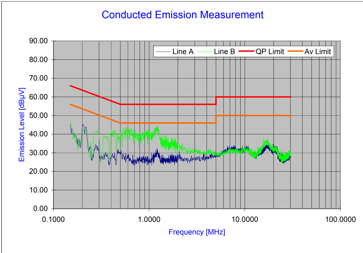
Plot 6-114. Line Conducted Plot with 802.11a
