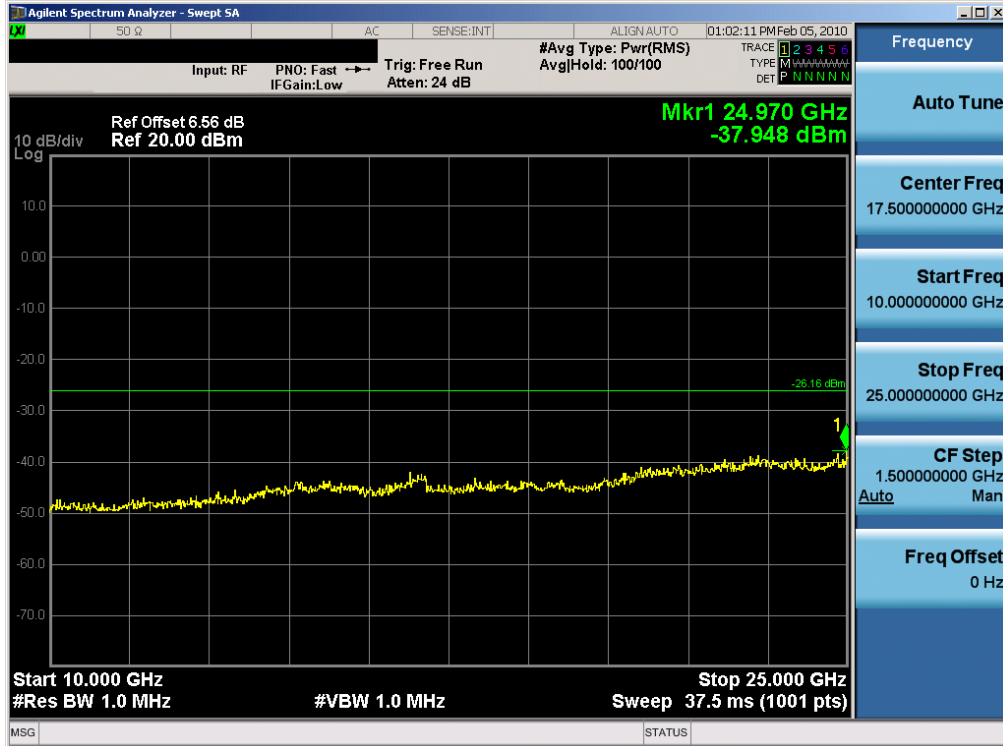
Plot 6-103. Conducted Spurious Plot (802.11b – Ch. 6) – Chain B
