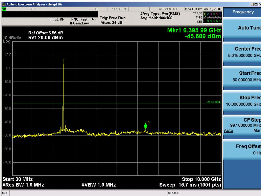
Plot 6-104. Conducted Spurious Plot (802.11b – Ch. 11) – Chain B
