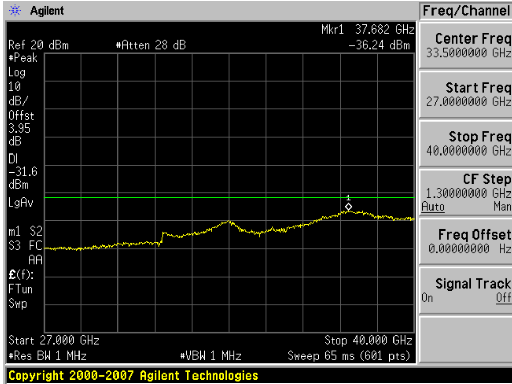
Plot 6-93. Conducted Spurious Plot (802.11a – Ch. 149) – Chain A
