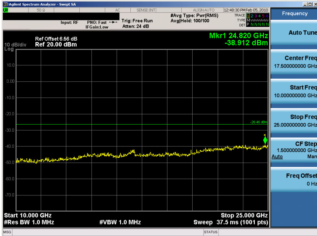
Plot 6-105. Conducted Spurious Plot (802.11b – Ch. 11) – Chain B
