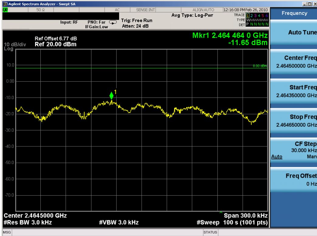
Plot 6-57. Power Spectral Density (802.11g Dual Transmit Mode – Ch. 11) – Chain A
