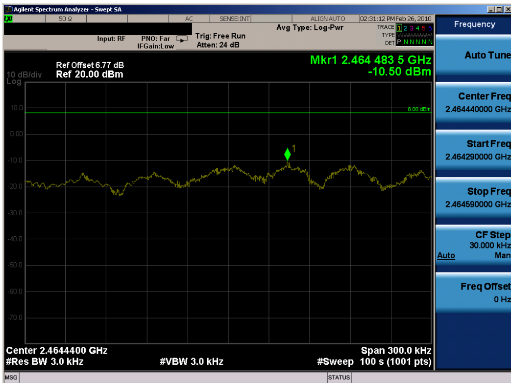
Plot 6-58. Power Spectral Density (802.11g Dual Transmit Mode – Ch. 11) – Chain B
