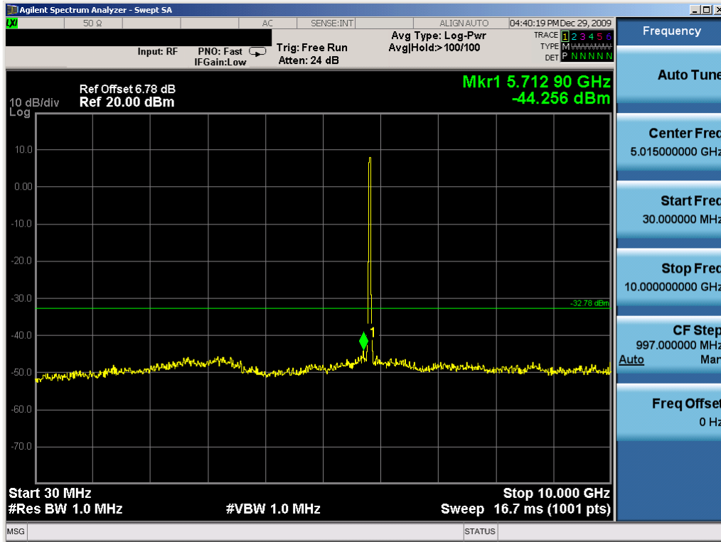
Plot 6-97. Conducted Spurious Plot (802.11a – Ch. 165) – Chain A
