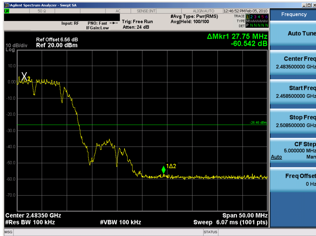
Plot 6-76. Band Edge Plot (802.11b – Ch. 11) – Chain B
