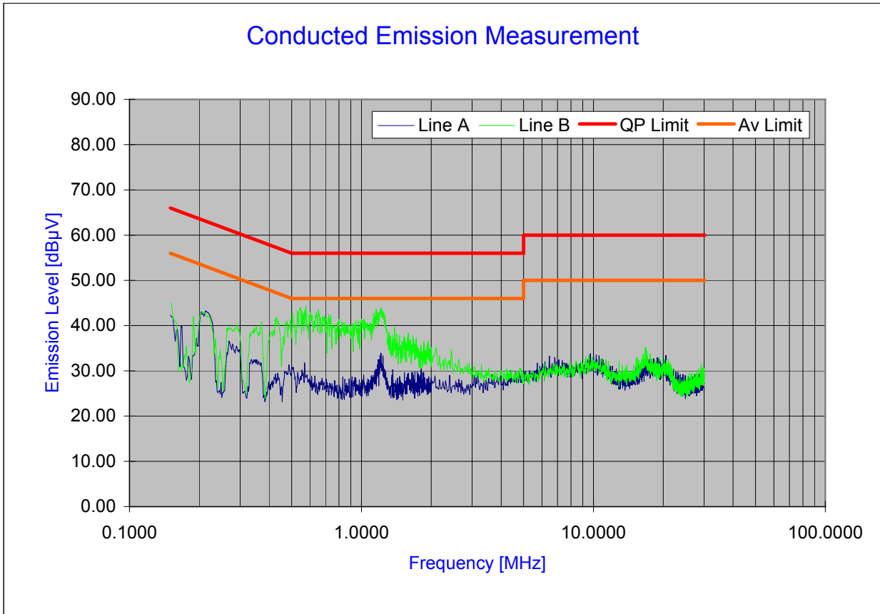
Plot 6-115. Line Conducted Plot with 802.11n
