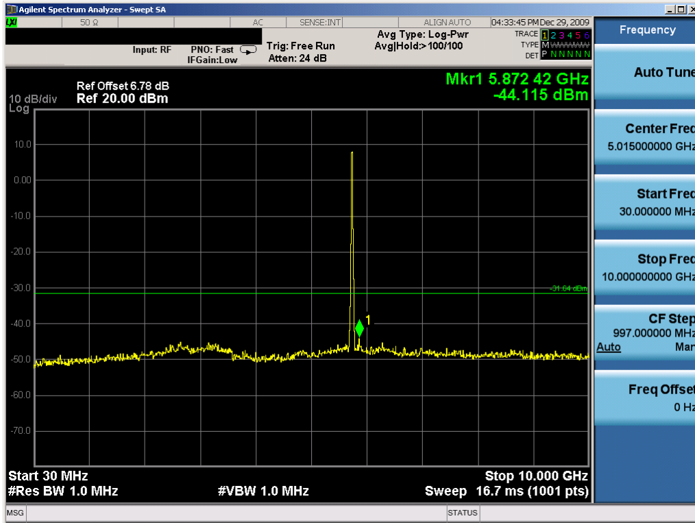
Plot 6-91. Conducted Spurious Plot (802.11a – Ch. 149) – Chain A
