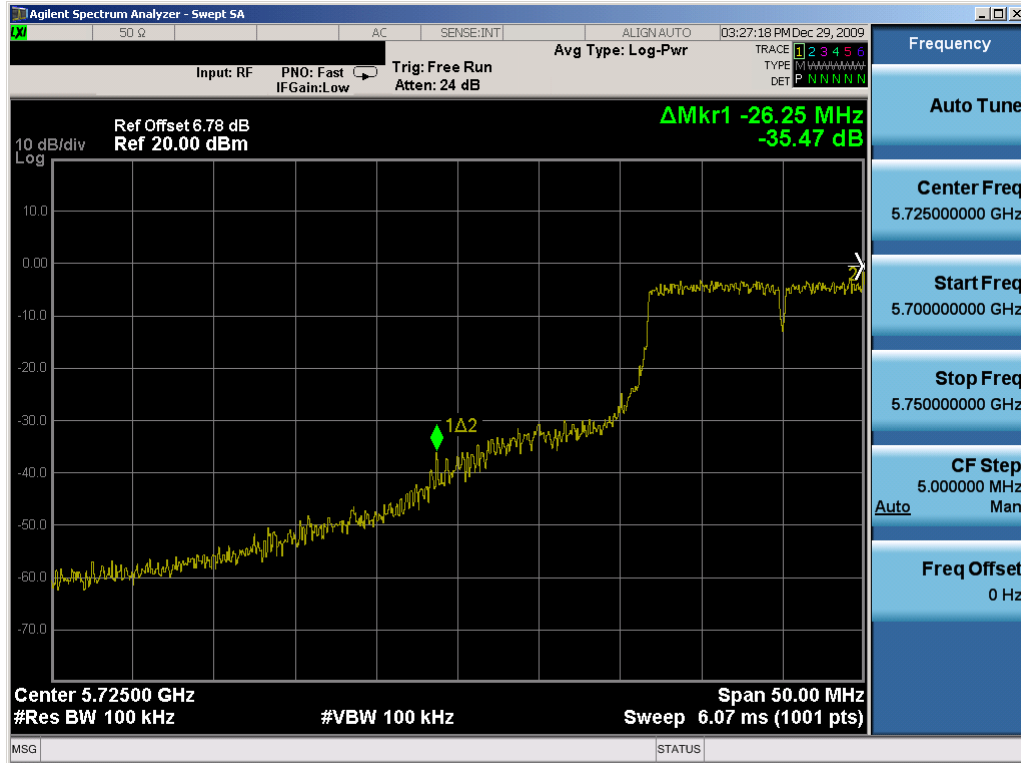
Plot 6-69. Band Edge Plot (802.11a – Ch. 149) – Chain A
