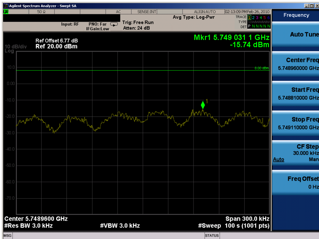
Plot 6-60. Power Spectral Density (802.11a Dual Transmit Mode – Ch. 149) – Chain B
