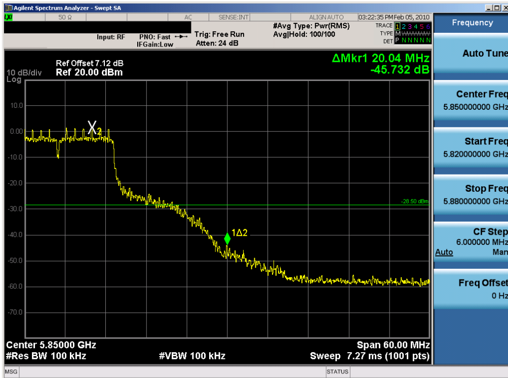
Plot 6-80. Band Edge Plot (802.11a – Ch. 165) – Chain B
