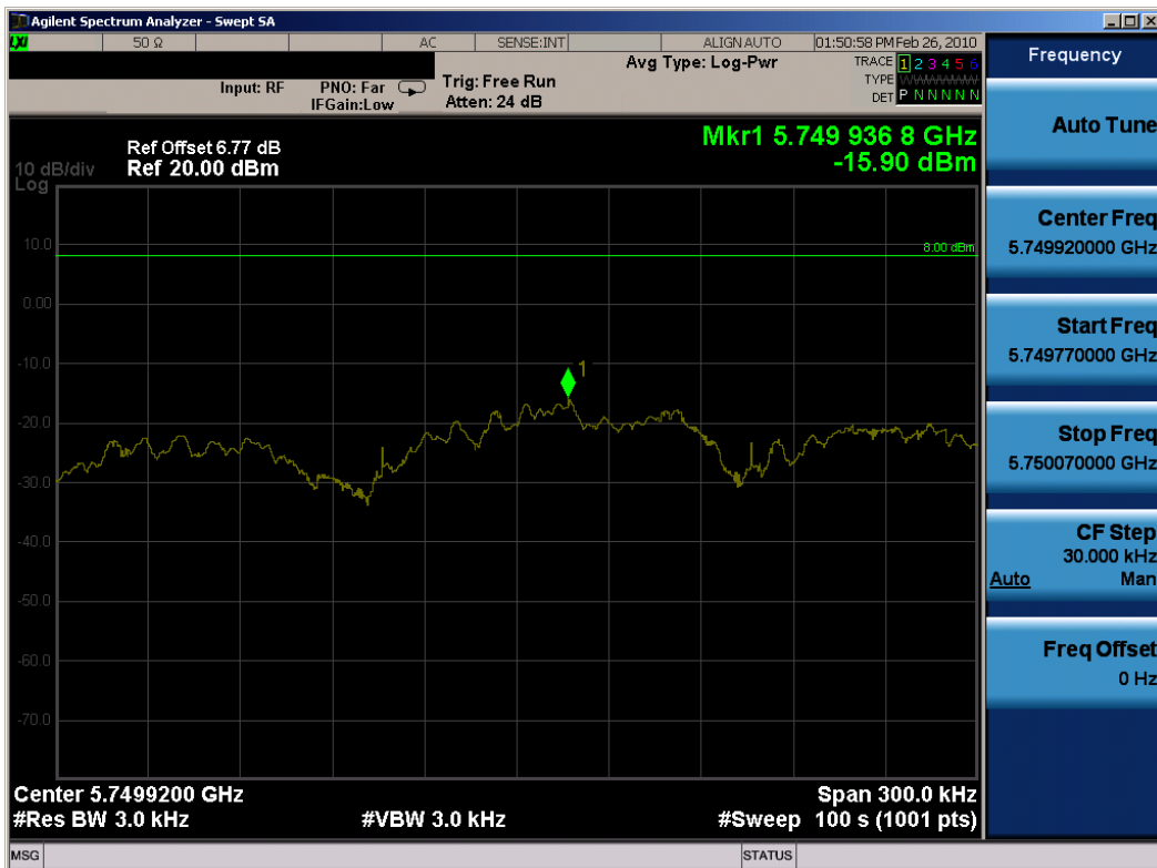
Plot 6-64. Power Spectral Density (802.11n (5.8GHz) Dual Transmit Mode – Ch. 151) – Chain B
