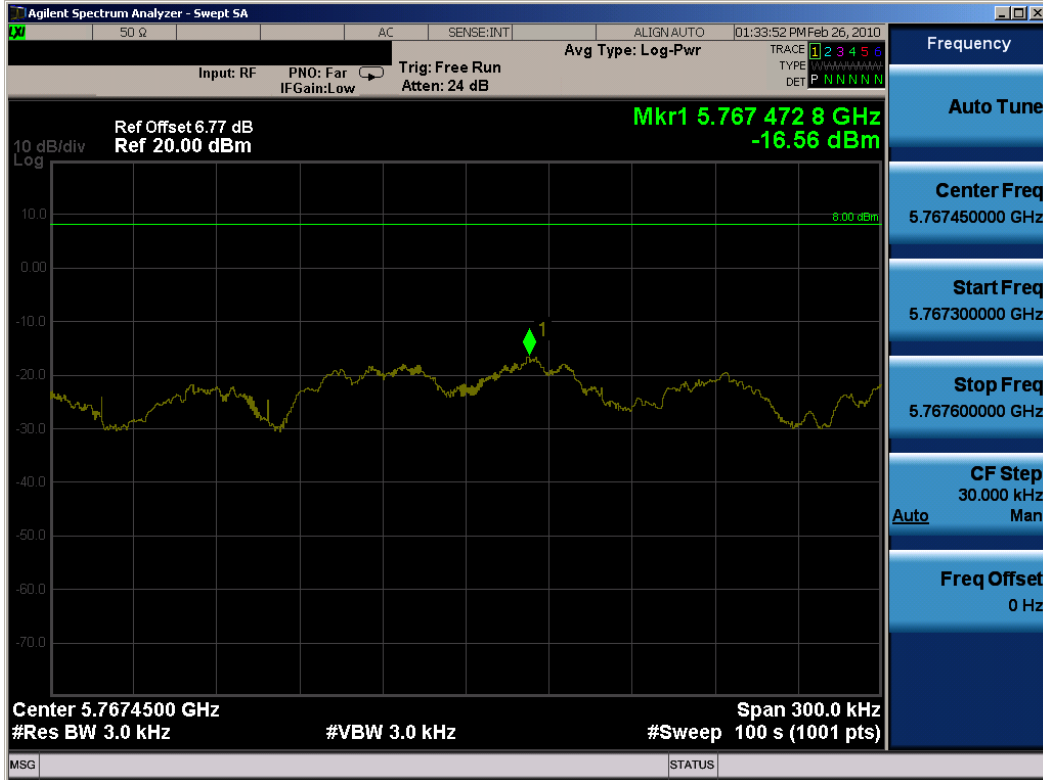
Plot 6-63. Power Spectral Density (802.11n (5.8GHz) Dual Transmit Mode – Ch. 151) – Chain A
