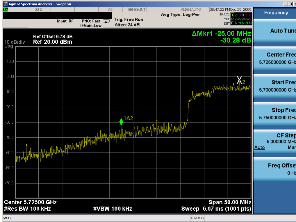
Plot 6-73. Band Edge Plot (802.11n (5.8GHz) – Ch. 151) – Chain A
