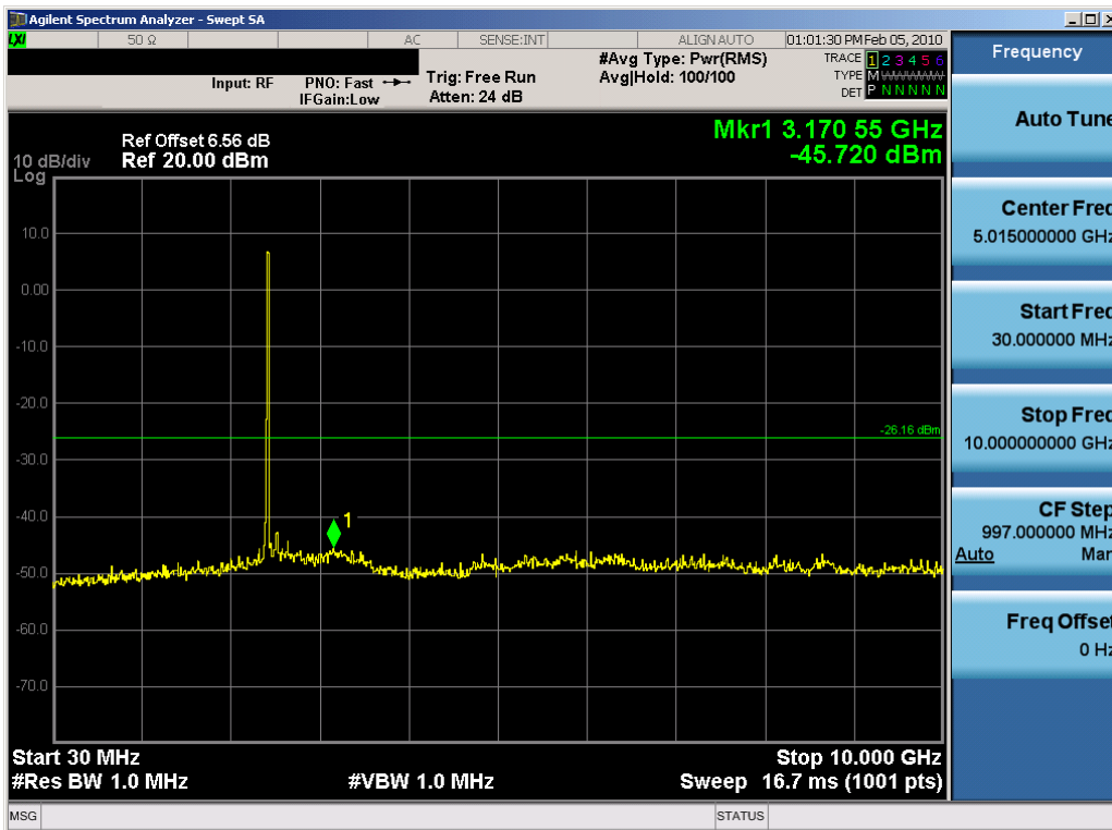
Plot 6-102. Conducted Spurious Plot (802.11b – Ch. 6) – Chain B
