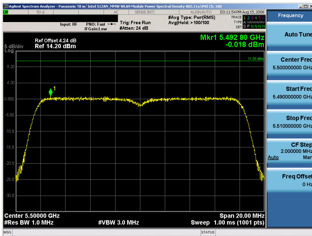
Plot 6-23. Peak Power Spectral Density Plot (802.11a (UNII) – Ch. 100)
