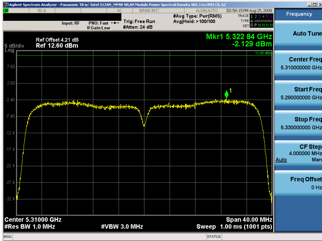
Plot 6-29. Peak Power Spectral Density Plot (802.11n (UNII) – Ch. 62)
