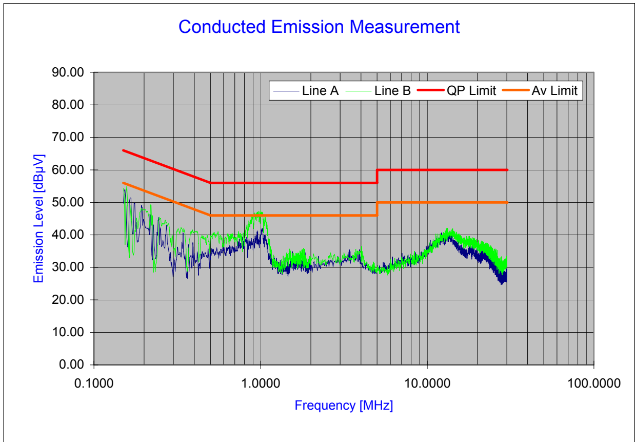
Plot 6-53. Line Conducted Plot with 802.11n (UNII Band II)
