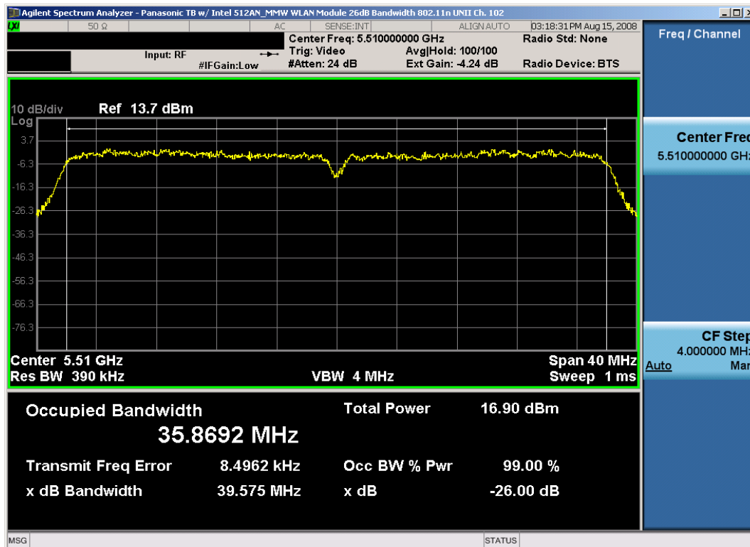
Plot 6-14. 26dB Bandwidth Plot (802.11n (UNII) – Ch. 102)
