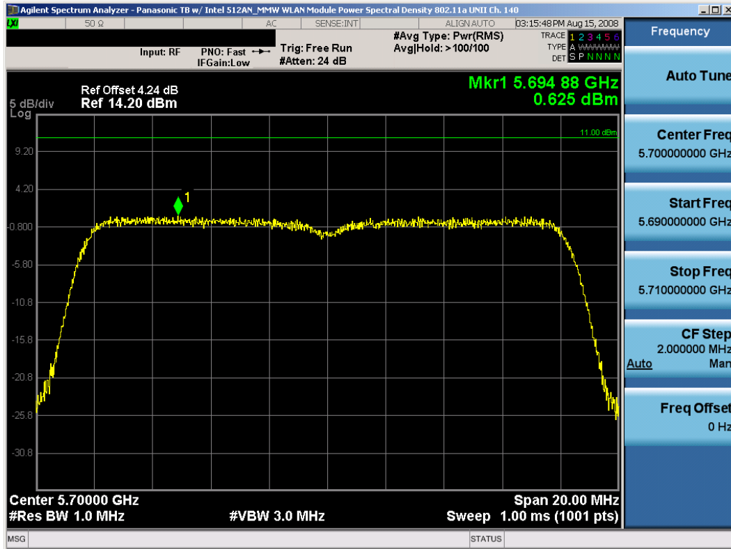
Plot 6-25. Peak Power Spectral Density Plot (802.11a (UNII) – Ch. 140)
