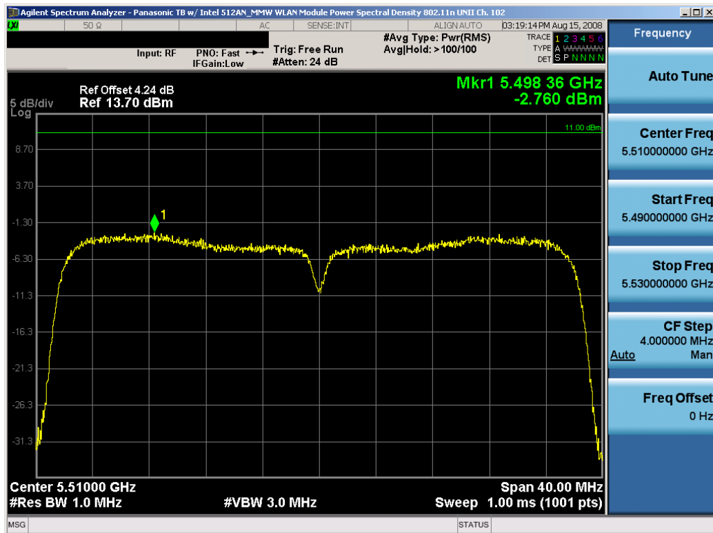
Plot 6-30. Peak Power Spectral Density Plot (802.11n (UNII) – Ch. 102)
