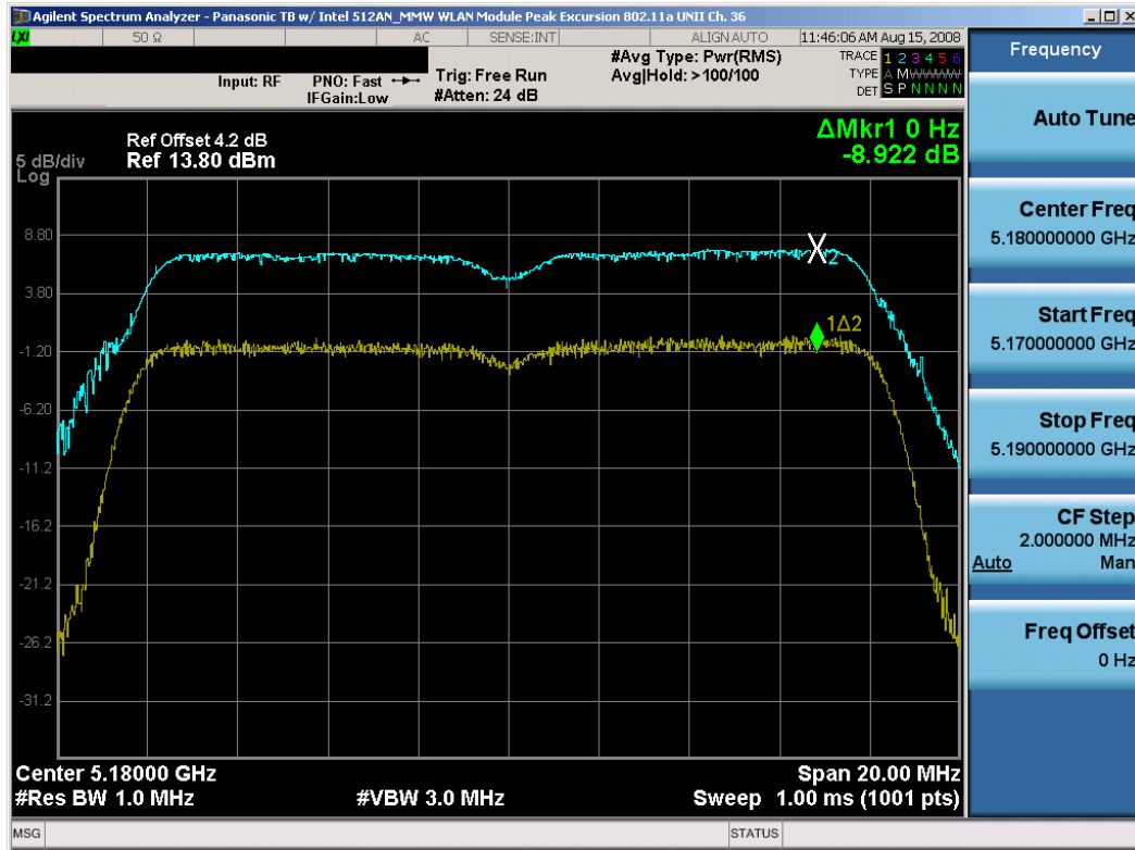
Plot 6-33. Peak Excursion Ratio Plot (802.11a (UNII) – Ch. 36)
