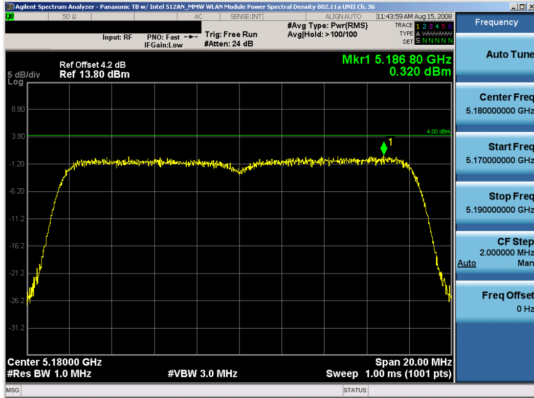
Plot 6-17. Peak Power Spectral Density Plot (802.11a (UNII) – Ch. 36)
