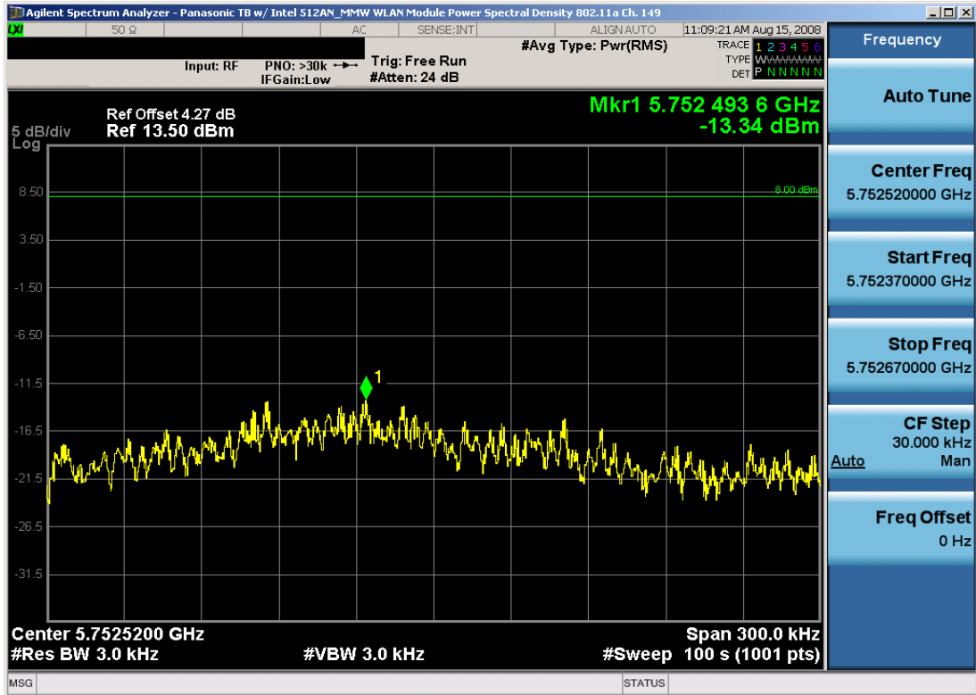
Plot 6-21. Power Spectral Density Plot (802.11a – Ch. 149)
