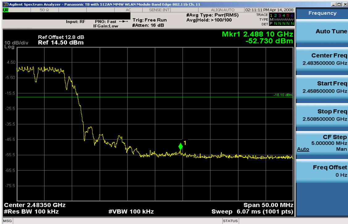
Plot 6-30. Band Edge Plot (802.11b – Ch. 11)
