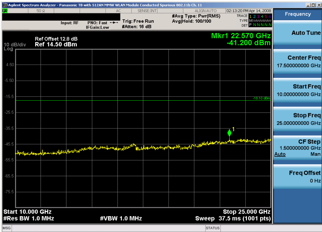
Plot 6-44. Conducted Spurious Plot (802.11b – Ch. 11)
