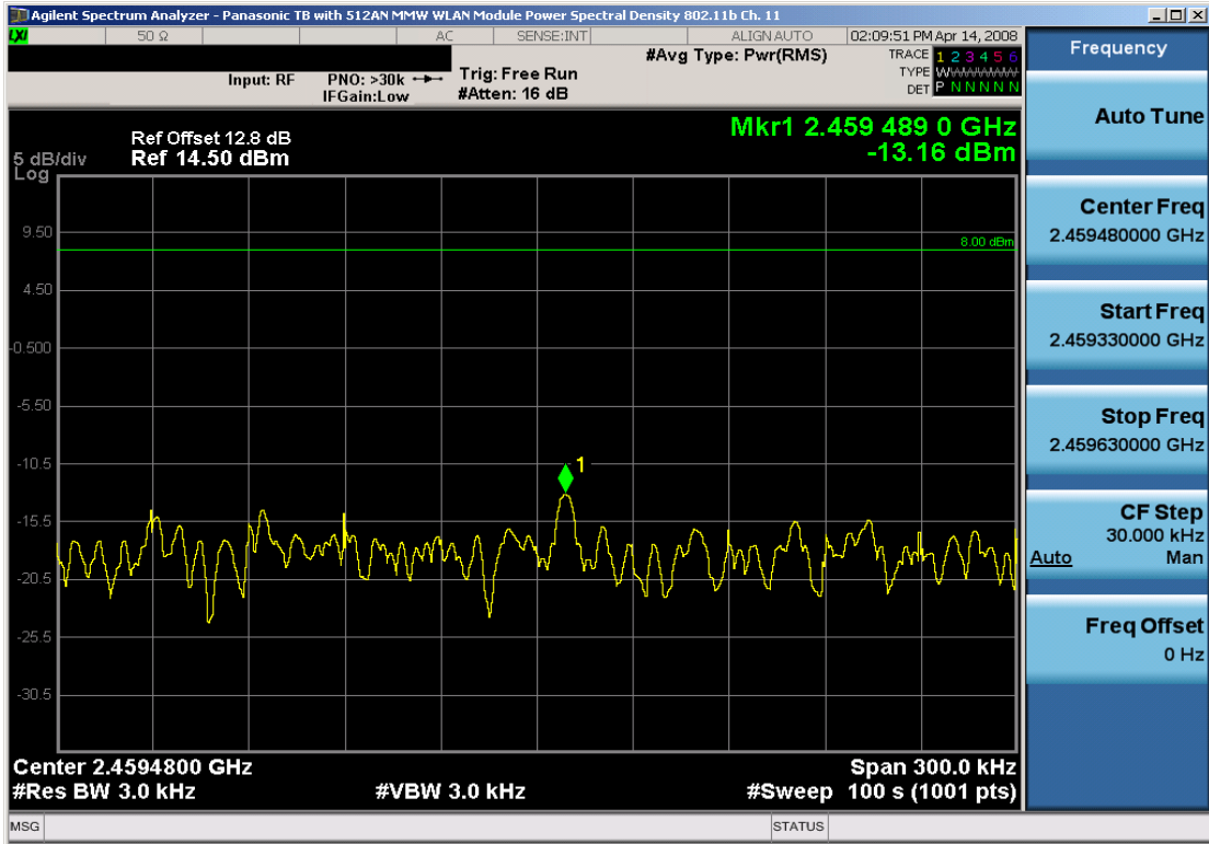
Plot 6-17. Power Spectral Density Plot (802.11b – Ch. 11)
