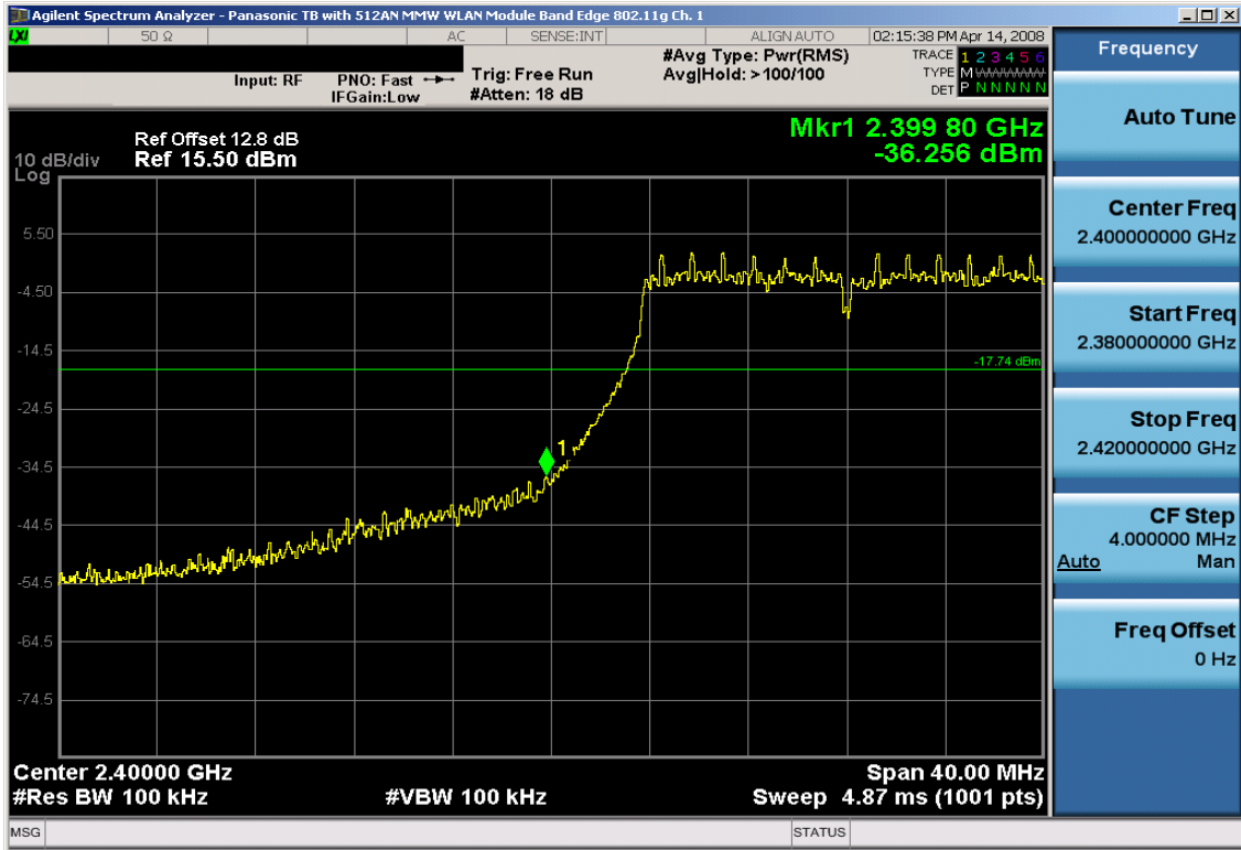
Plot 6-31. Band Edge Plot (802.11g– Ch. 1)
