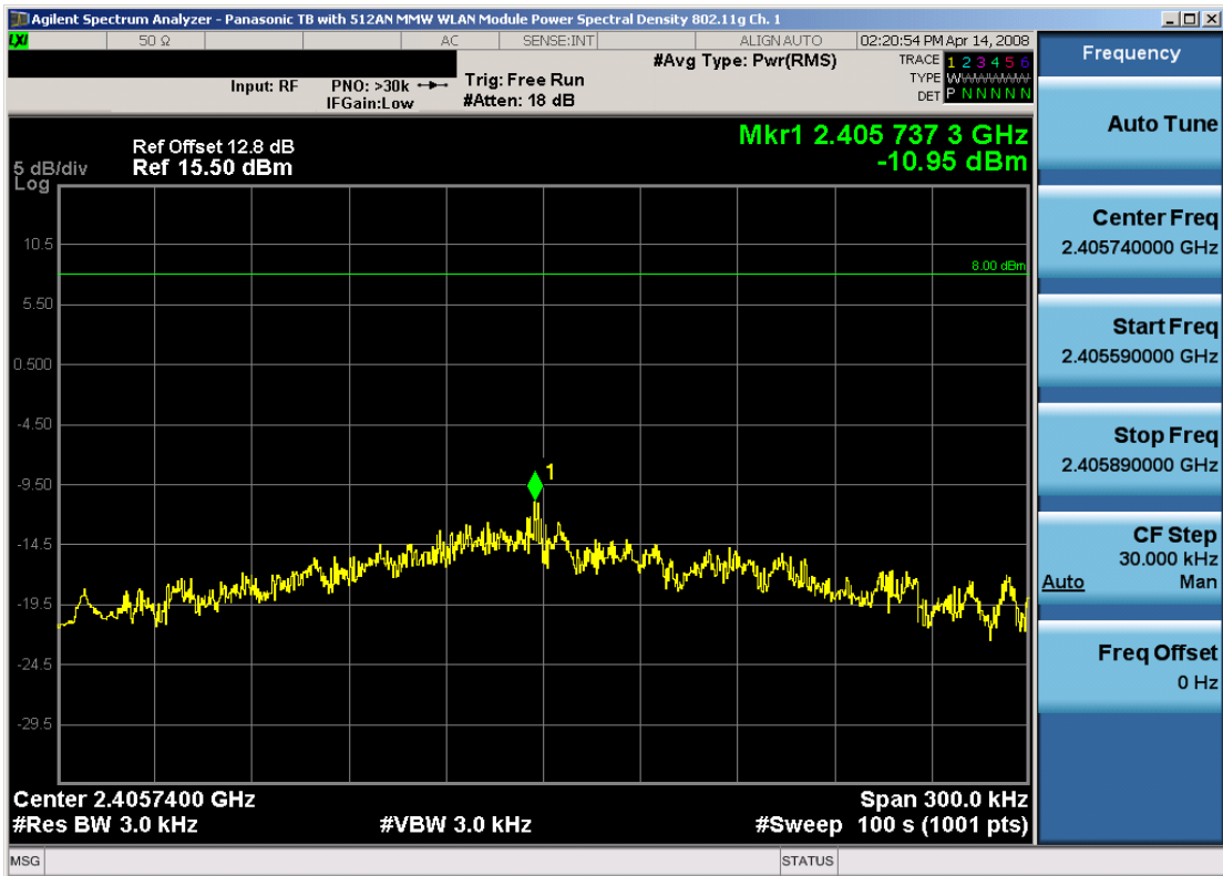
Plot 6-18. Power Spectral Density Plot (802.11g – Ch. 1)
