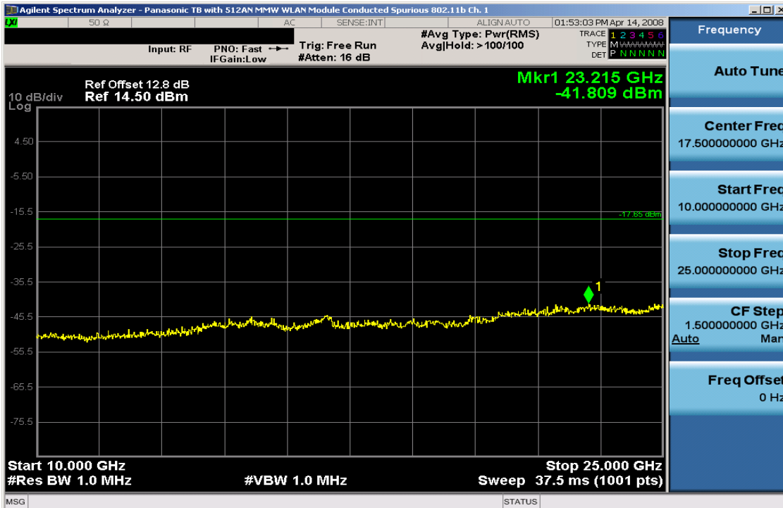
Plot 6-40. Conducted Spurious Plot (802.11b – Ch. 1)
