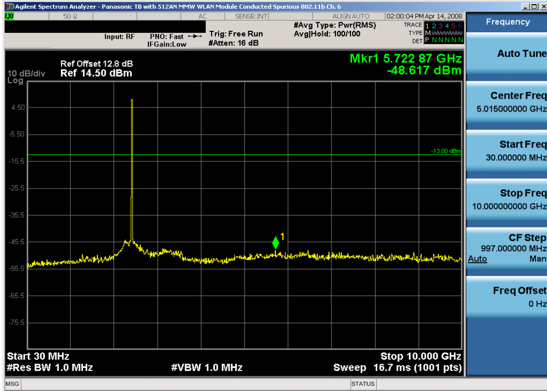
Plot 6-41. Conducted Spurious Plot (802.11b – Ch. 6)
