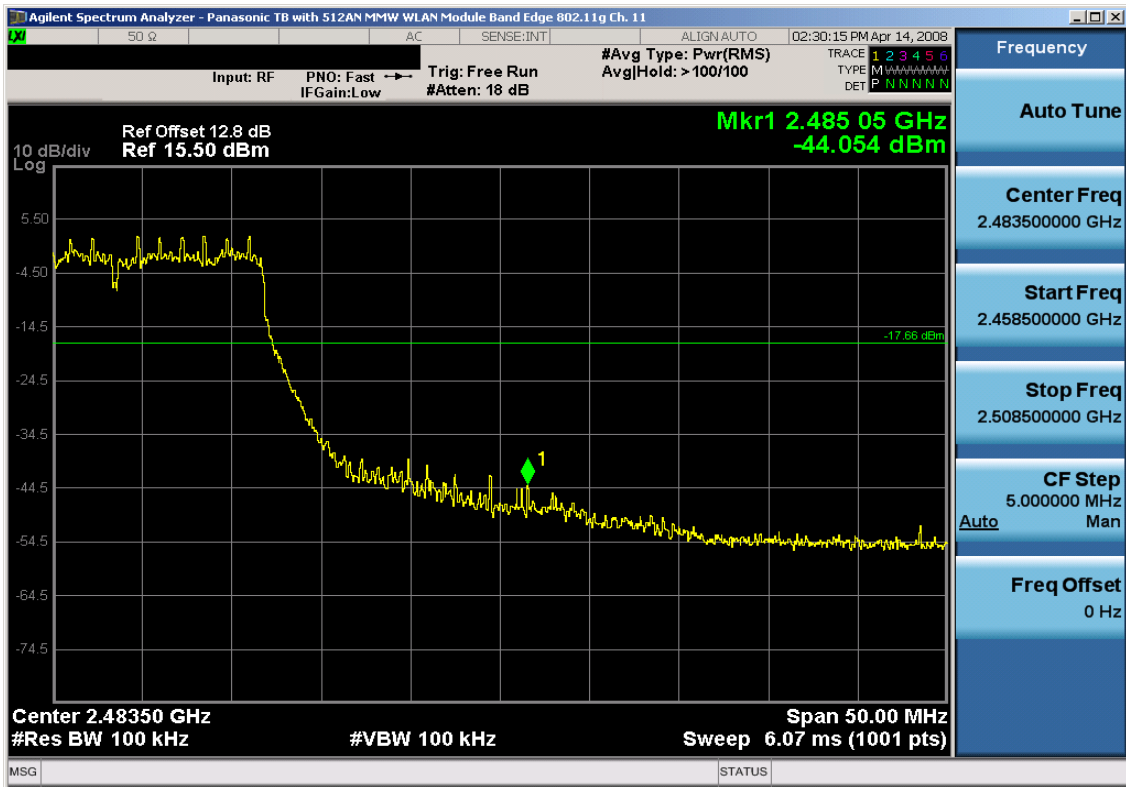
Plot 6-32. Band Edge Plot (802.11g – Ch. 11)
