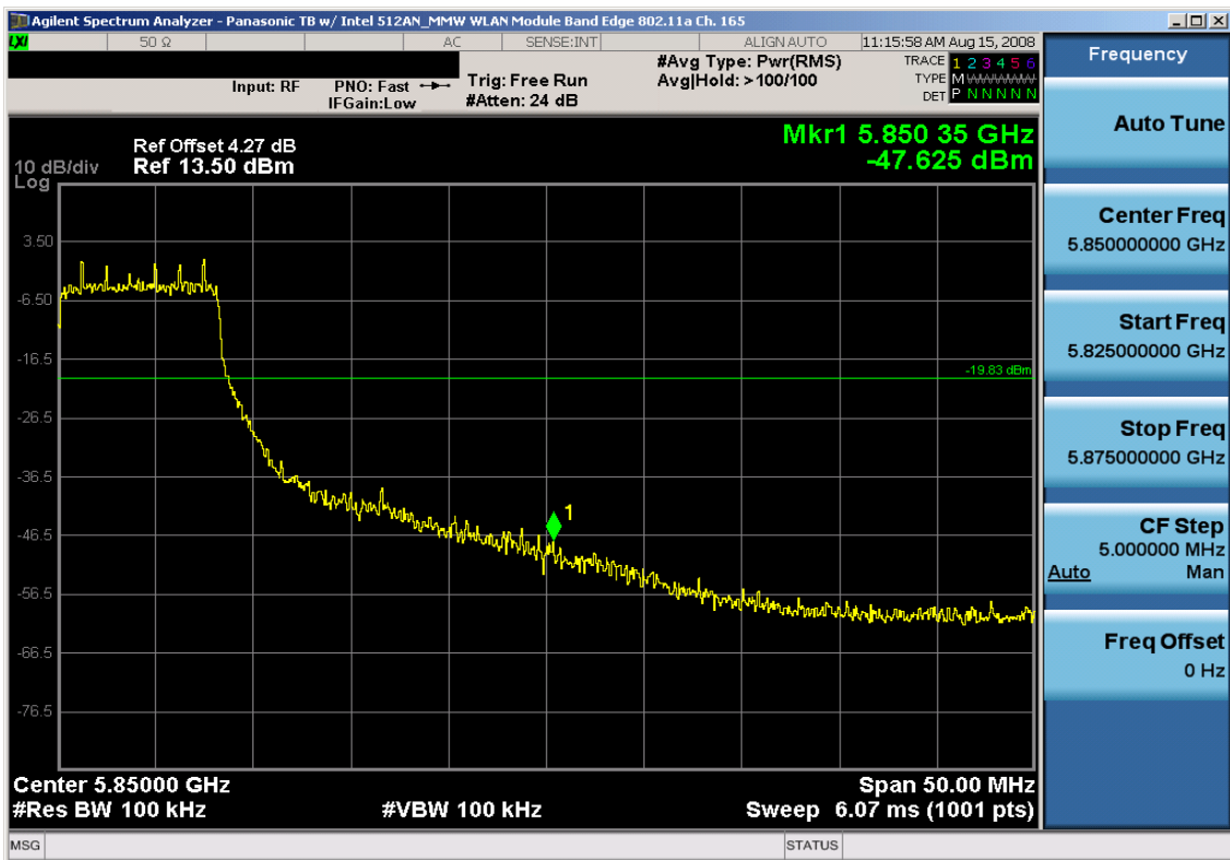
Plot 6-34. Band Edge Plot (802.11a – Ch. 165)
