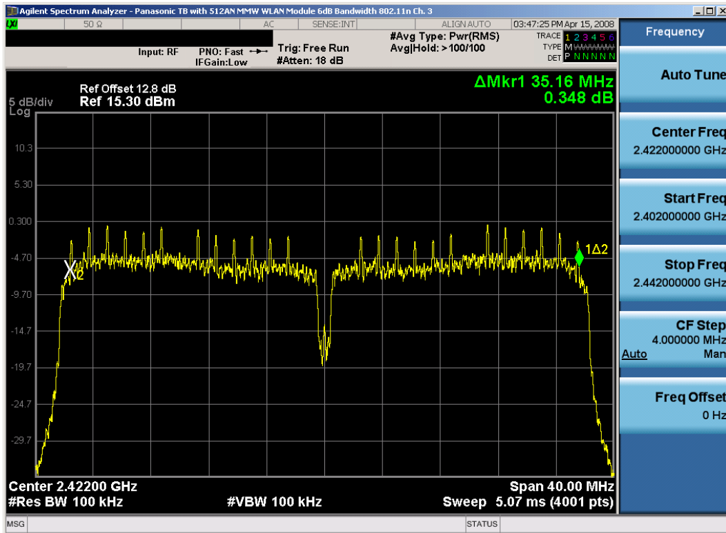
Plot 6-10. 6dB Bandwidth Plot (802.11n (2.4GHz) – Ch. 3)
