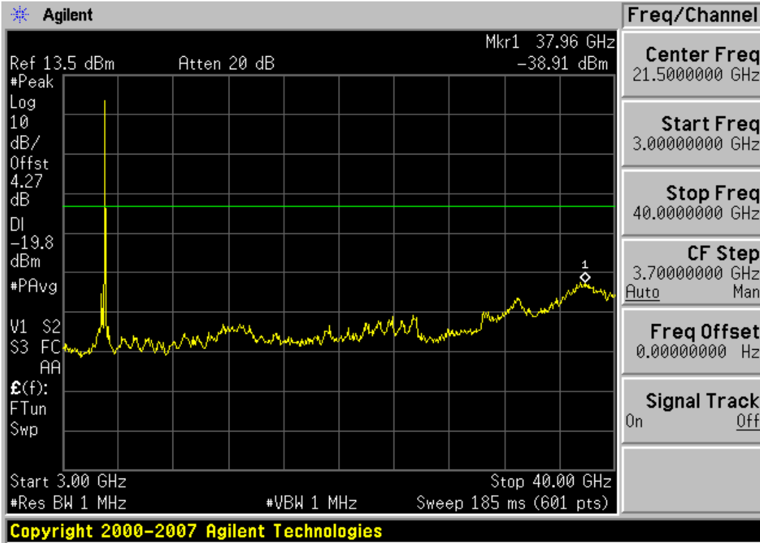
Plot 6-49. Conducted Spurious Plot (802.11a – Ch. 165)
