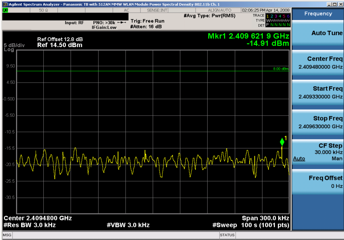
Plot 6-15. Power Spectral Density Plot (802.11b – Ch. 1)
