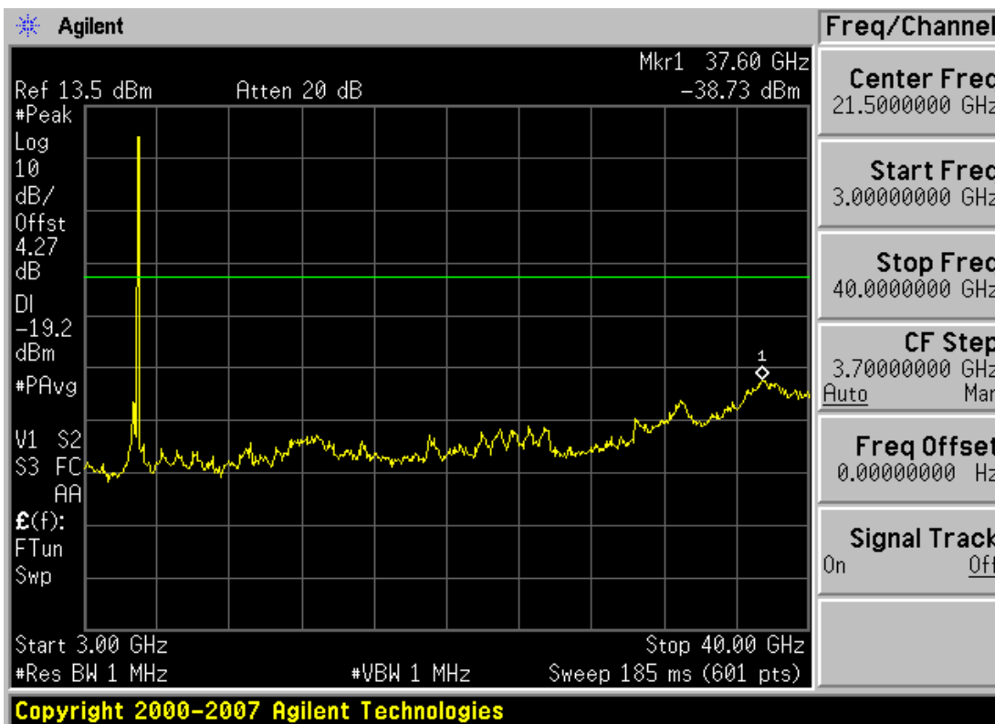
Plot 6-45. Conducted Spurious Plot (802.11a – Ch. 149)
