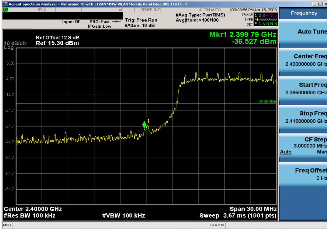
Plot 6-35. Band Edge Plot (802.11n (2.4GHz) – Ch. 3)
