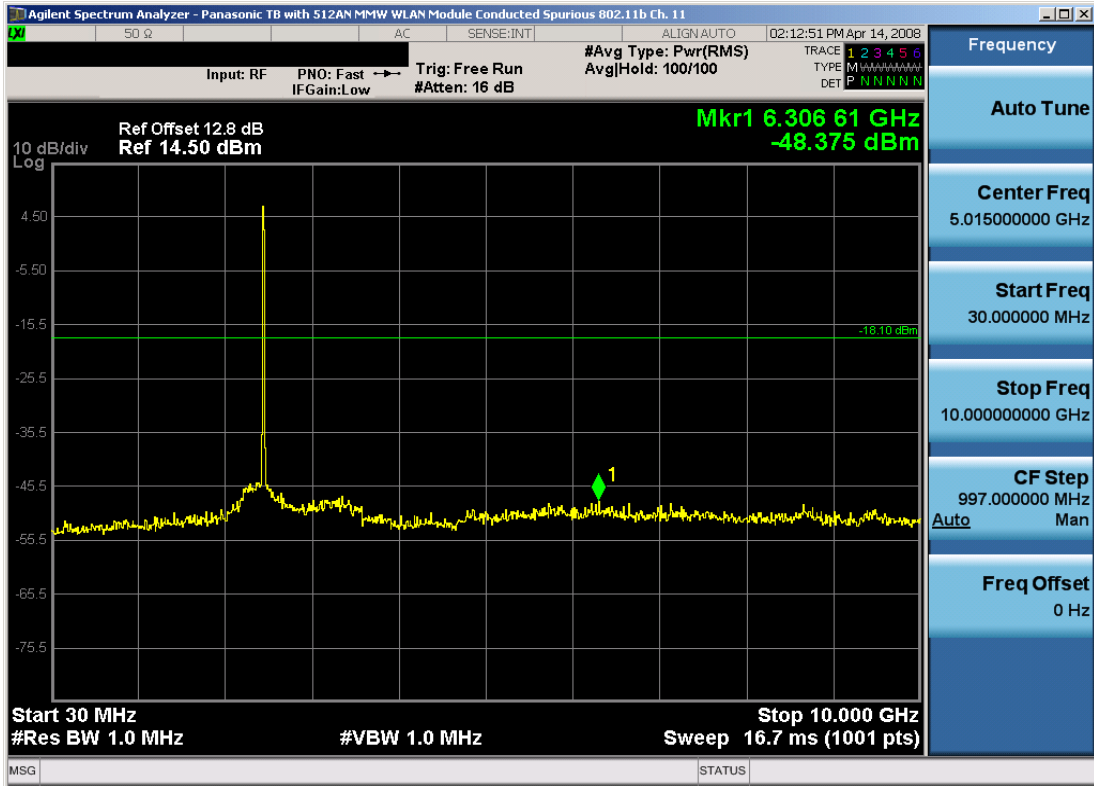
Plot 6-43. Conducted Spurious Plot (802.11b – Ch. 11)
