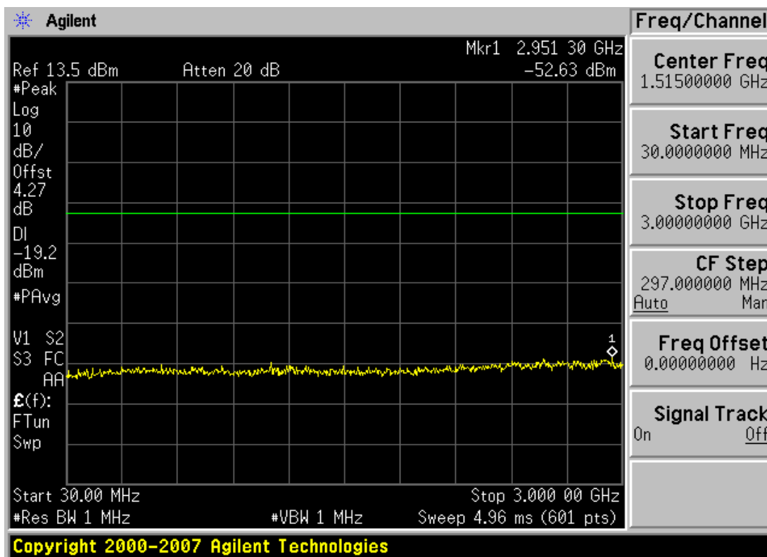
Plot 6-46. Conducted Spurious Plot (802.11a – Ch. 149)
