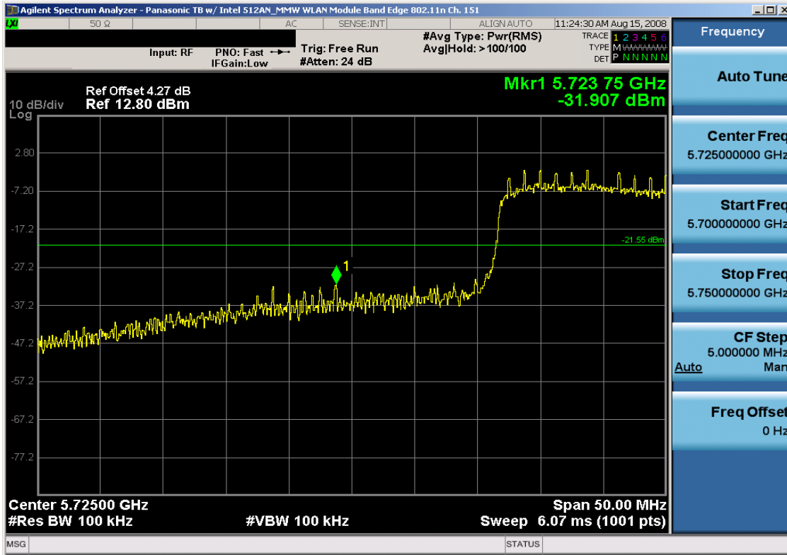
Plot 6-37. Band Edge Plot (802.11n (5.8GHz) – Ch. 151)
