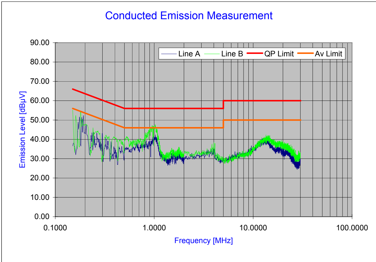
Plot 6-53. Line Conducted Plot with 802.11g
