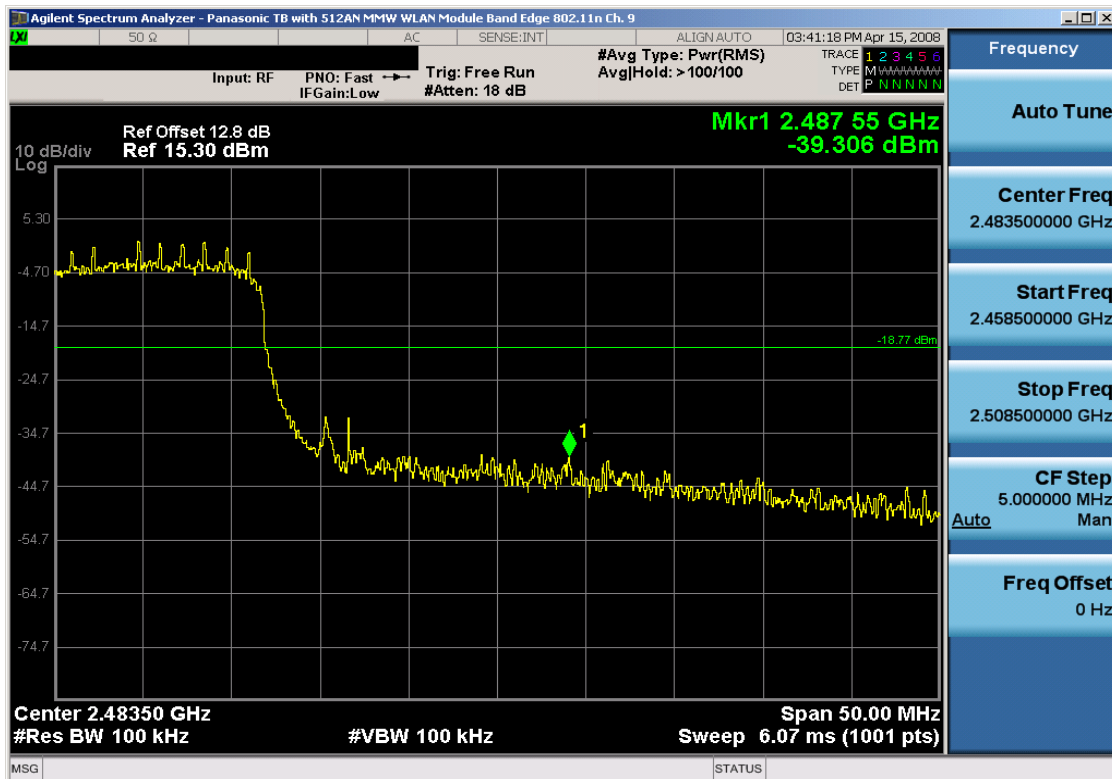
Plot 6-36. Band Edge Plot (802.11n (2.4GHz) – Ch. 9)
