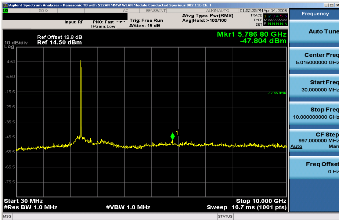
Plot 6-39. Conducted Spurious Plot (802.11b – Ch. 1)
