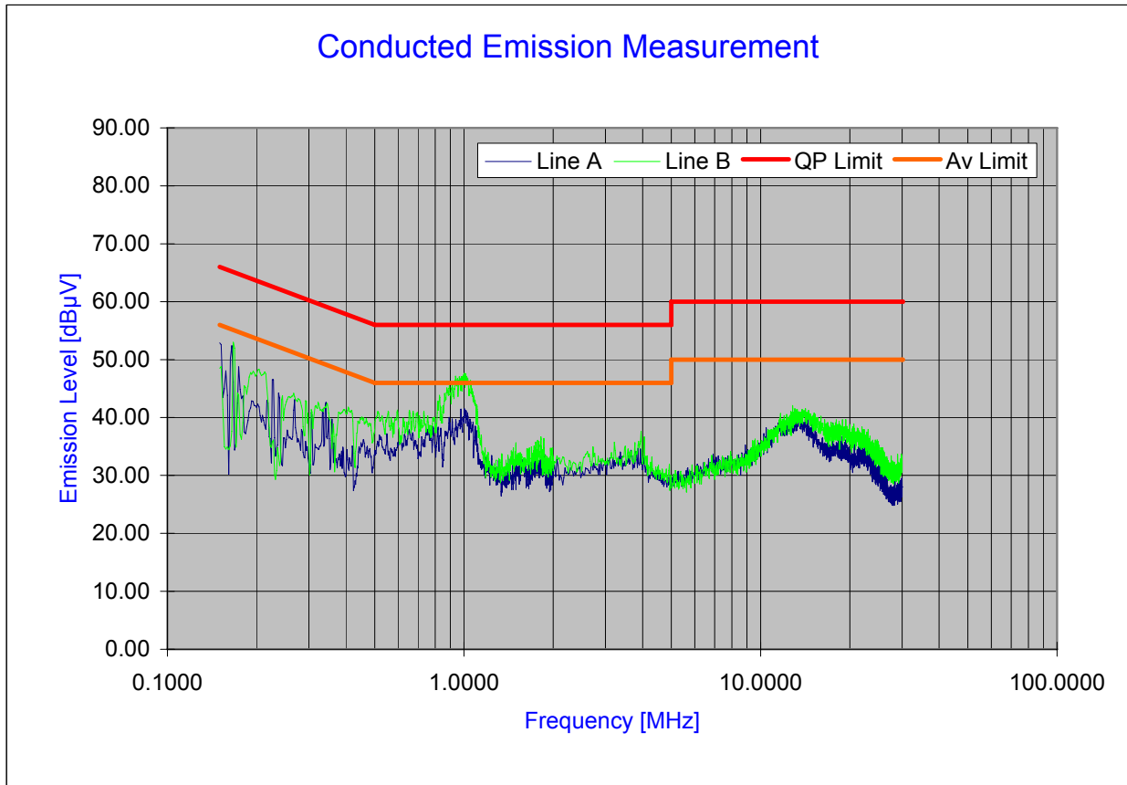
Plot 6-52. Line Conducted Plot with 802.11b
