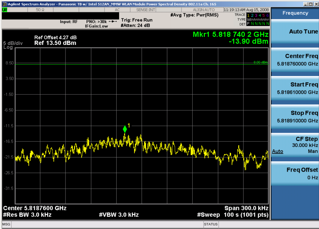
Plot 6-23. Power Spectral Density Plot (802.11a – Ch. 165)
