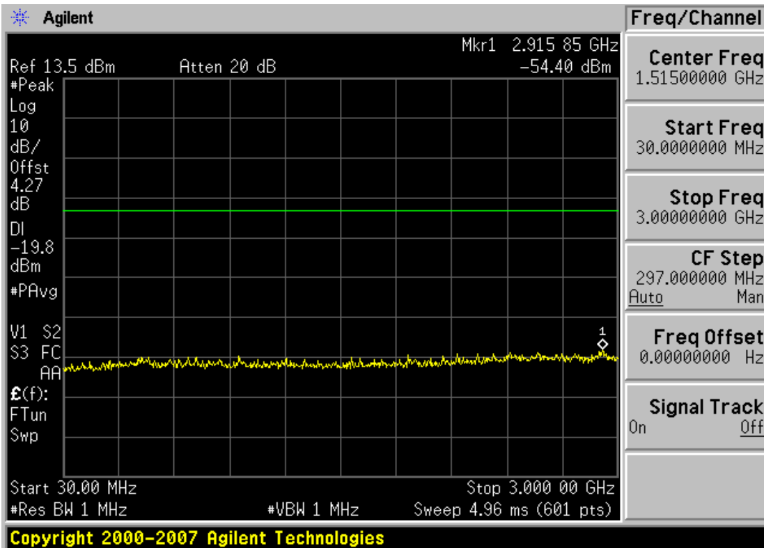
Plot 6-50. Conducted Spurious Plot (802.11a – Ch. 165)
