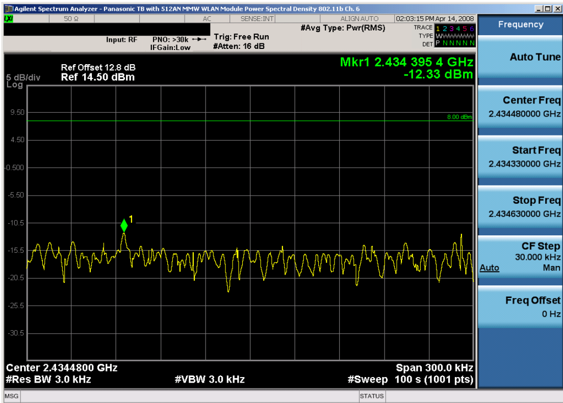
Plot 6-16. Power Spectral Density Plot (802.11b – Ch. 6)
