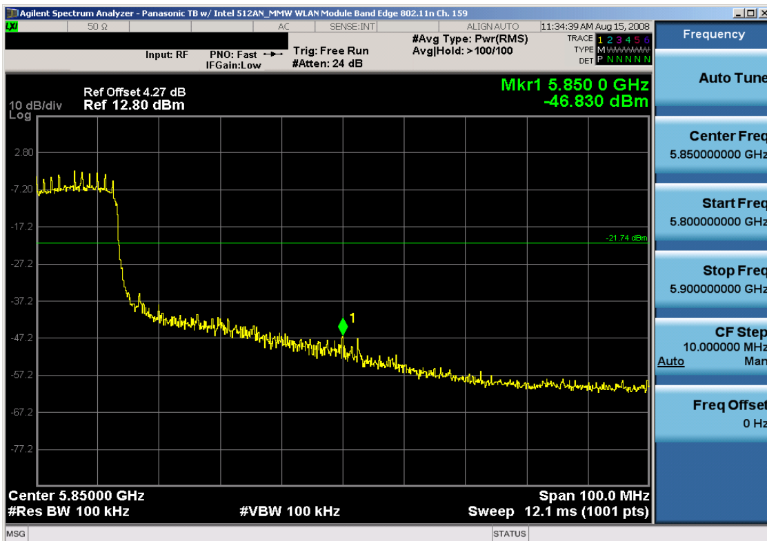
Plot 6-38. Band Edge Plot (802.11n (5.8GHz) – Ch. 159)
