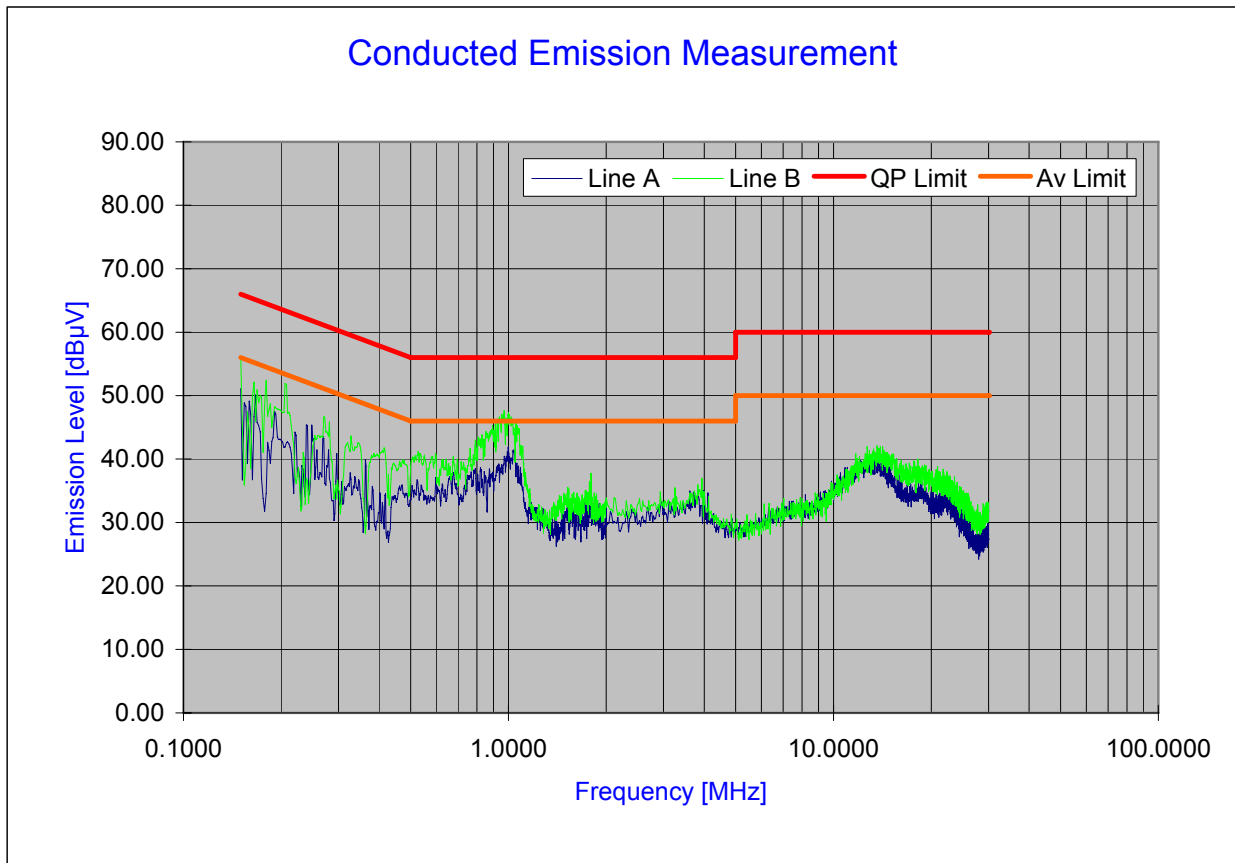
Plot 6-51. Line Conducted Plot with 802.11a
