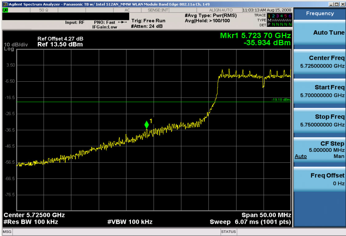
Plot 6-33. Band Edge Plot (802.11a – Ch. 149)
