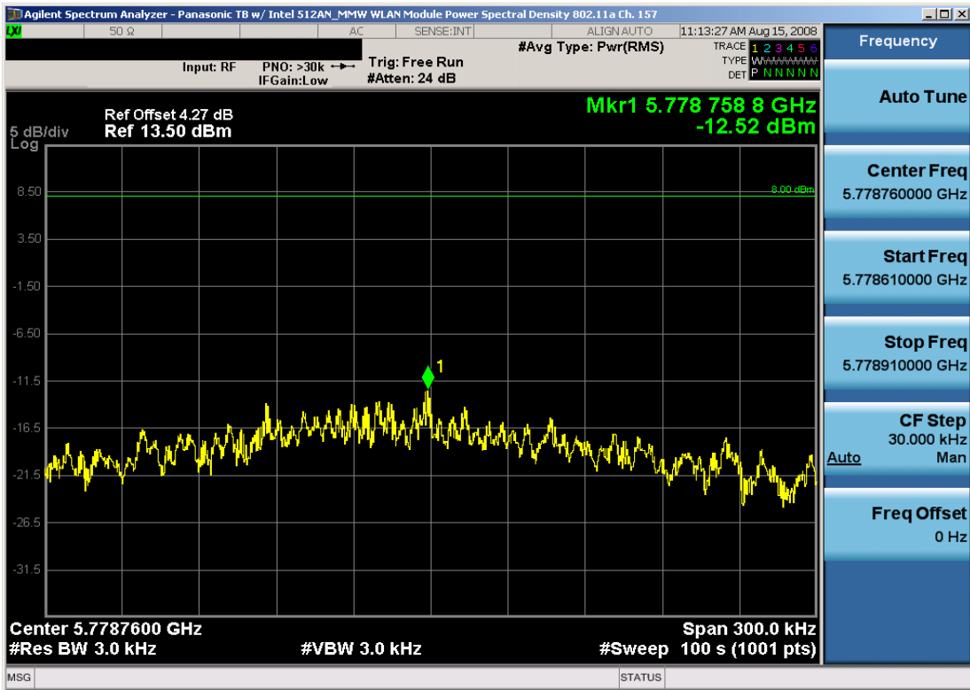
Plot 6-22. Power Spectral Density Plot (802.11a – Ch. 157)
