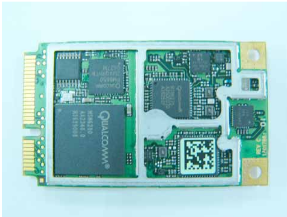
WWAN Module Interior Bottom View
