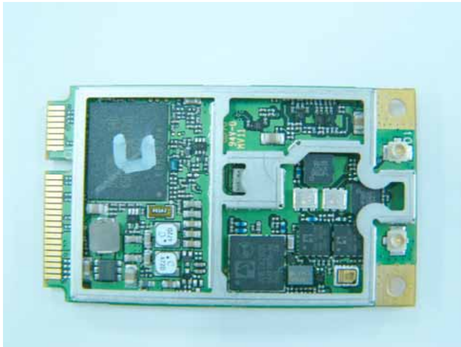
WWAN Module Interior Top View
