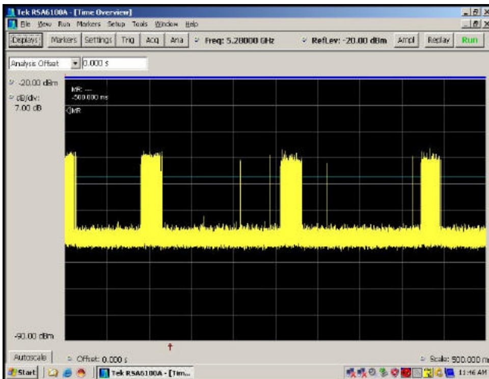
Figure 5-2. Time Display WLAN Channel Traffic (Streaming Video)
