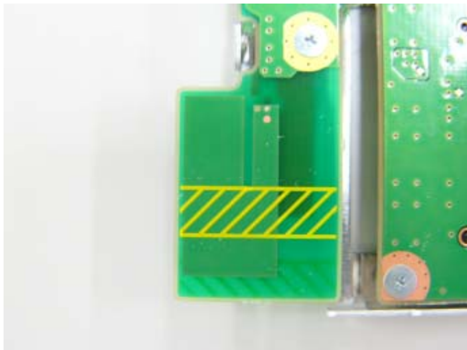
UNDP-1 Aux RX Antenna
