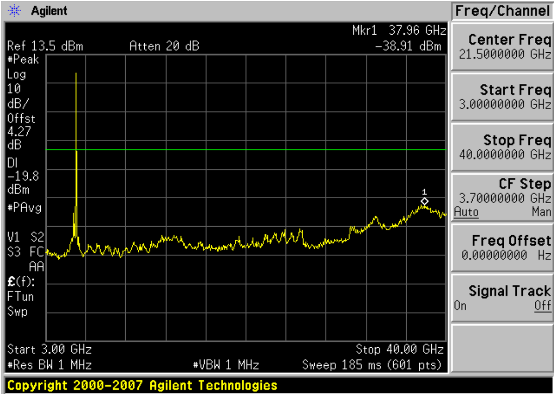
Plot 6-49. Conducted Spurious Plot (802.11a – Ch. 165)
