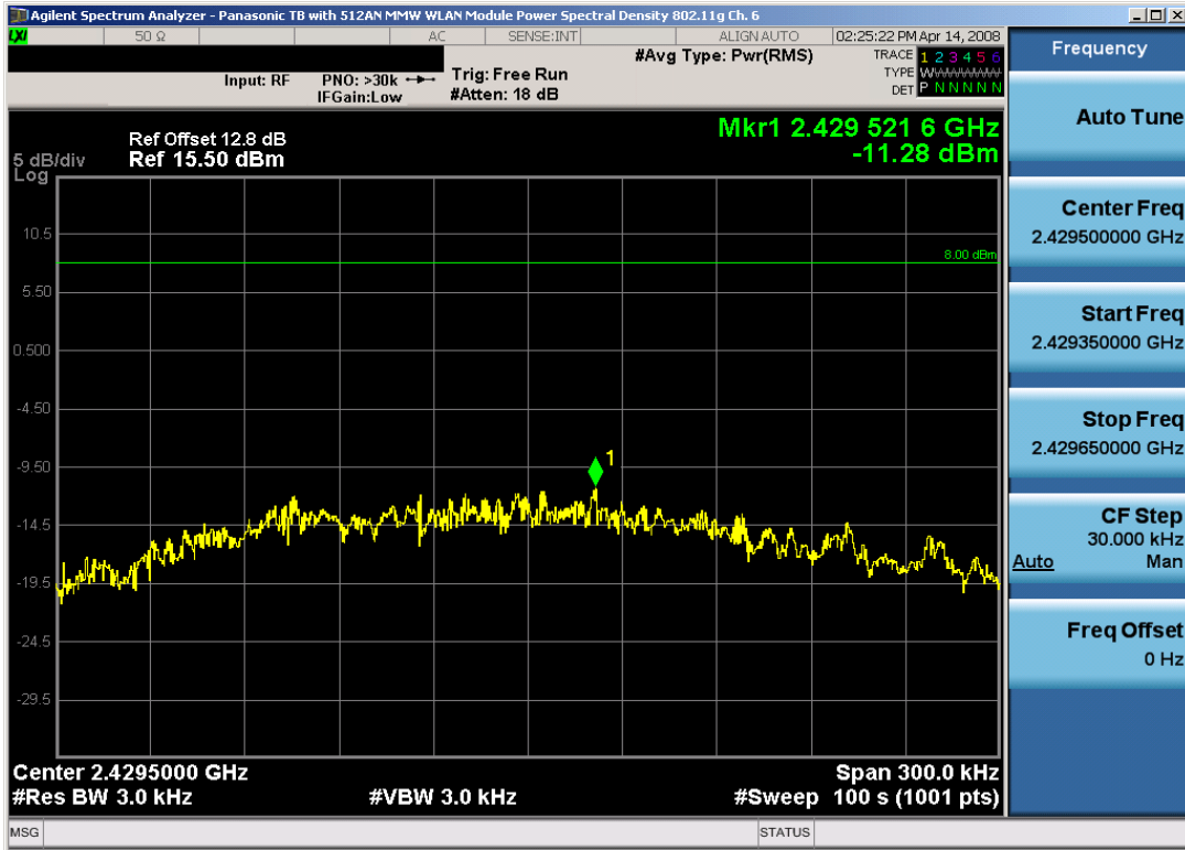
Plot 6-19. Power Spectral Density Plot (802.11g – Ch. 6)
