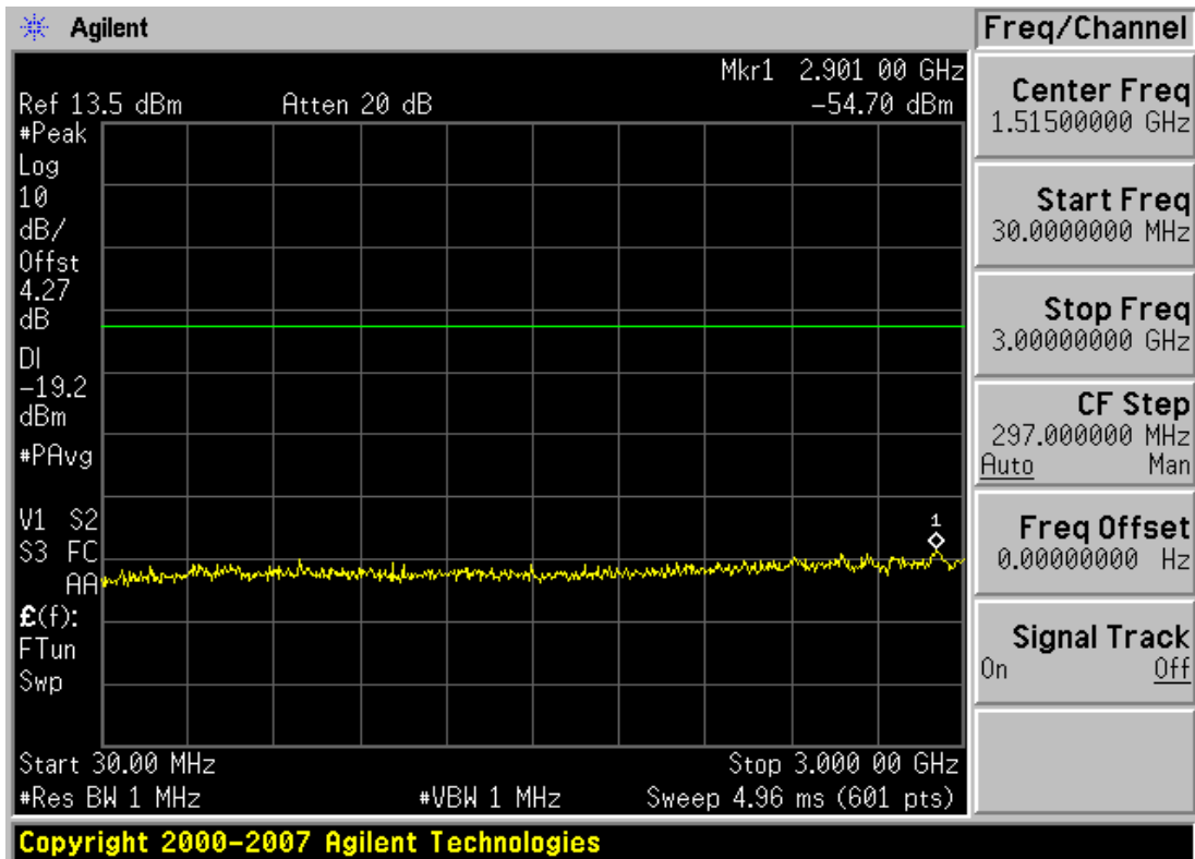
Plot 6-48. Conducted Spurious Plot (802.11a – Ch. 157)
