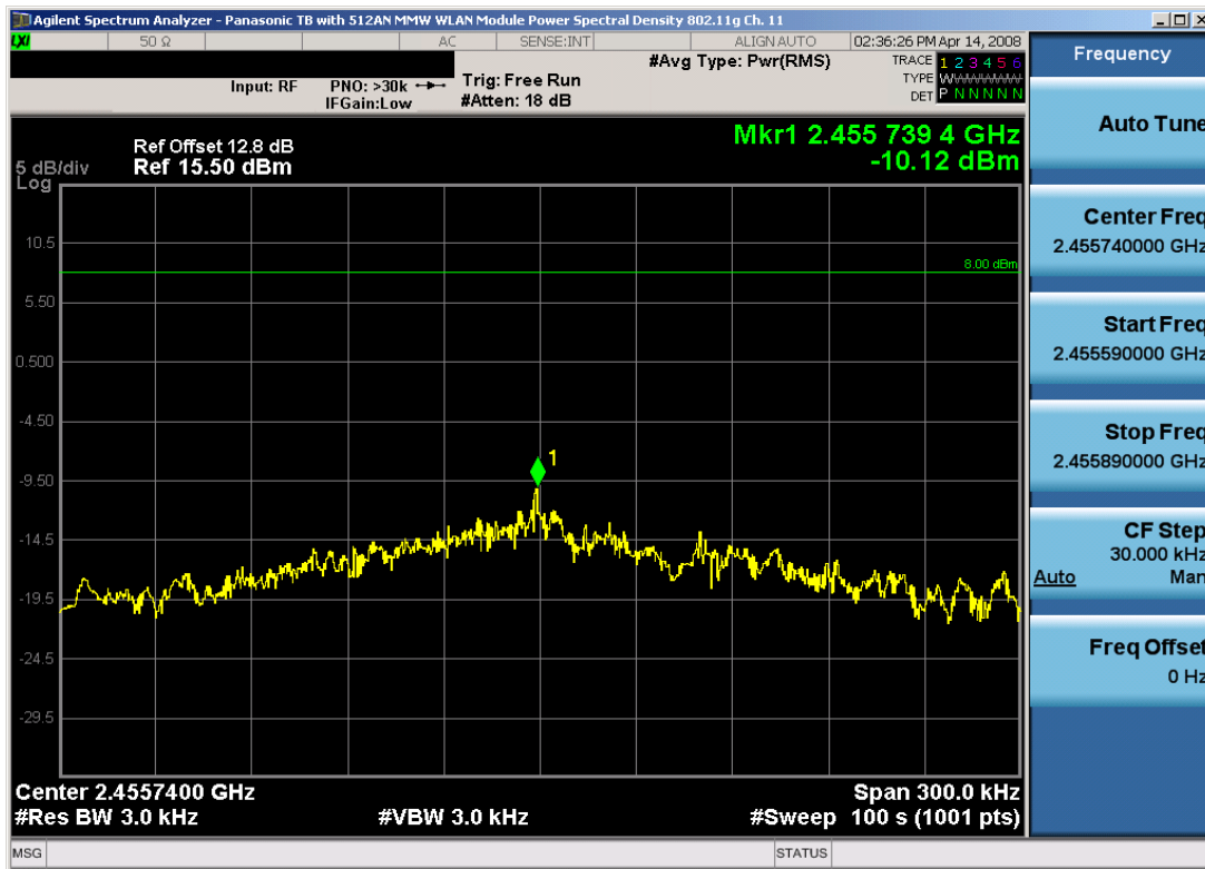
Plot 6-20. Power Spectral Density Plot (802.11g – Ch. 11)
