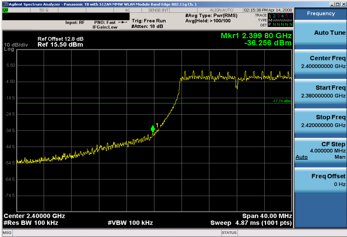
Plot 6-31. Band Edge Plot (802.11g – Ch. 1)
