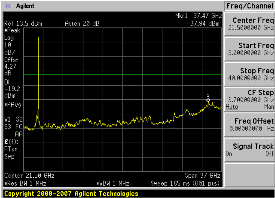
Plot 6-47. Conducted Spurious Plot (802.11a – Ch. 157)
