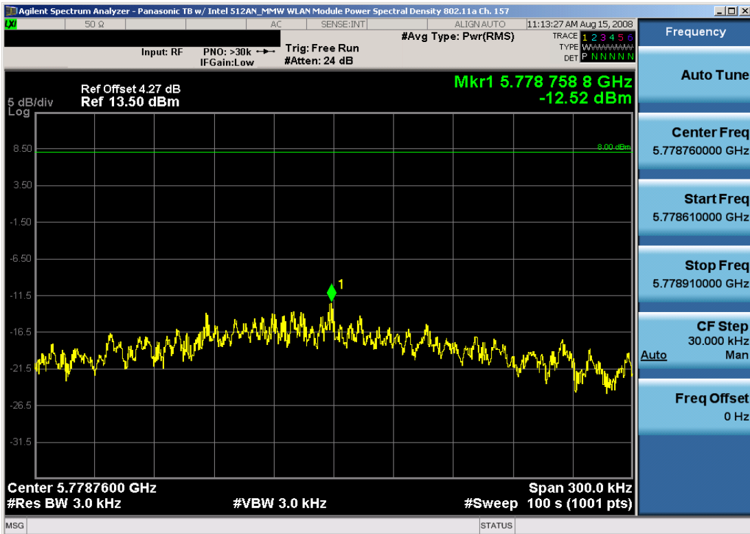
Plot 6-22. Power Spectral Density Plot (802.11a – Ch. 157)
