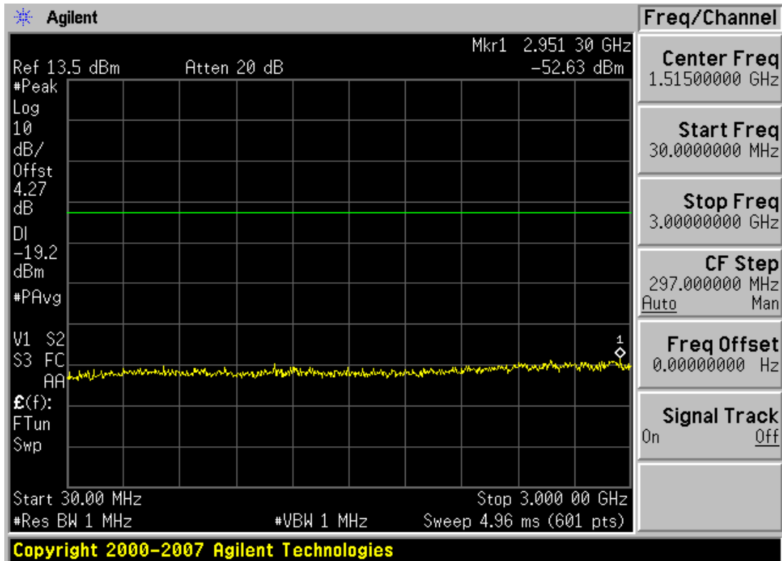
Plot 6-46. Conducted Spurious Plot (802.11a – Ch. 149)
