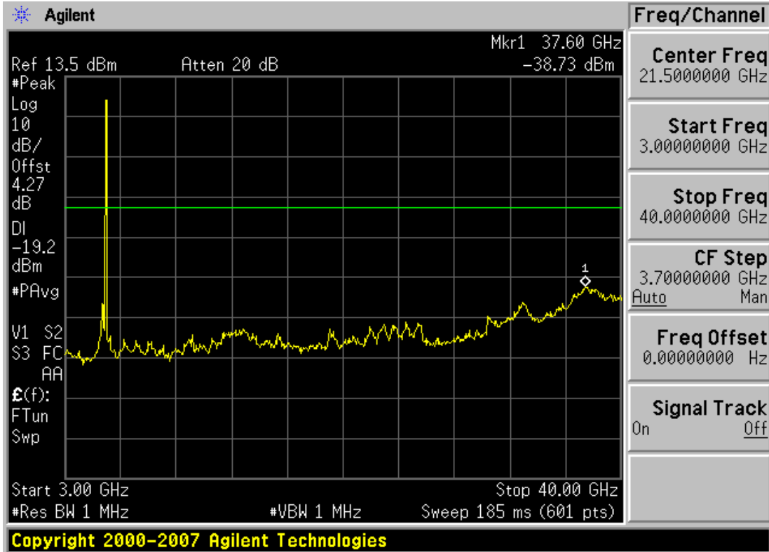
Plot 6-45. Conducted Spurious Plot (802.11a – Ch. 149)
