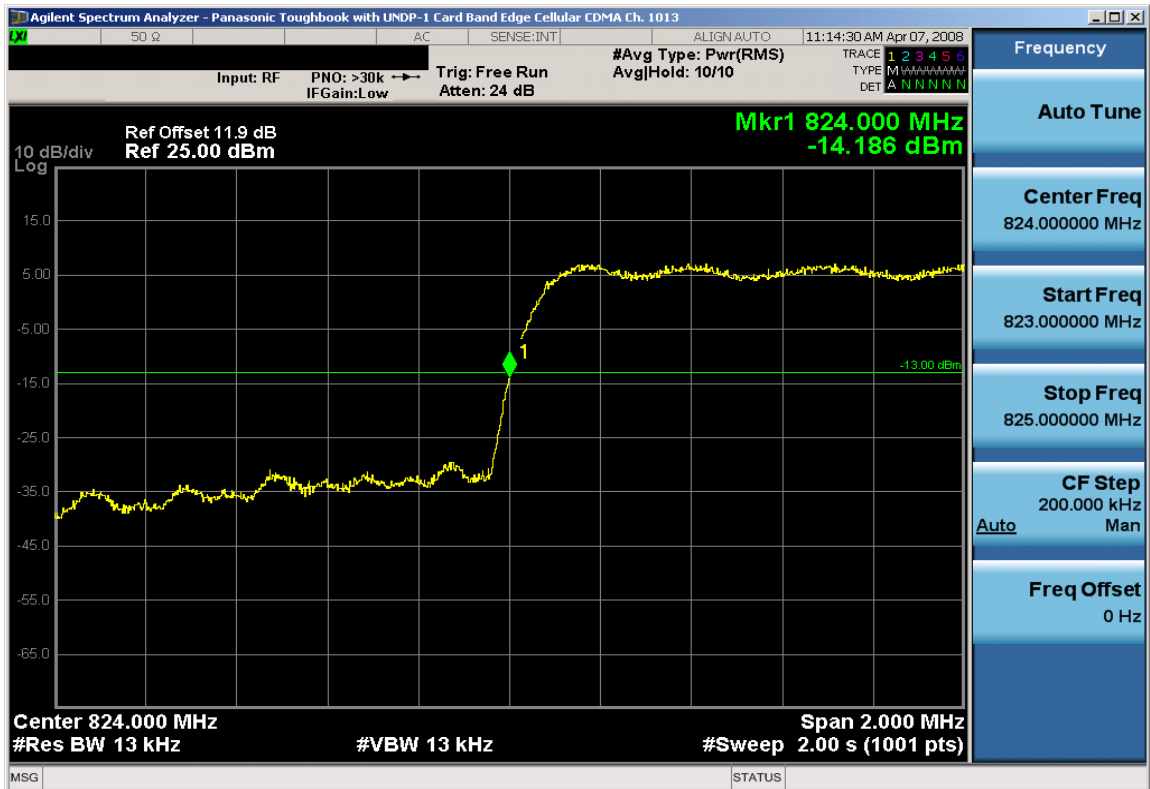
Plot 7-48. Band Edge Plot (Cellular CDMA Mode – Ch. 1013)
