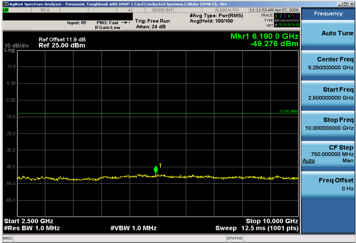
Plot 7-51. Conducted Spurious Plot (Cellular CDMA Mode – Ch. 384)
