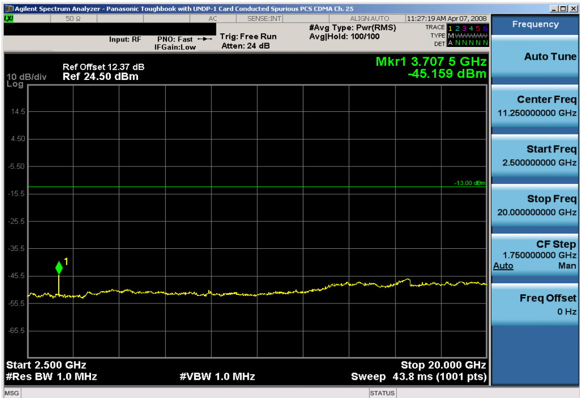
Plot 7-58. Conducted Spurious Plot (PCS CDMA Mode – Ch. 25)
