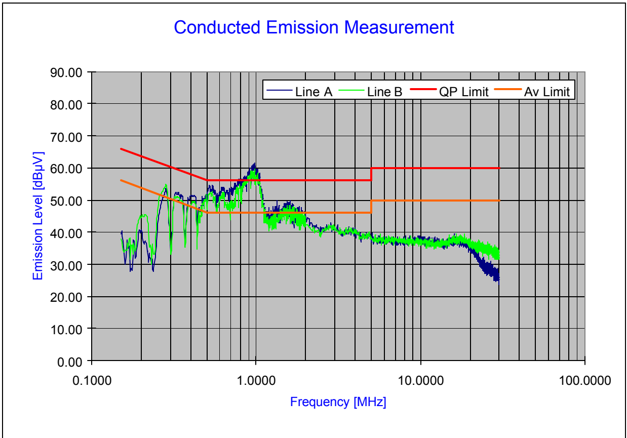
Plot 6-20. Line Conducted Plot with 802.11a (UNII-II Band)
