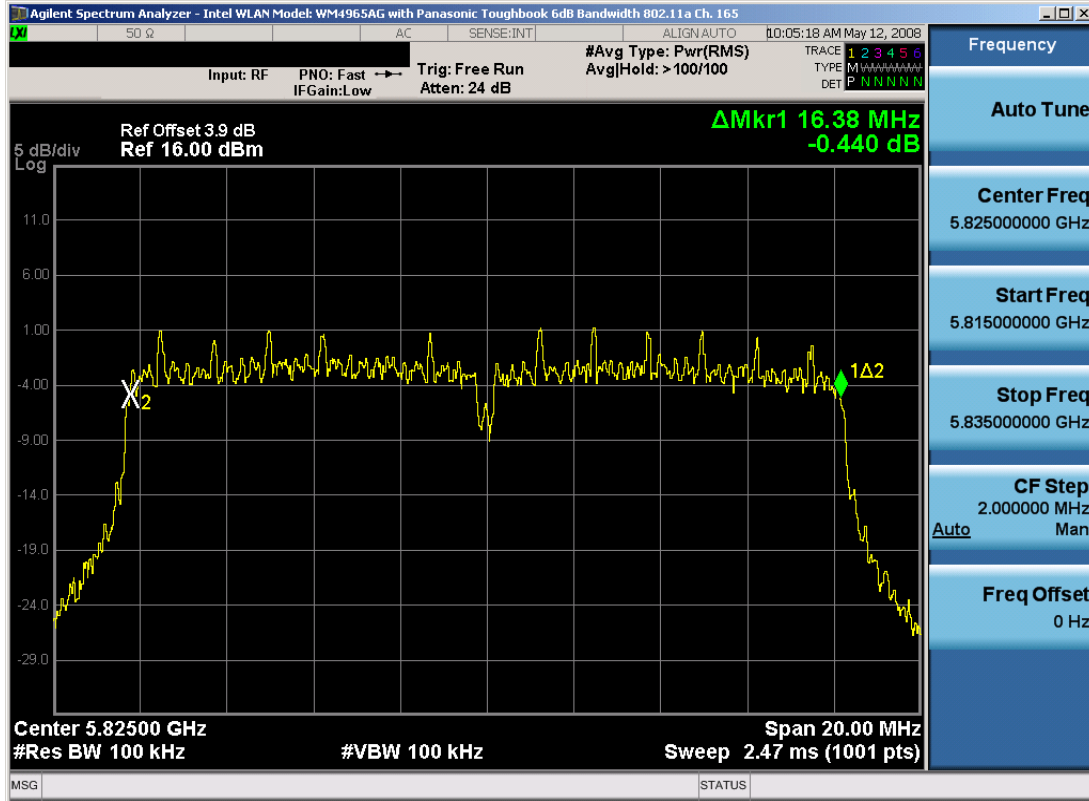
Plot 6-9. 6dB Bandwidth Plot (802.11a – Ch. 165)
