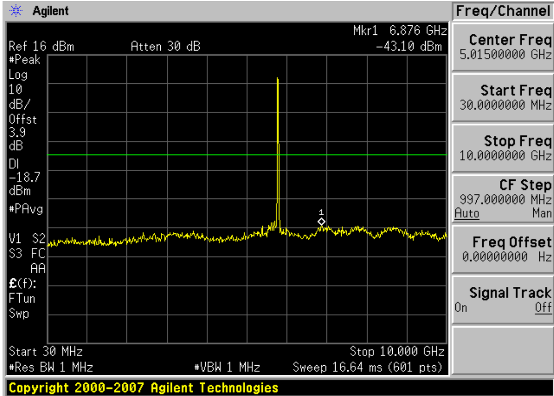
Plot 6-33. Conducted Spurious Plot (802.11a – Ch. 157)
