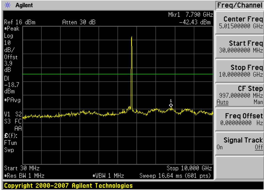
Plot 6-31. Conducted Spurious Plot (802.11a – Ch. 149)
