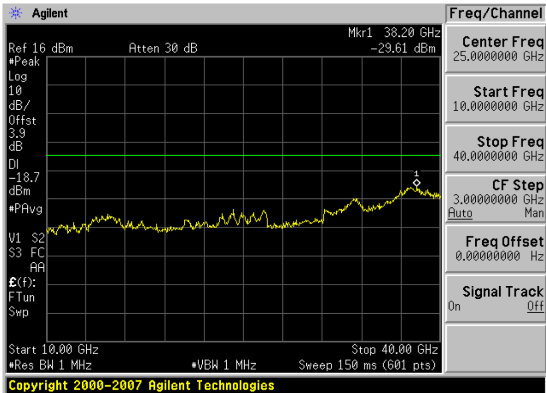
Plot 6-34. Conducted Spurious Plot (802.11a – Ch. 157)
