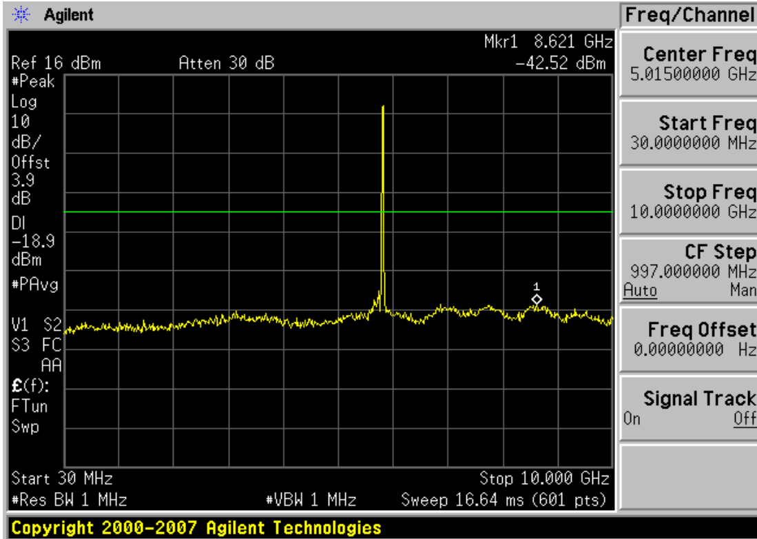
Plot 6-35. Conducted Spurious Plot (802.11a – Ch. 165)
