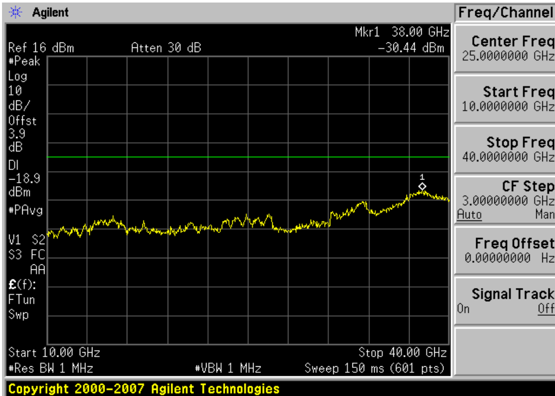
Plot 6-36. Conducted Spurious Plot (802.11a – Ch. 165)
