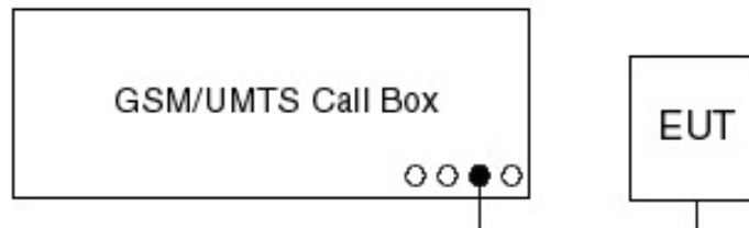
Figure 6-1. GSM/WCDMA Conducted Power Test Setup Diagram
