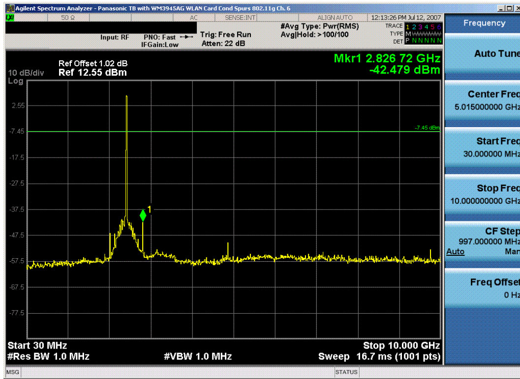
Plot 6-19. Conducted Spurious Plot (802.11g – Ch. 6)
