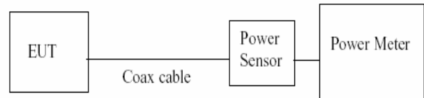
Figure 6-3. Test Instrument & Measurement Setup
