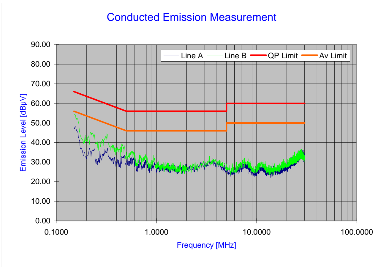
Plot 6-29. Line Conducted Plot with 802.11a
