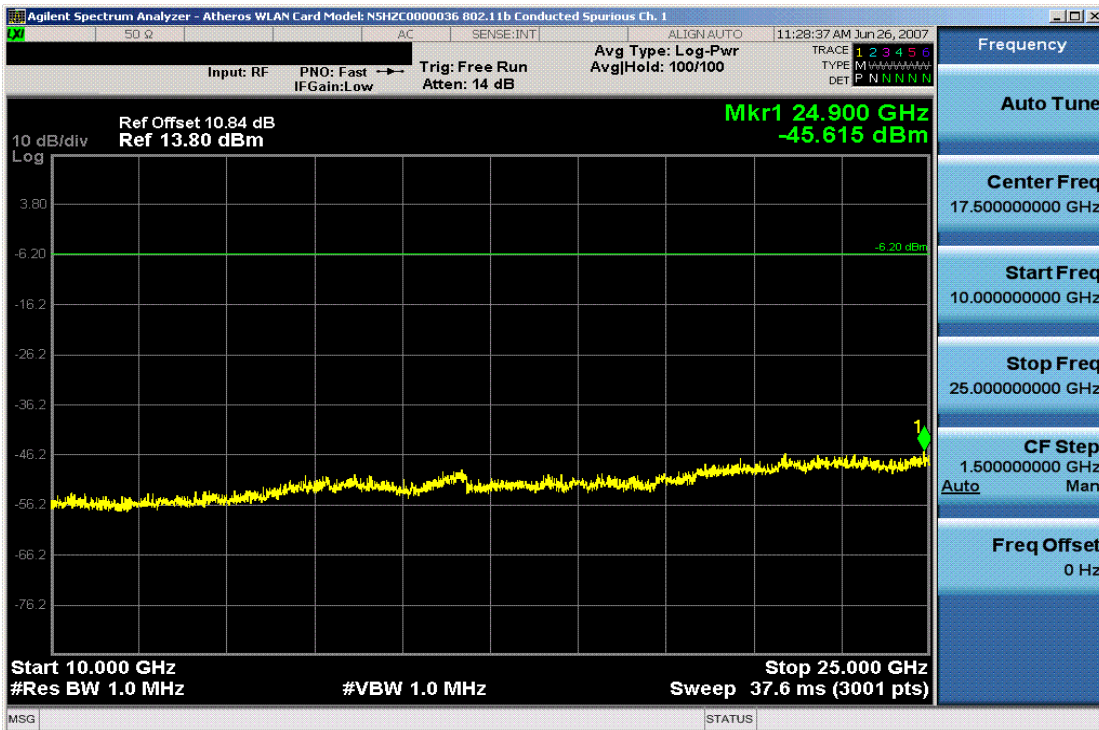
Plot 6-22. Conducted Spurious Plot (802.11b – Ch. 1)
