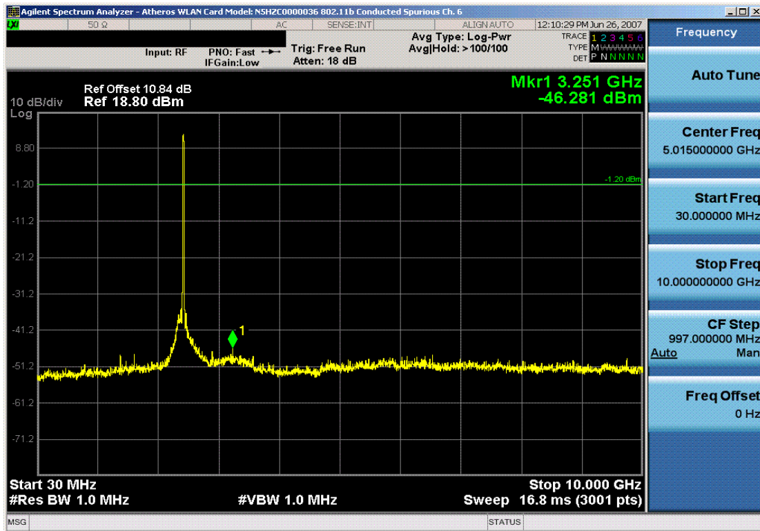
Plot 6-23. Conducted Spurious Plot (802.11b – Ch. 6)
