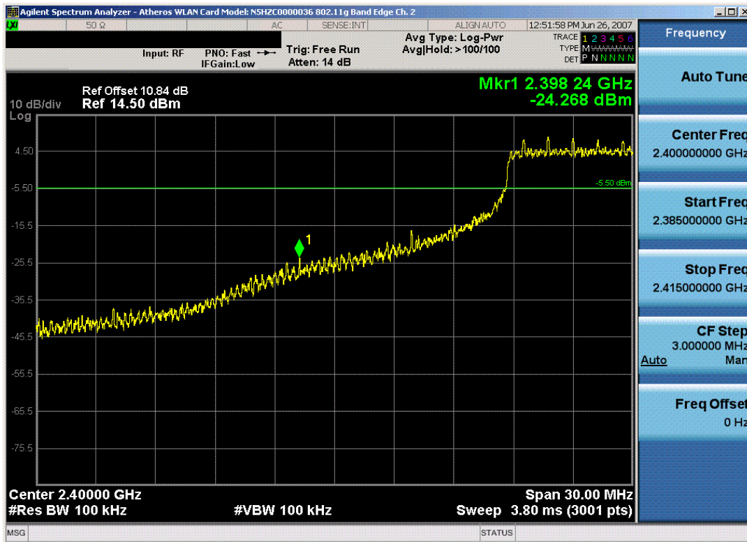
Plot 6-18. Band Edge Plot (802.11g – Ch. 2)
