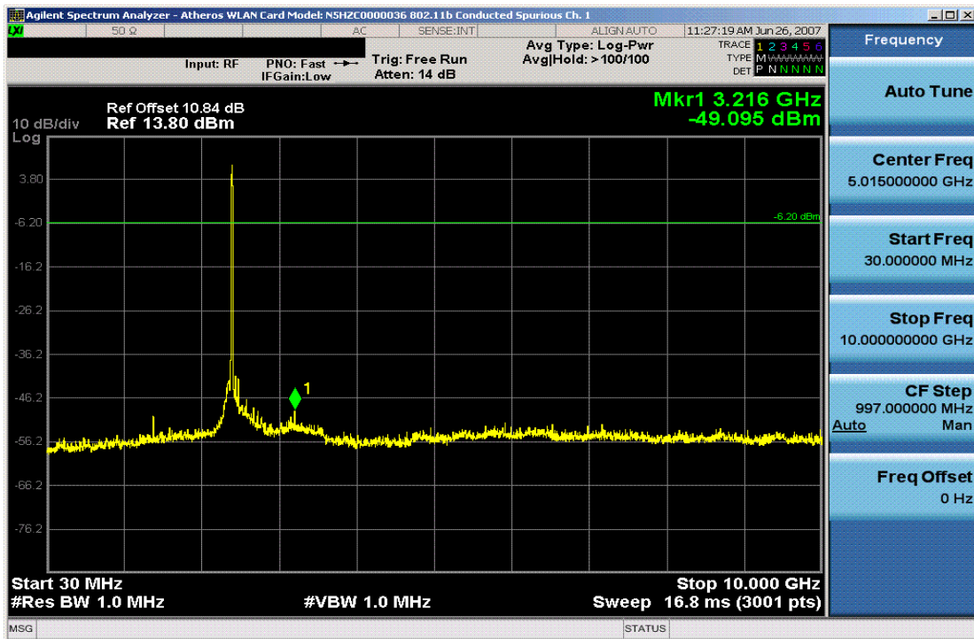
Plot 6-21. Conducted Spurious Plot (802.11b – Ch. 1)
