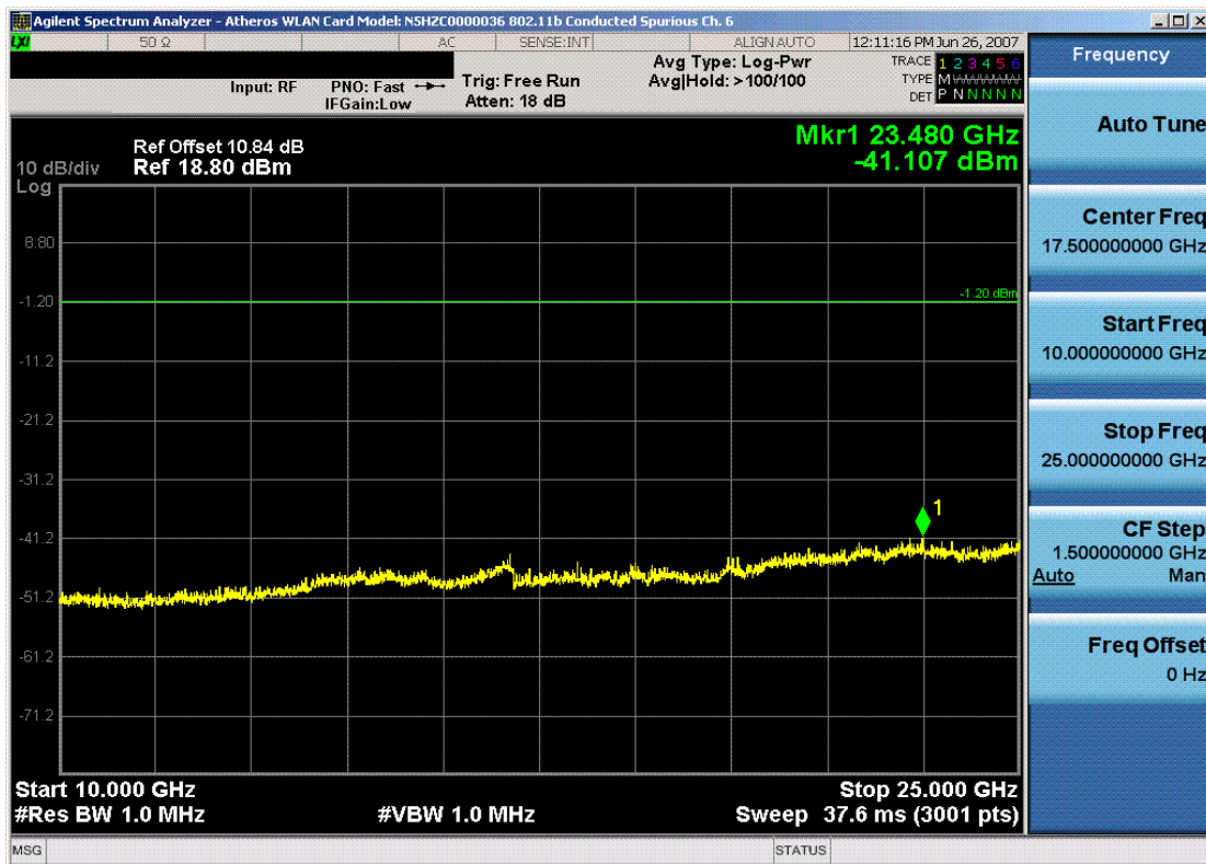
Plot 6-24. Conducted Spurious Plot (802.11b – Ch. 6)
