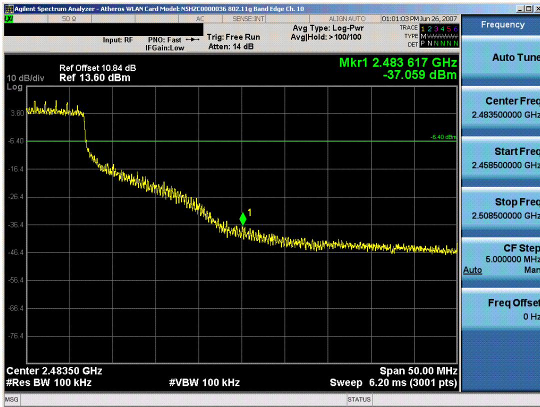
Plot 6-19. Band Edge Plot (802.11g – Ch. 10)
