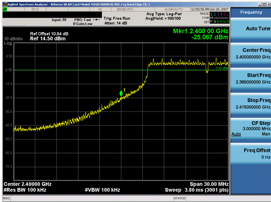
Plot 6-17. Band Edge Plot (802.11g – Ch. 1)
