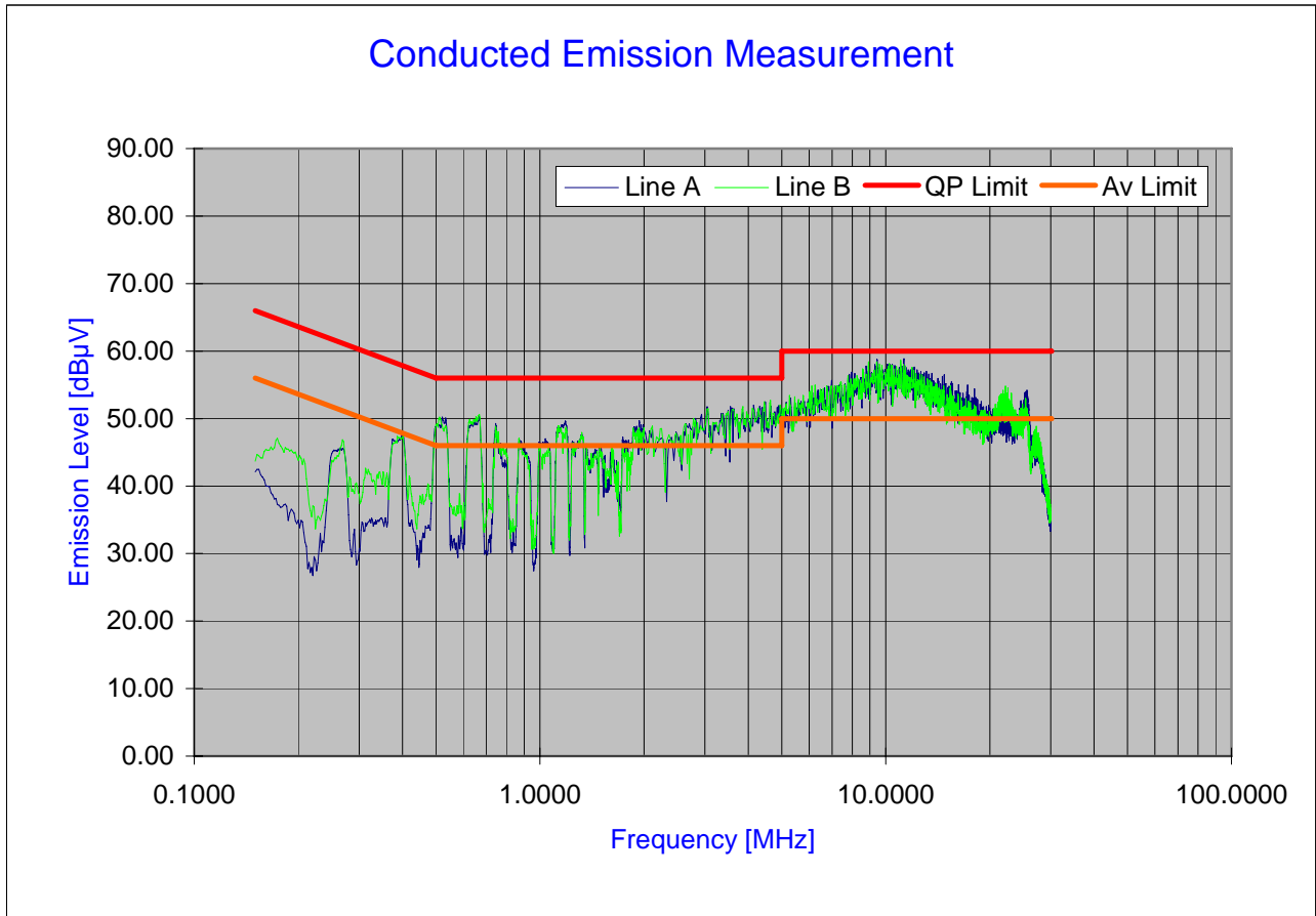
Plot 6-28. Line Conducted Plot with 802.11g
