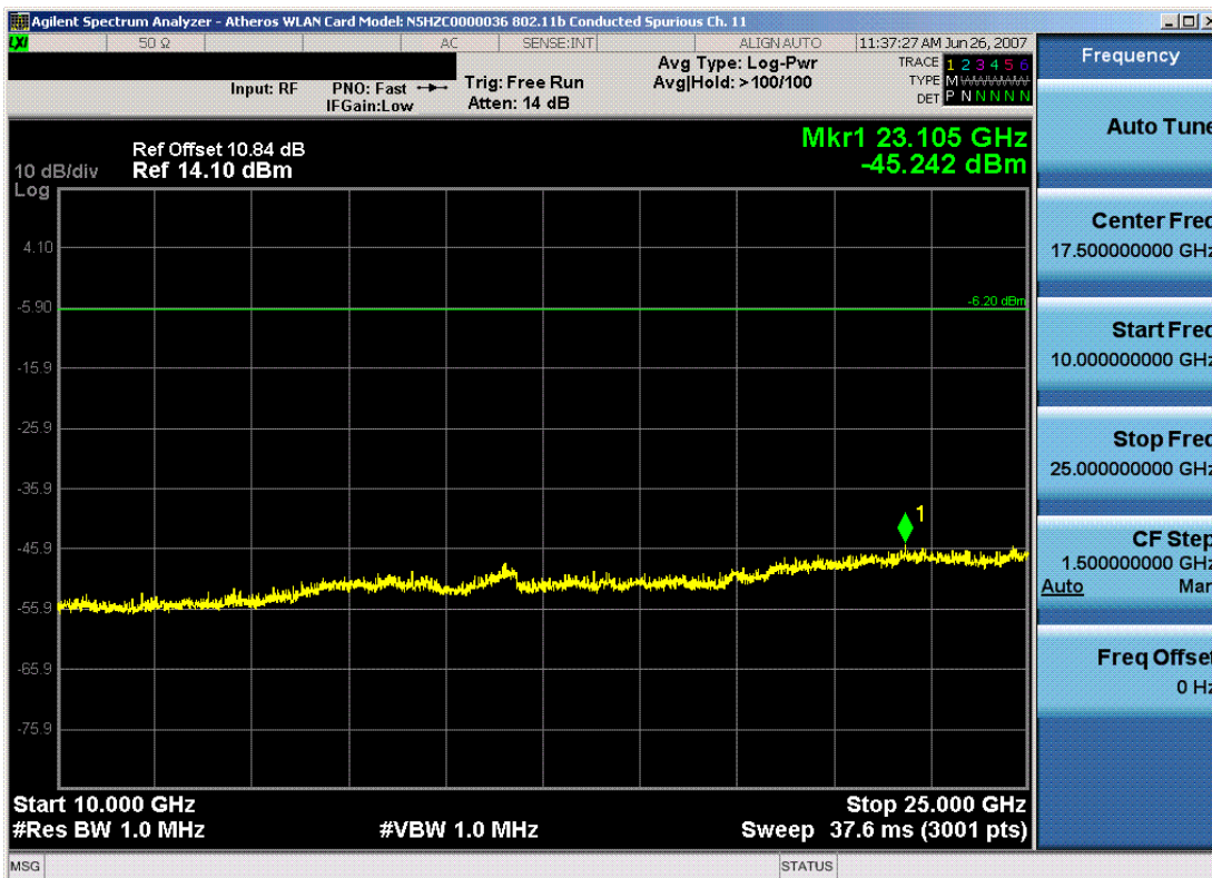
Plot 6-26. Conducted Spurious Plot (802.11b – Ch. 11)
