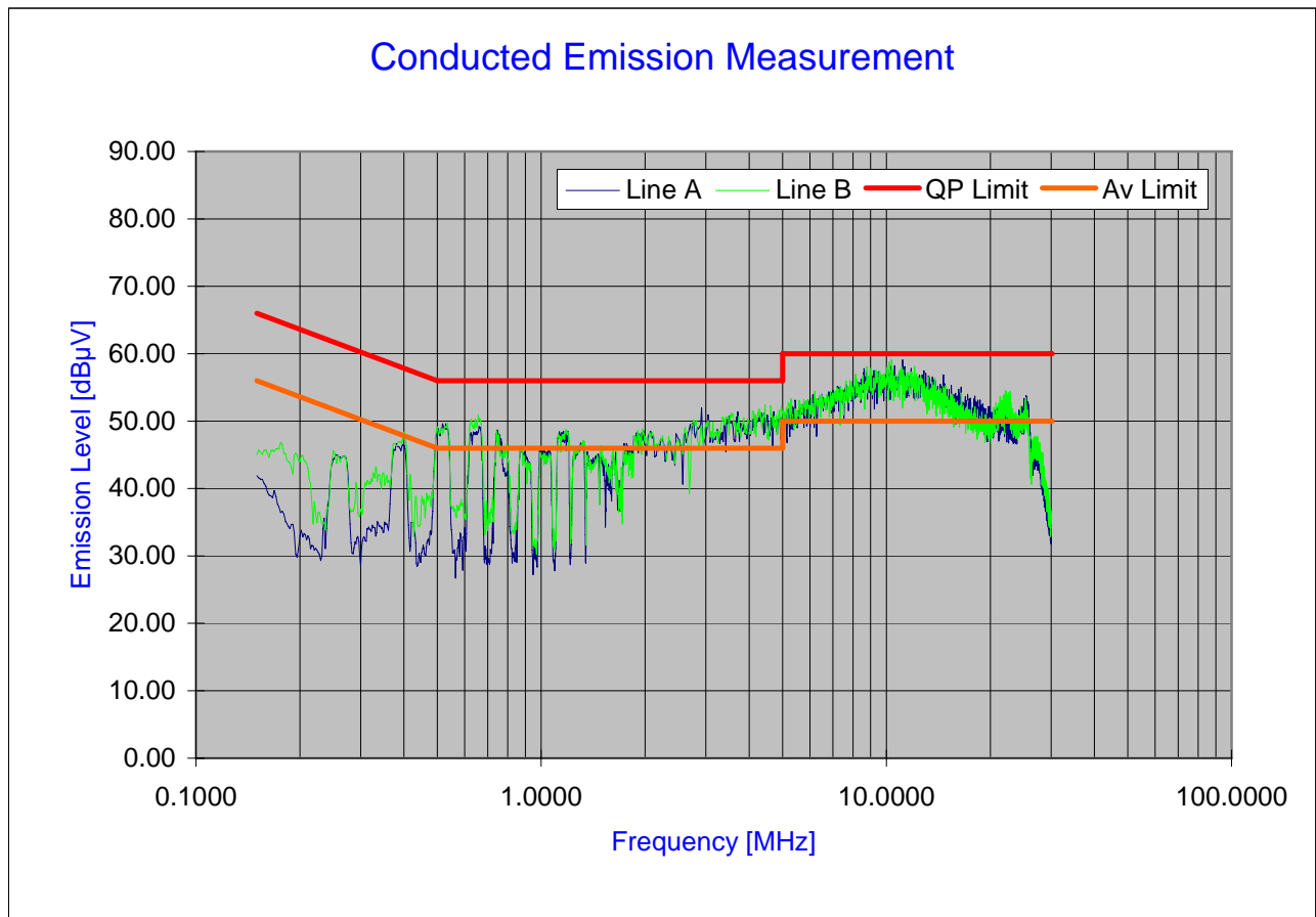
Plot 6-27. Line Conducted Plot with 802.11b
