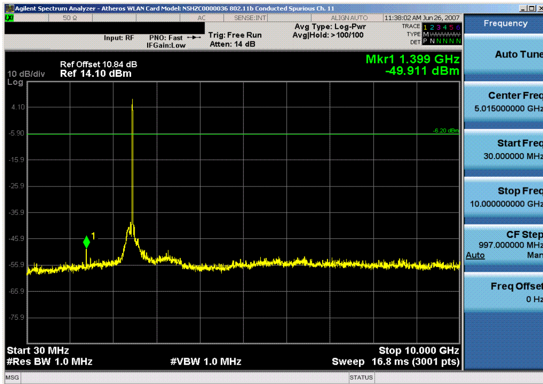
Plot 6-25. Conducted Spurious Plot (802.11b – Ch. 11)
