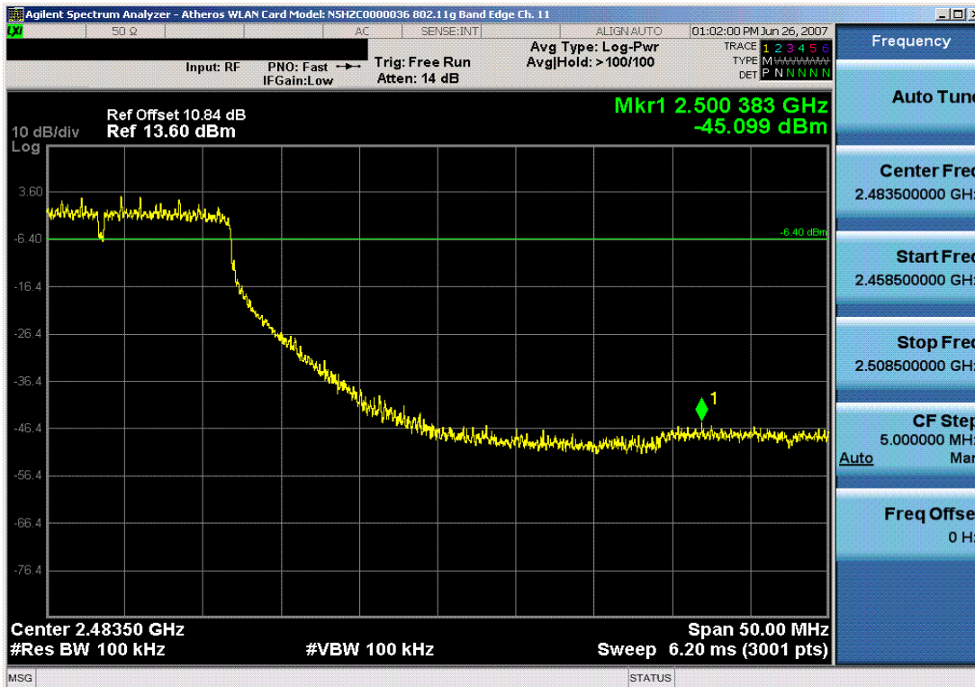
Plot 6-20. Band Edge Plot (802.11g – Ch. 11)
