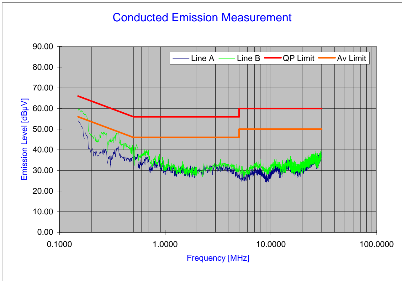
Plot 6-27. Line Conducted Plot with 802.11g
