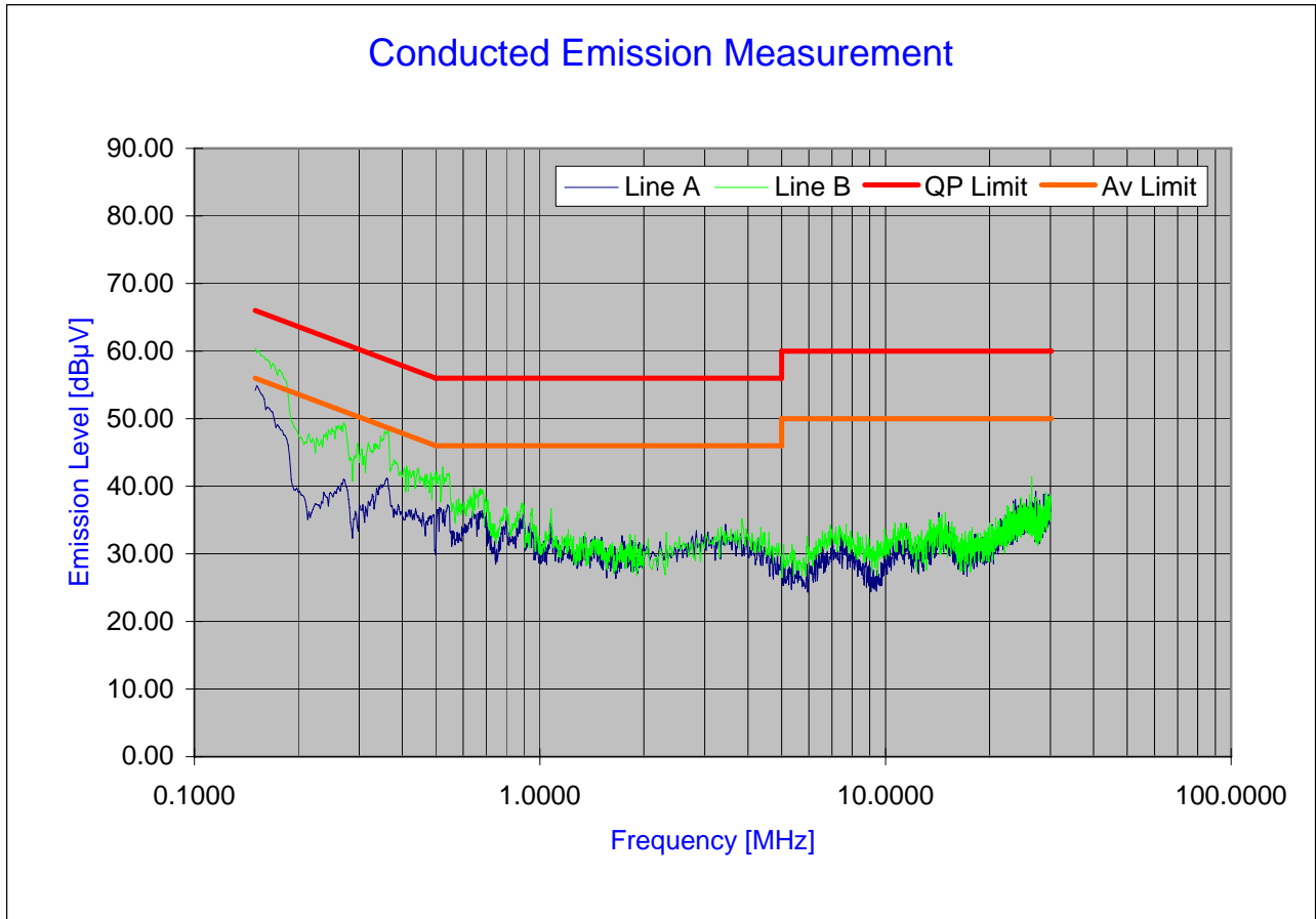
Plot 6-25. Line Conducted Plot with 802.11a
