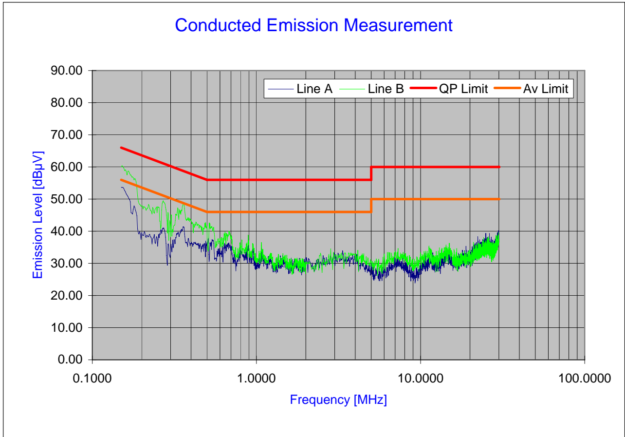
Plot 6-26. Line Conducted Plot with 802.11b
