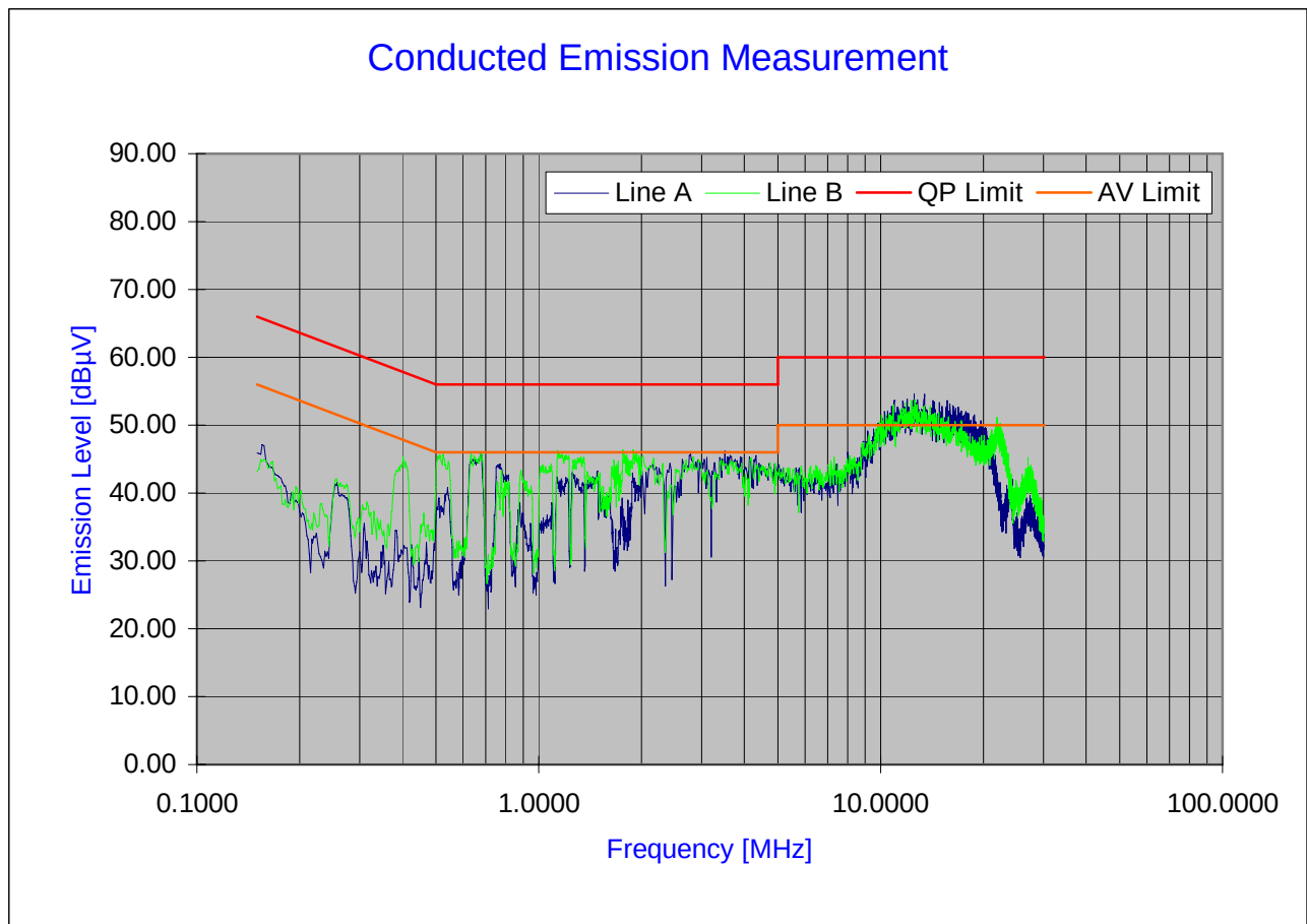
Plot 6-25. Line Conducted Plot with 802.11b
