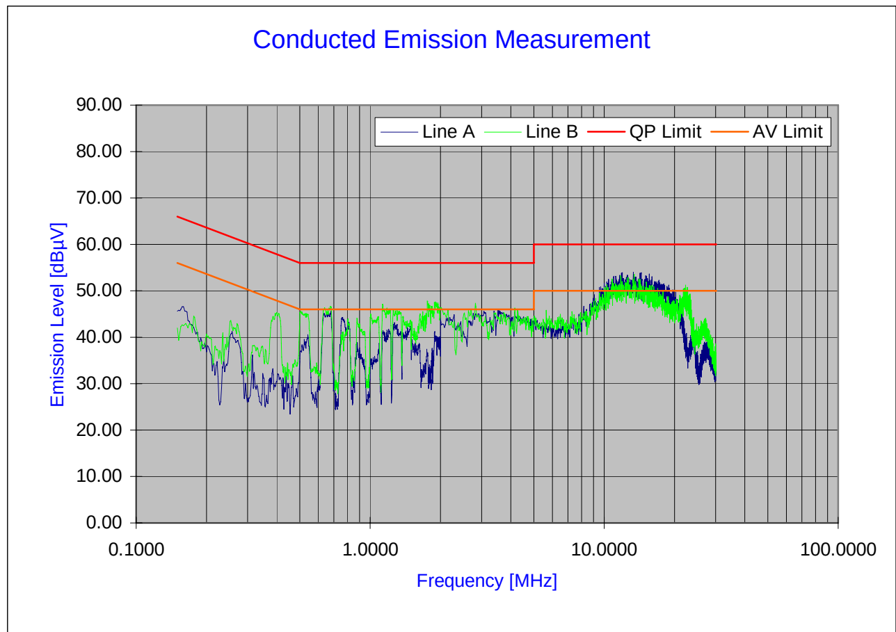
Plot 6-27. Line Conducted Plot with 802.11a
