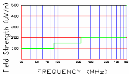
Figure A-1. Radiated limits at 3 meters.
