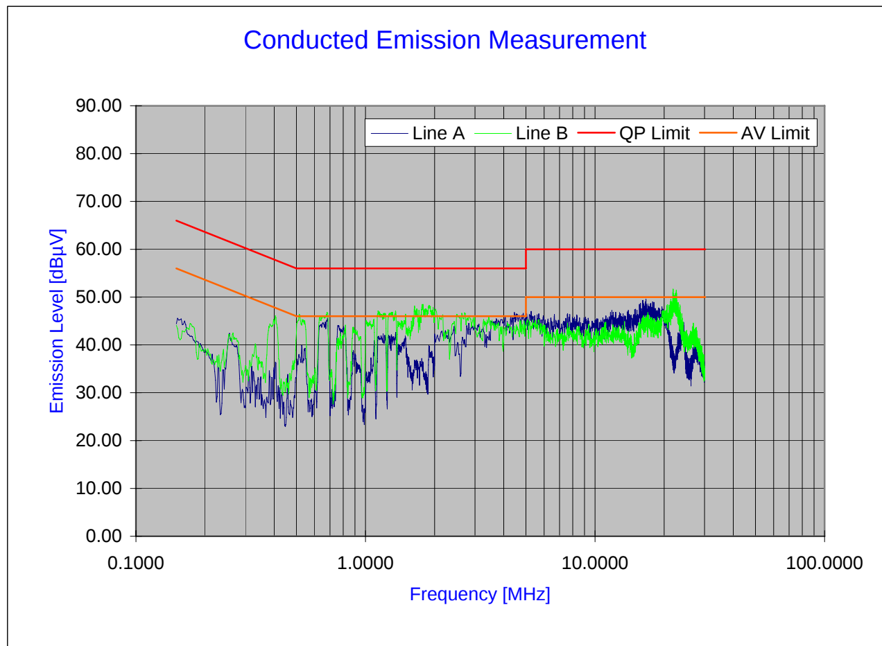
Plot 6-13. Line Conducted Plot with 802.11a (UNII Low Band)
