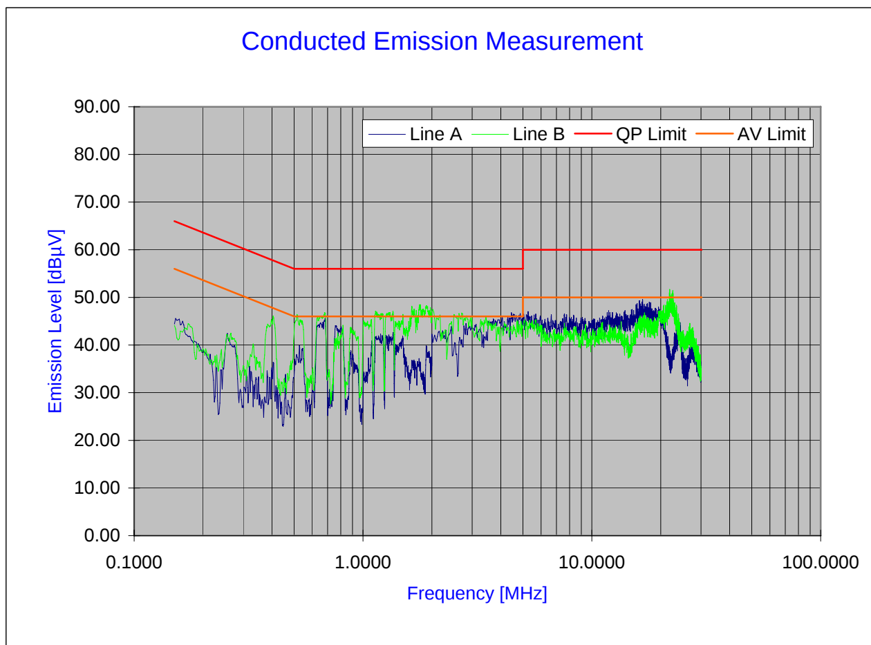
Plot 6-27. Line Conducted Plot with 802.11a
