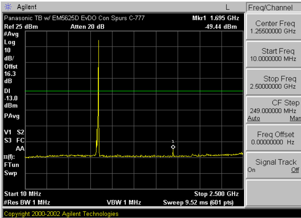
Plot A-9. Conducted Spurious Plot (Cellular CDMA EvDO Mode – Ch. 777)
