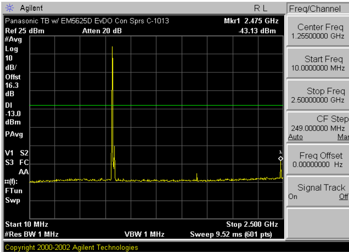
Plot A-1. Conducted Spurious Plot (Cellular CDMA EvDO Mode – Ch. 1013)
