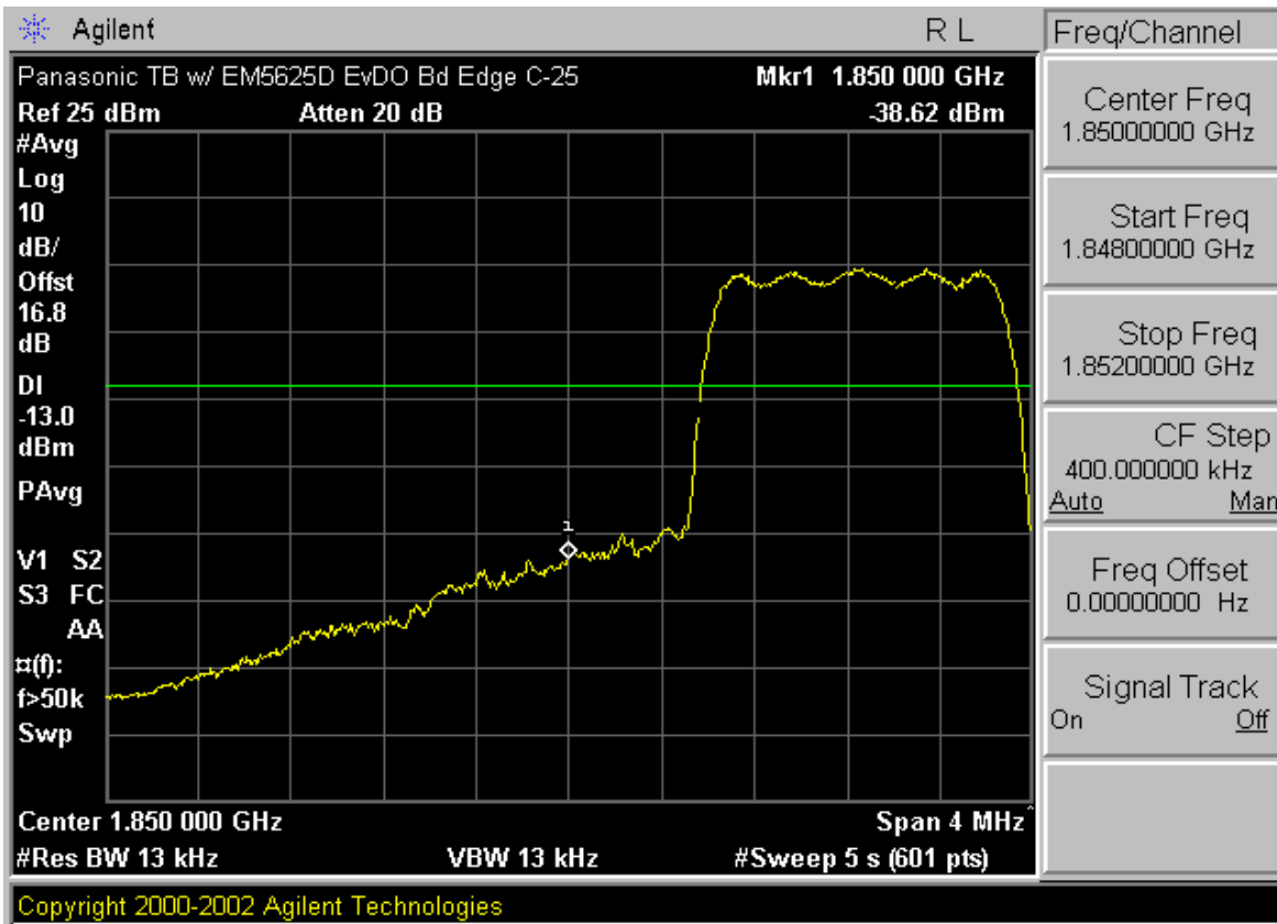
Plot A-15. Band Edge Plot (PCS CDMA EvDO Mode – Ch. 25)
