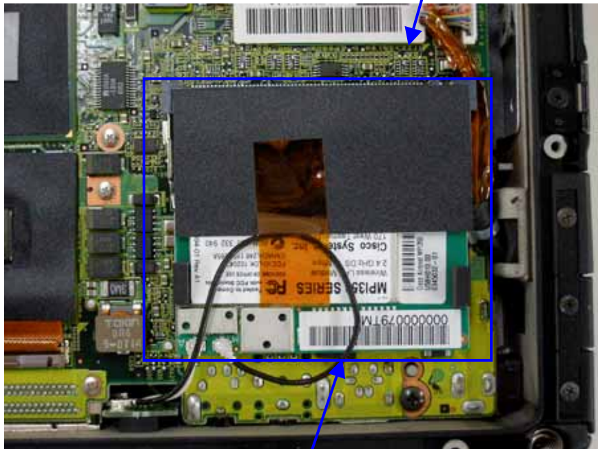
WLAN Card Position
