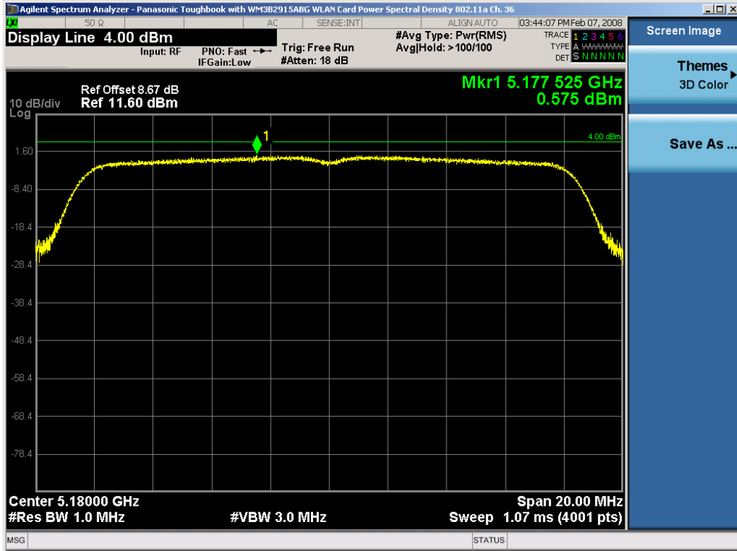
Plot 6-7. Peak Power Spectral Density Plot (802.11a (UNII) – Ch. 36)
