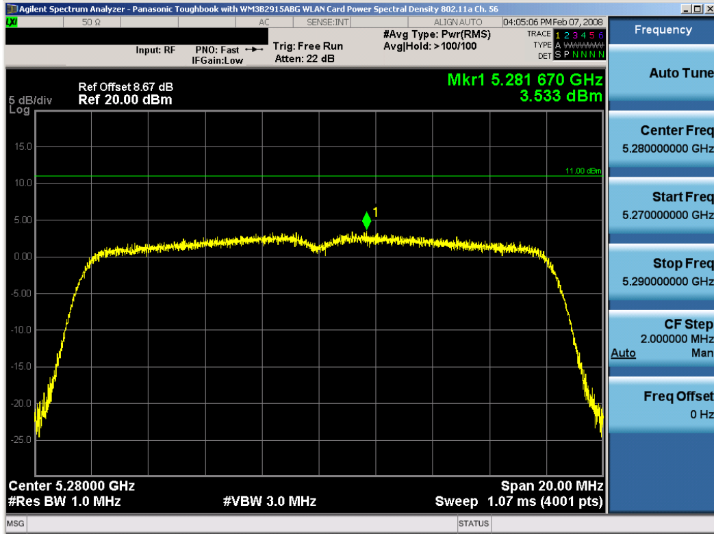
Plot 6-11. Peak Power Spectral Density Plot (802.11a (UNII) – Ch. 56)
