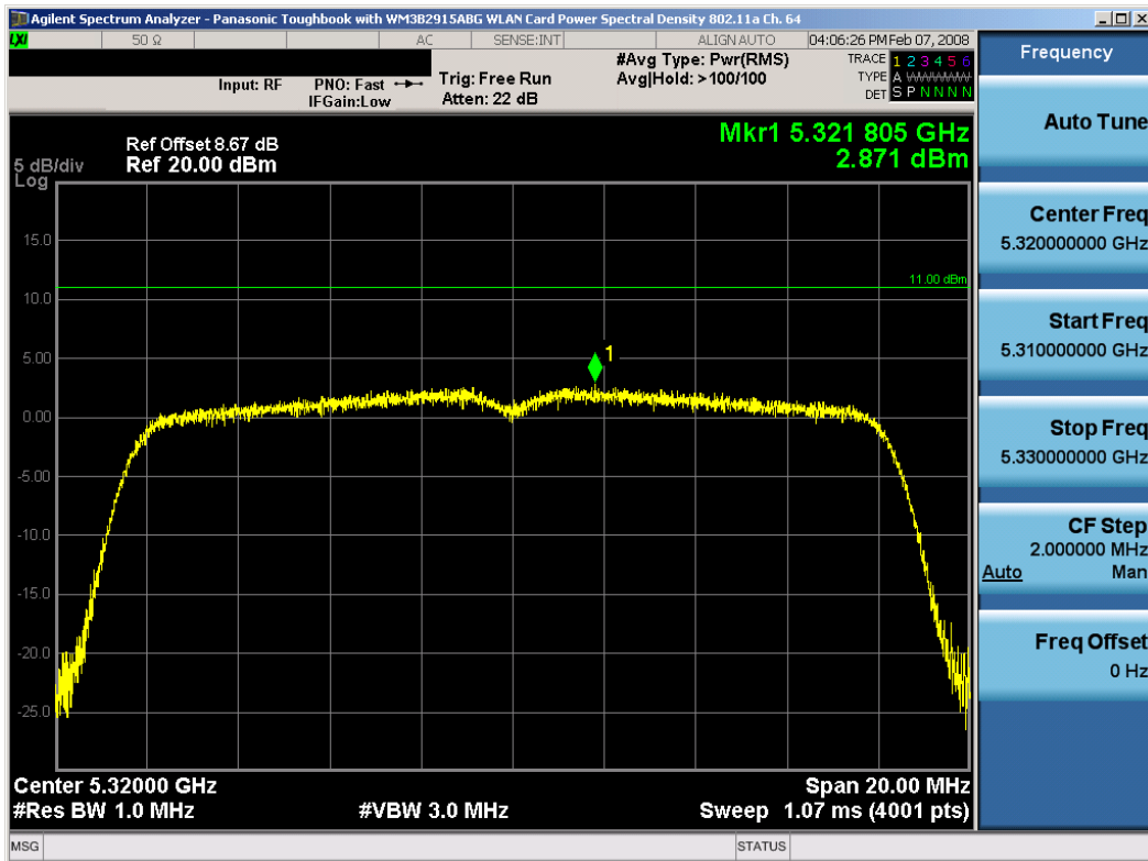
Plot 6-12. Peak Power Spectral Density Plot (802.11a (UNII) – Ch. 64)
