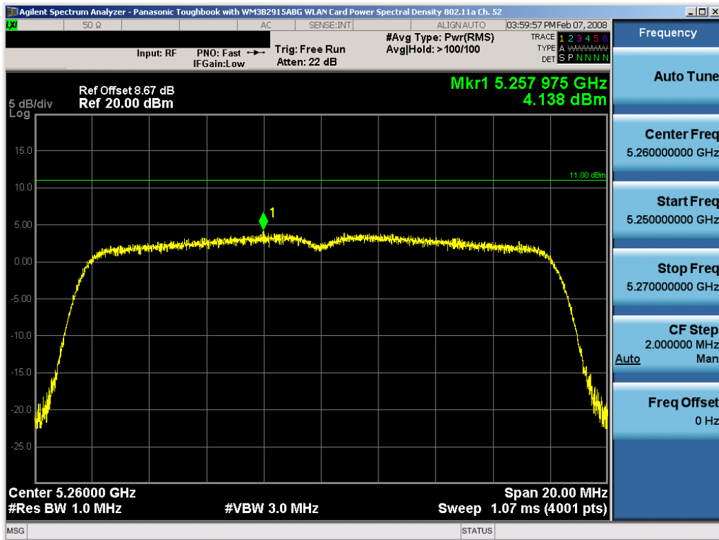
Plot 6-10. Peak Power Spectral Density Plot (802.11a (UNII) – Ch. 52)
