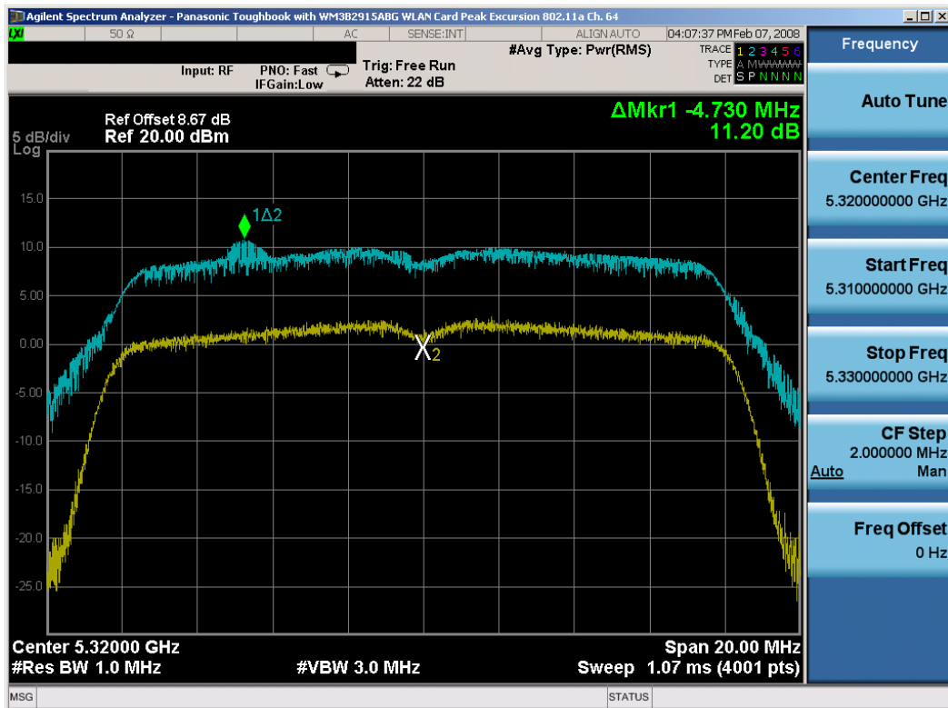
Plot 6-18. Excursion Ratio Plot (802.11a (UNII) – Ch. 64)
