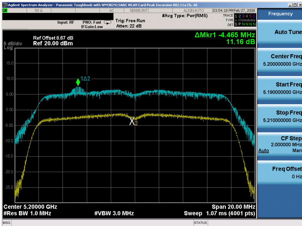
Plot 6-14. Peak Excursion Ratio Plot (802.11a (UNII) – Ch. 40)
