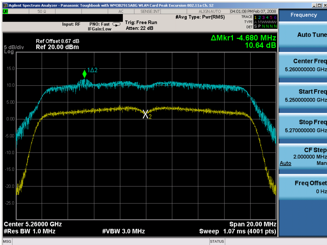
Plot 6-16. Peak Excursion Ratio Plot (802.11a (UNII) – Ch. 52)
