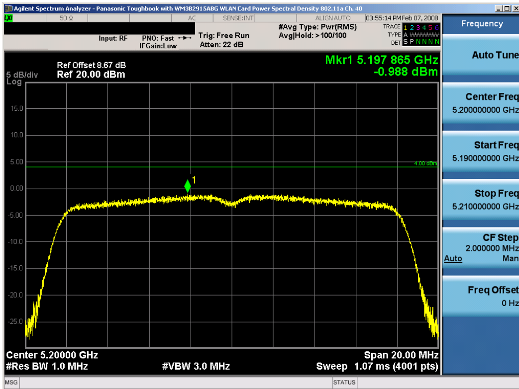
Plot 6-8. Peak Power Spectral Density Plot (802.11a (UNII) – Ch. 40)
