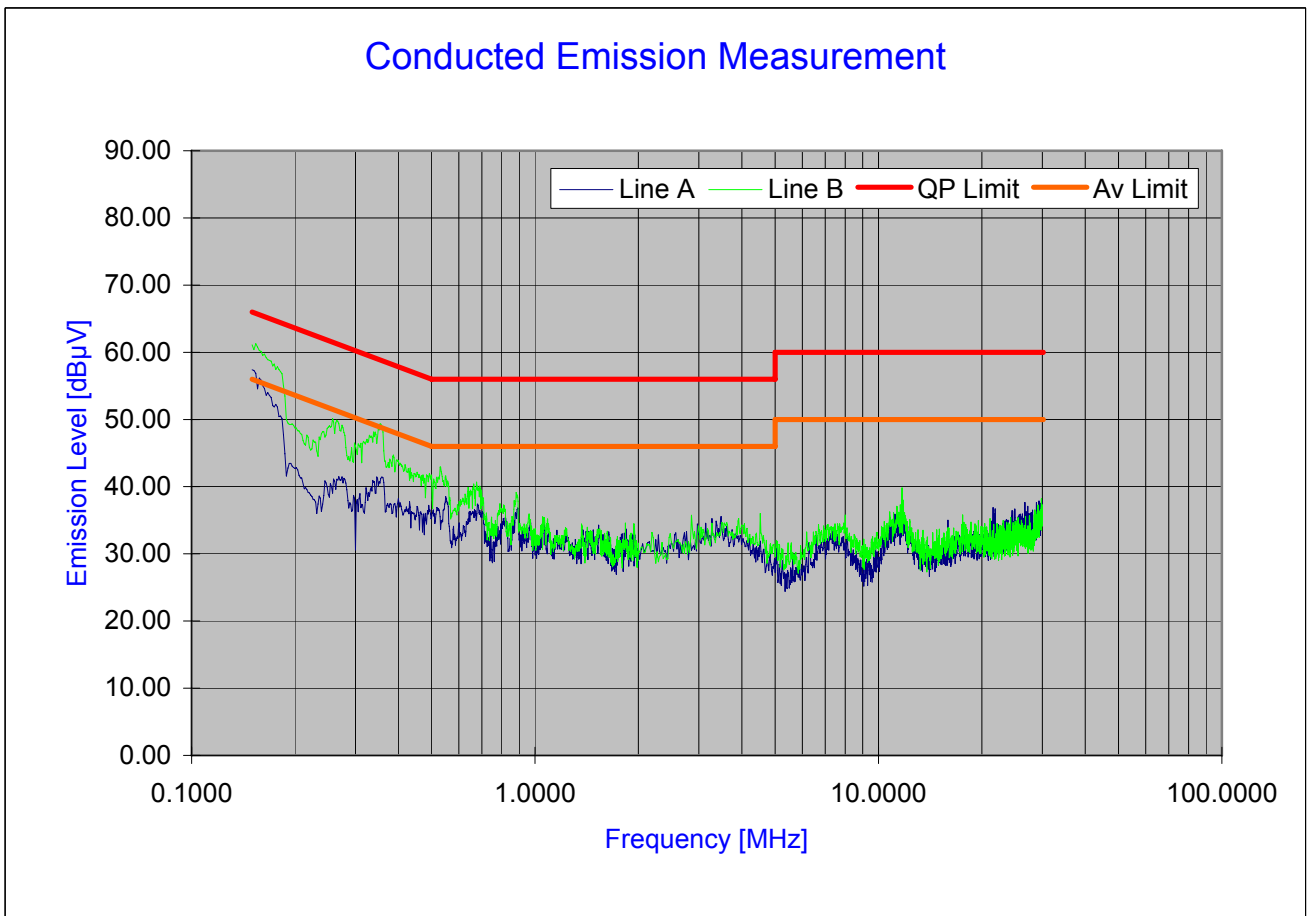
Plot 6-19. Line Conducted Plot with 802.11a (UNII-I Band)
