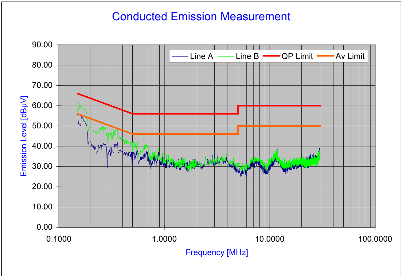
Plot 6-20. Line Conducted Plot with 802.11a (UNII-II Band)
