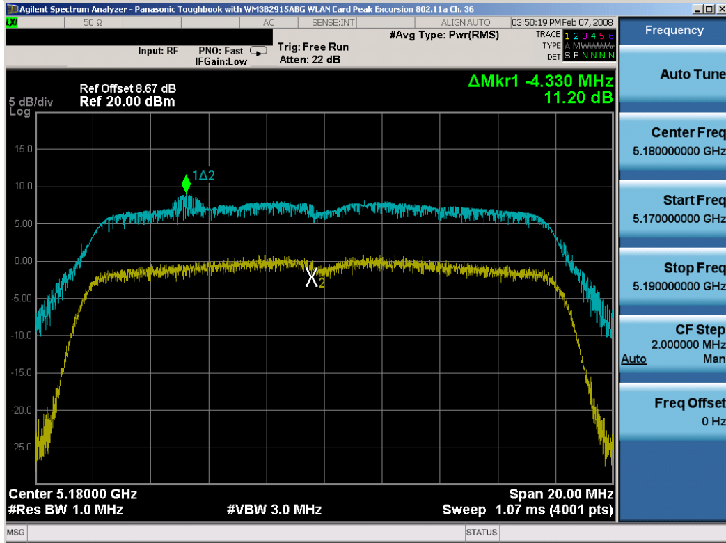
Plot 6-13. Peak Excursion Ratio Plot (802.11a (UNII) – Ch. 36)
