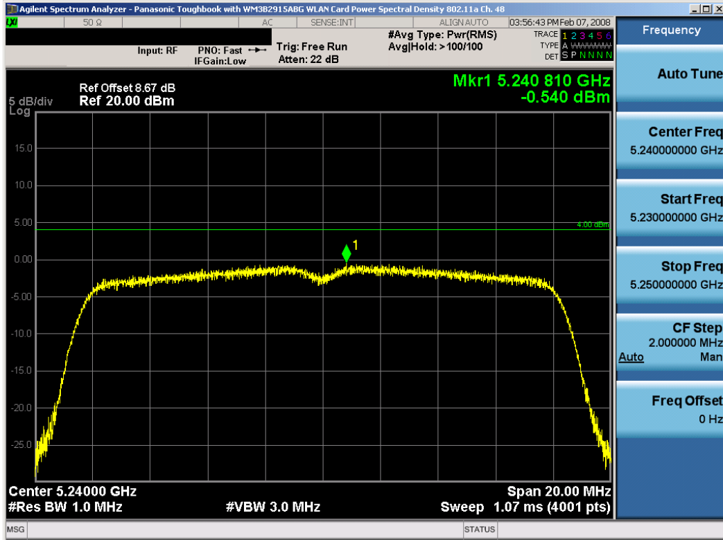
Plot 6-9. Peak Power Spectral Density Plot (802.11a (UNII) – Ch. 48)
