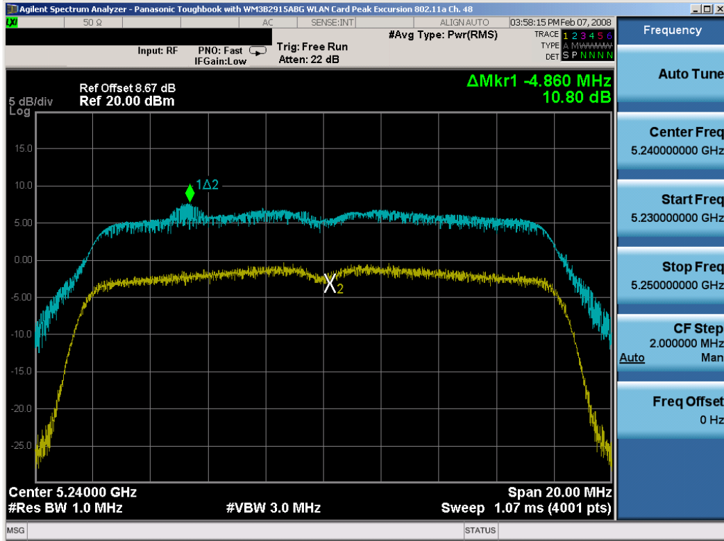
Plot 6-15. Peak Excursion Ratio Plot (802.11a (UNII) – Ch. 48)
