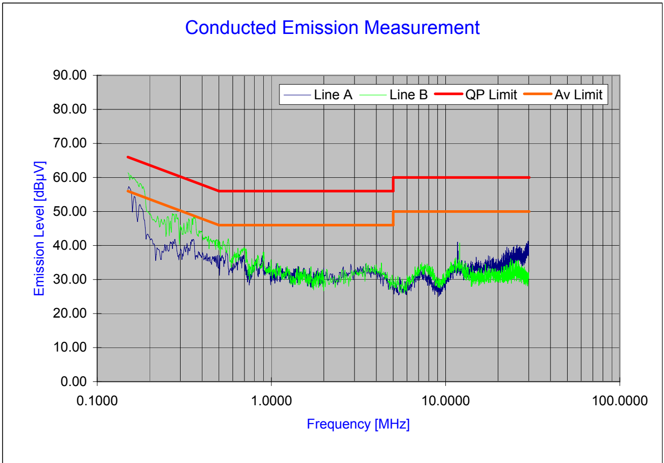
Plot 6-39. Line Conducted Plot with 802.11a
