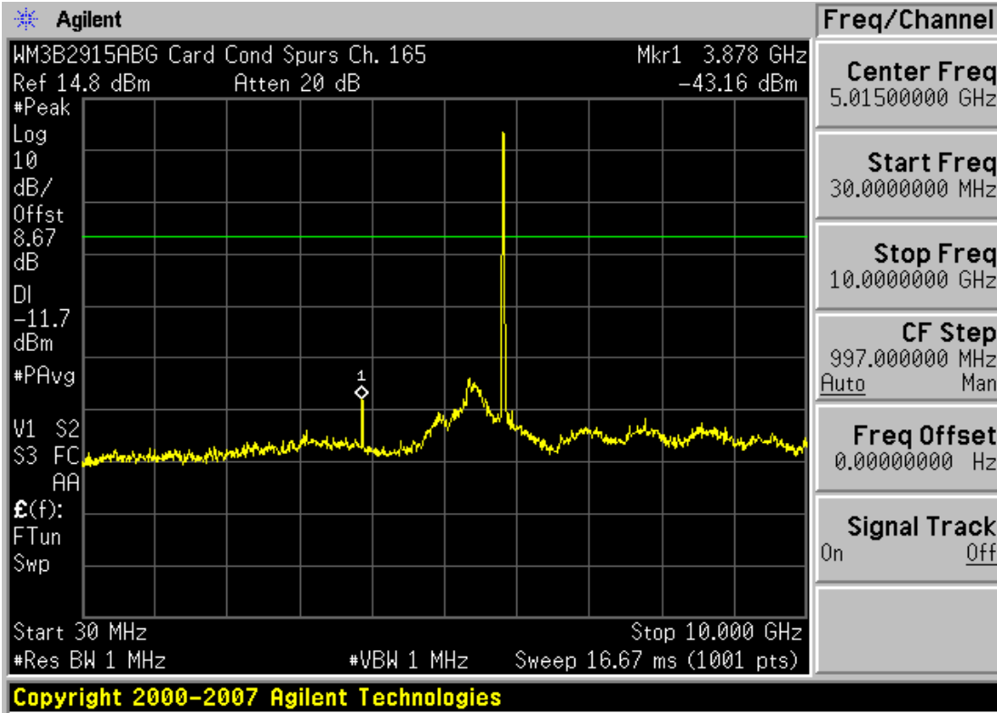
Plot 6-35. Conducted Spurious Plot (802.11a – Ch. 165)
