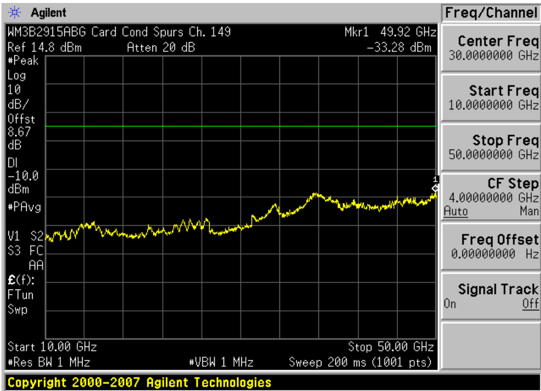
Plot 6-32. Conducted Spurious Plot (802.11a – Ch. 149)
