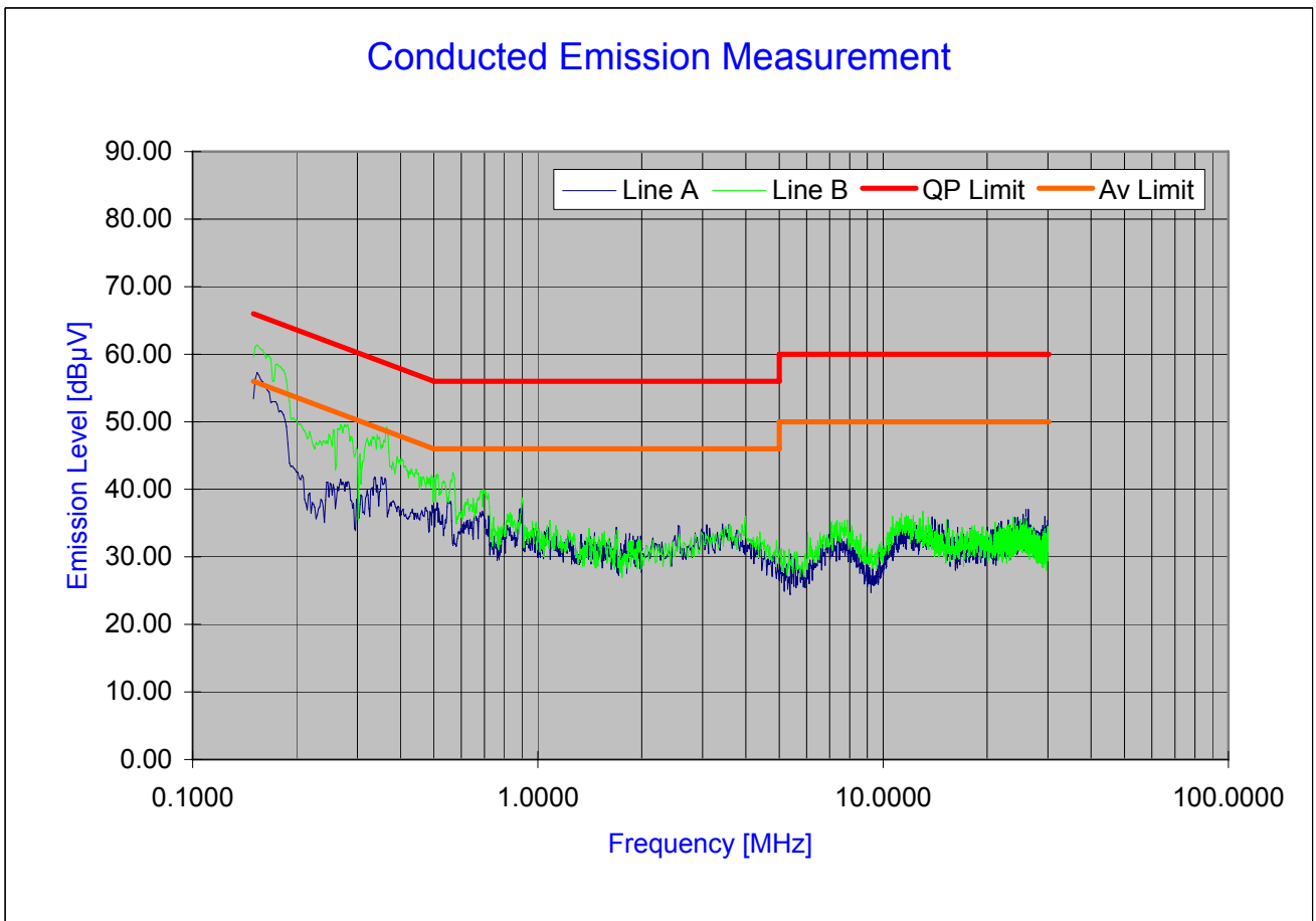
Plot 6-38. Line Conducted Plot with 802.11g
