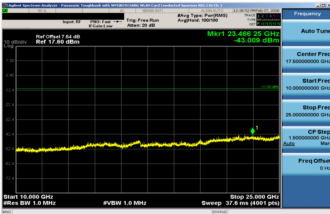
Plot 6-26. Conducted Spurious Plot (802.11b – Ch. 1)
