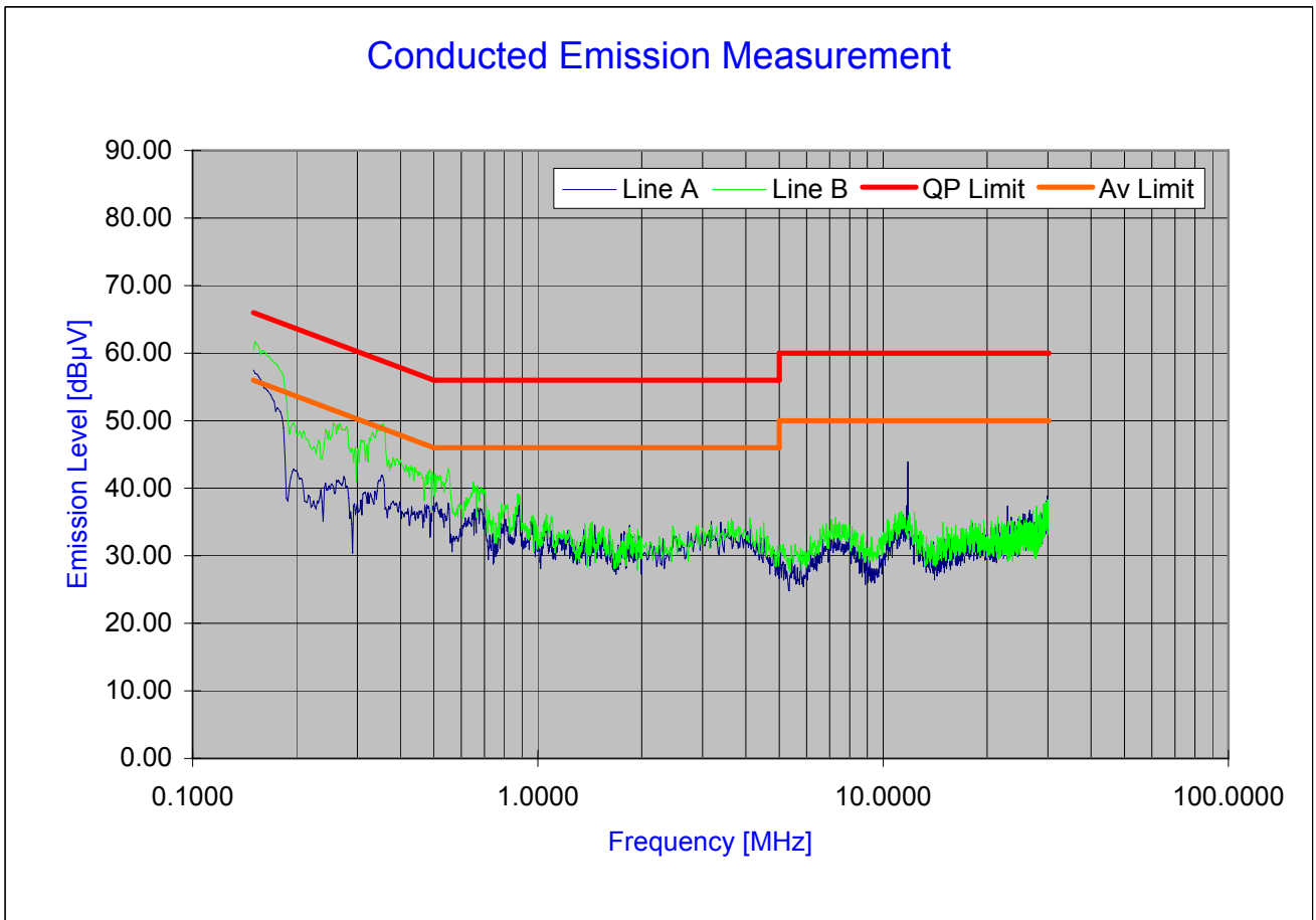
Plot 6-37. Line Conducted Plot with 802.11b
