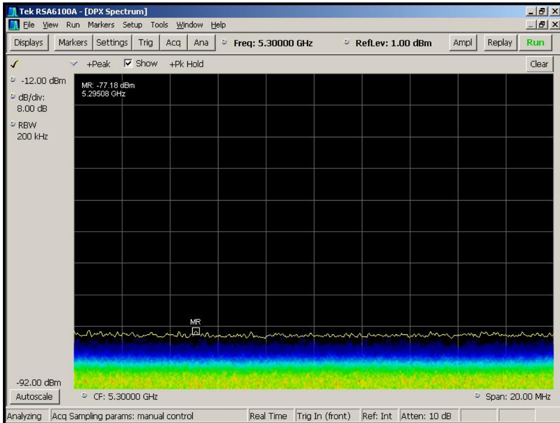
Figure 5-9 Non-occupancy Period after startup - 30min
