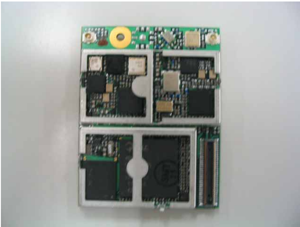
EM5625D Module Interior Bottom View
