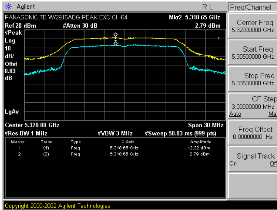
Plot A-17. Peak Excursion Ratio Plot – Ch. 64
