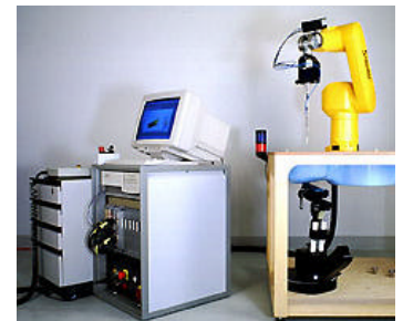
Fig. 1 SAR Test Setup
