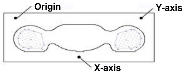
Fig 10. SAR Measurement Points in Area Scan Notebook PC w/ GSM PCS Module Panasonic FCC ID: ACJ9TGCF-27GSM
