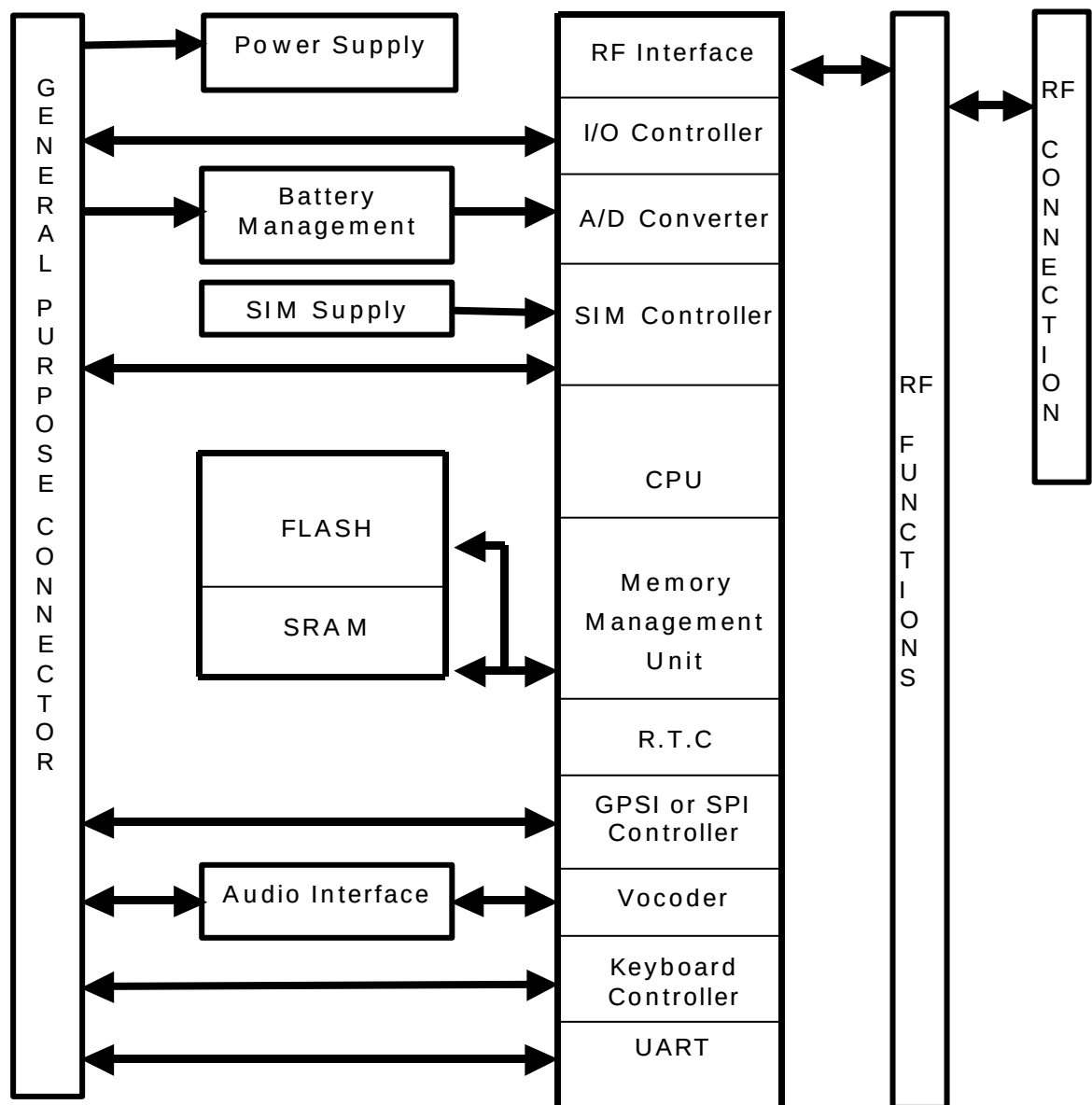
Figure 1 : Functional architecture
