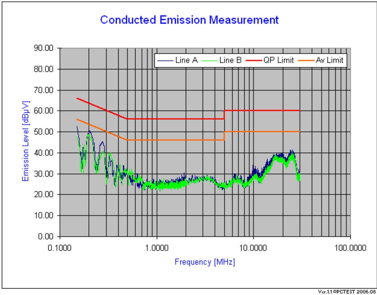
Plot 6-42. Line Conducted Plot with 802.11a (UNII Band III)
