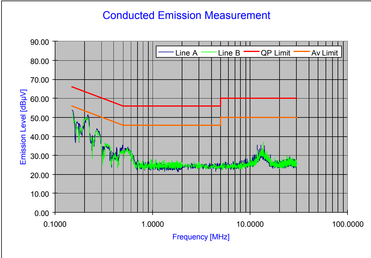
Plot 6-34. Line Conducted Plot with 802.11a (UNII Band I)
