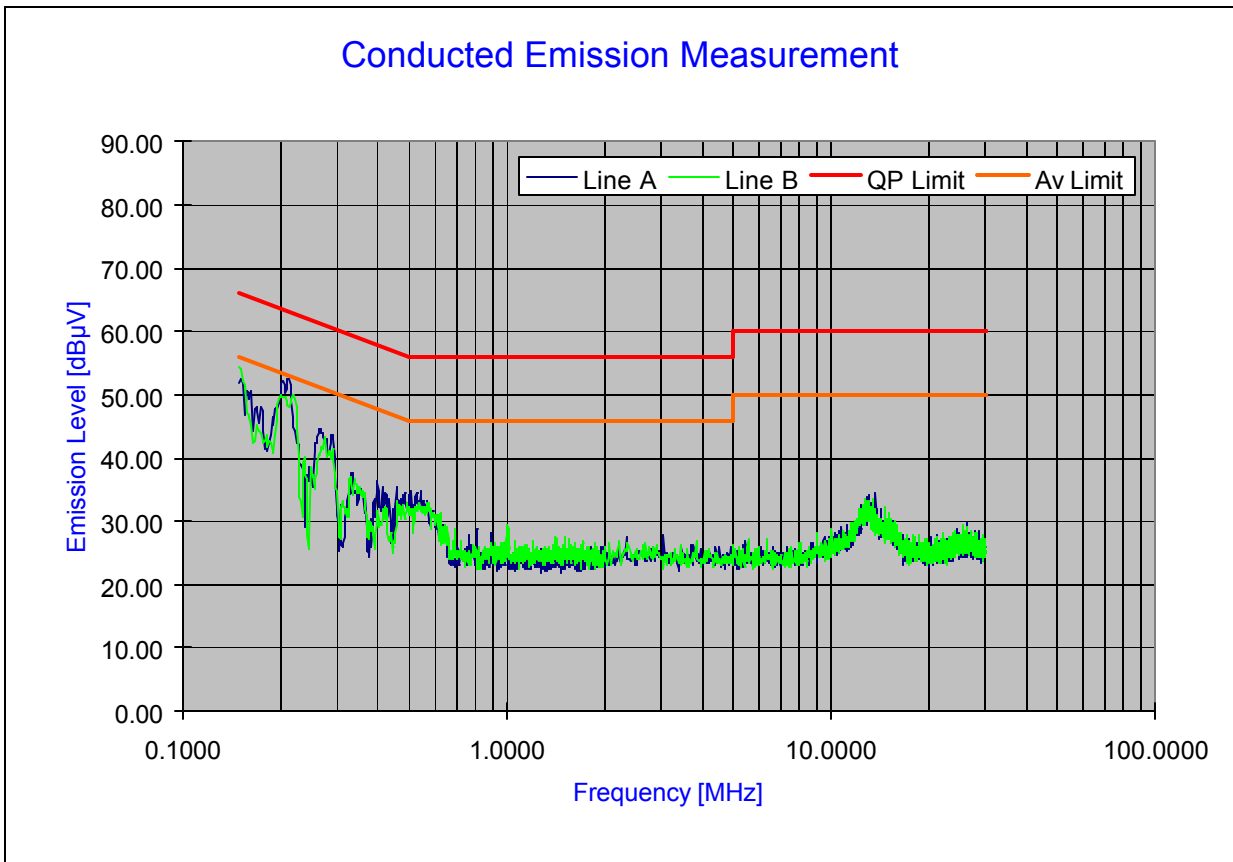
Plot 6-35. Line Conducted Plot with 802.11a (UNII Band II)
