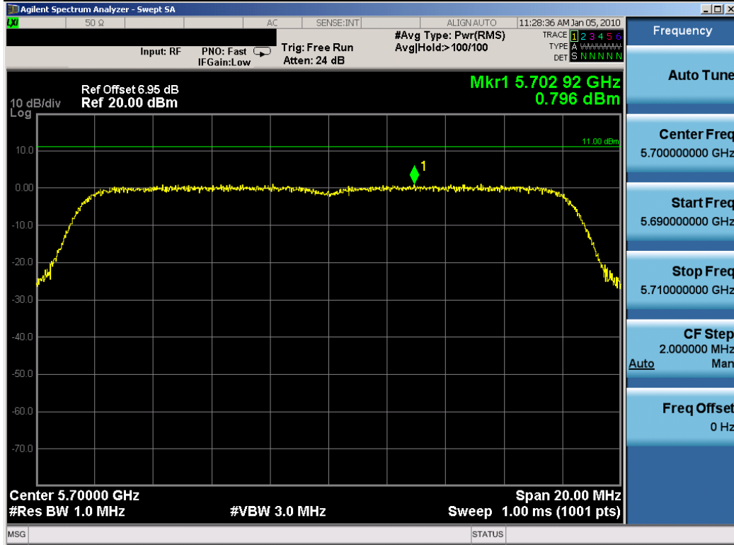
Plot 6-17. Peak Power Spectral Density Plot for UNII-Band3 (802.11a – Ch. 140) – Chain A
