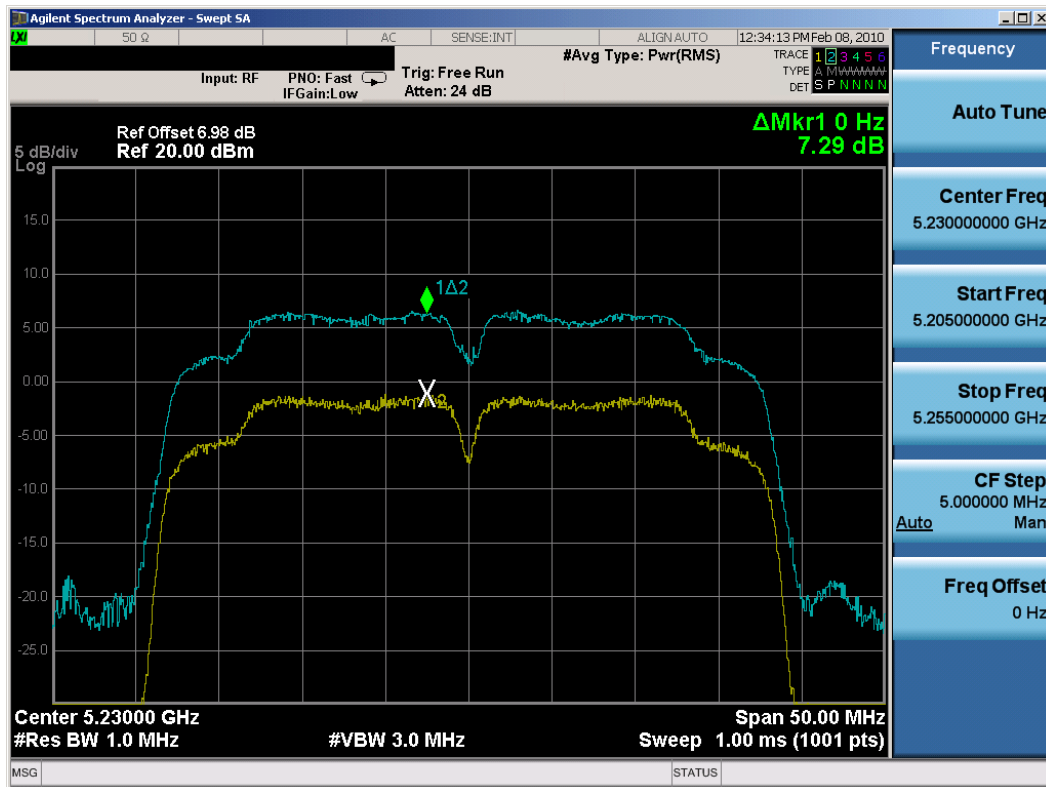
Plot 6-31. Peak Excursion Ratio Plot (802.11n (UNII) – Ch. 46) – Chain B
