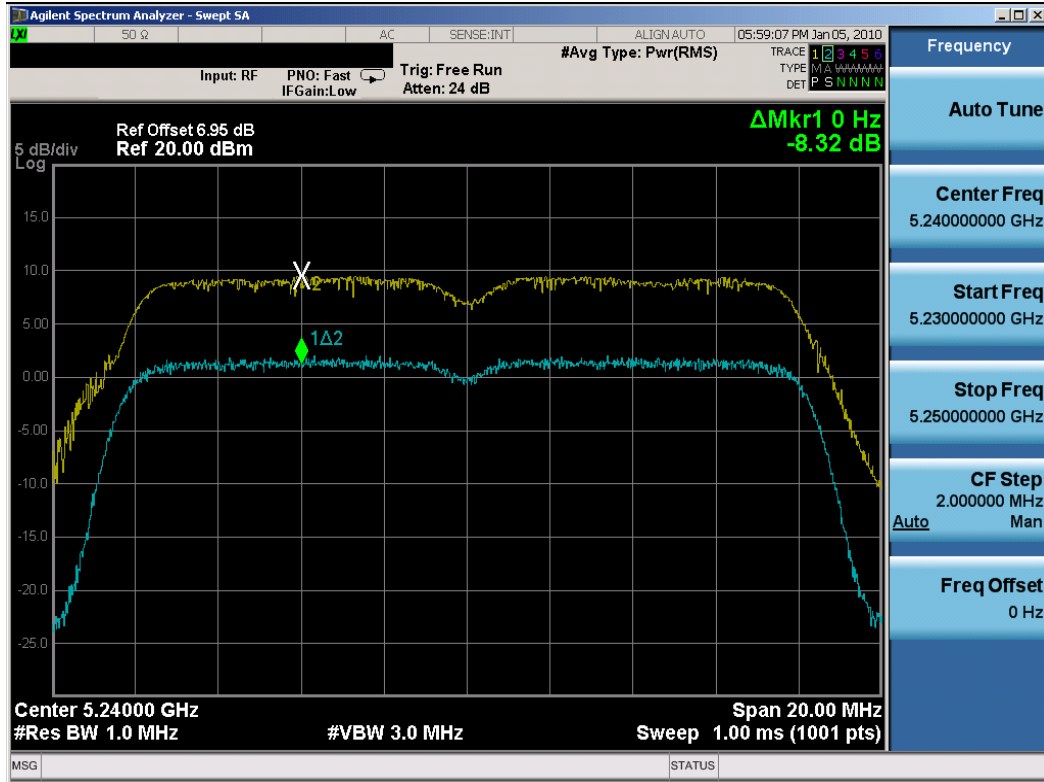
Plot 6-22. Peak Excursion Ratio Plot (802.11a (UNII) – Ch. 48) – Chain A
