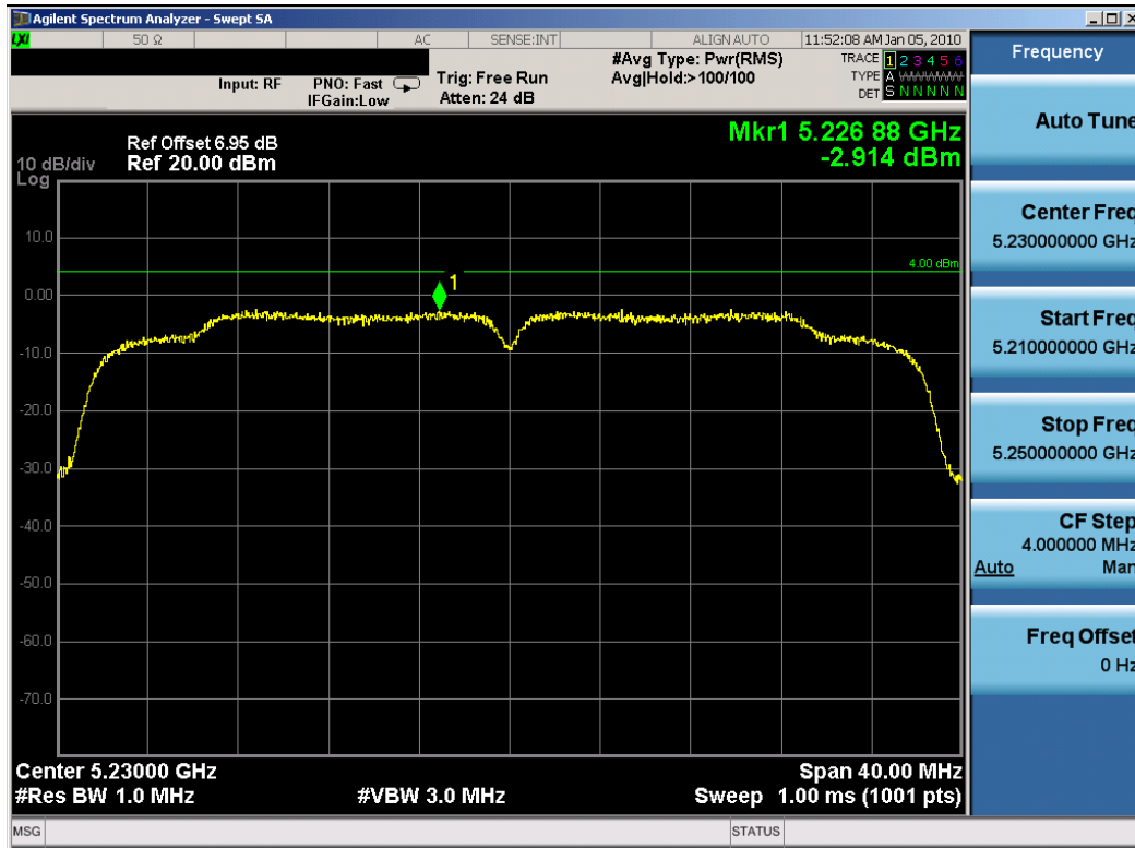
Plot 6-14. Peak Power Spectral Density Plot for UNII-Band1 (802.11n – Ch. 46) – Chain A
