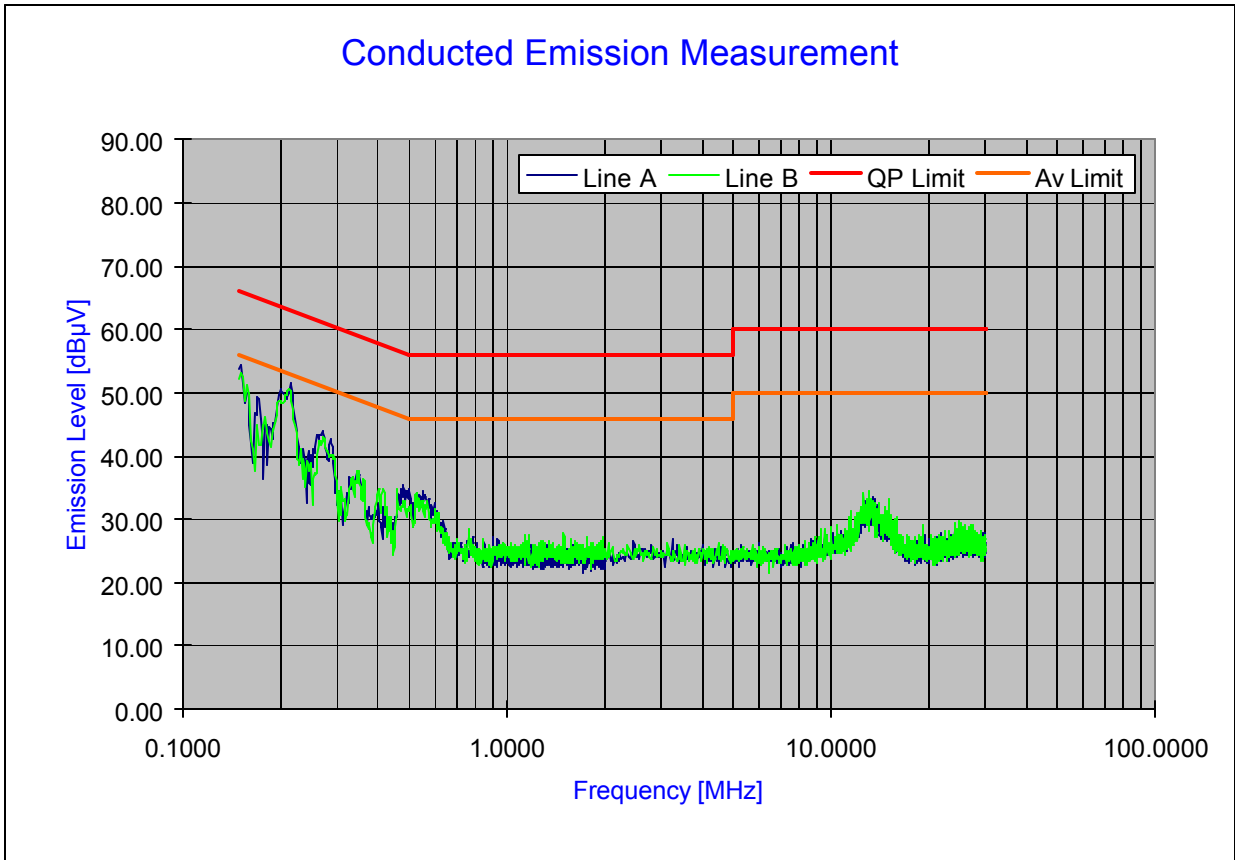
Plot 6-37. Line Conducted Plot with 802.11n (UNII Band I)
