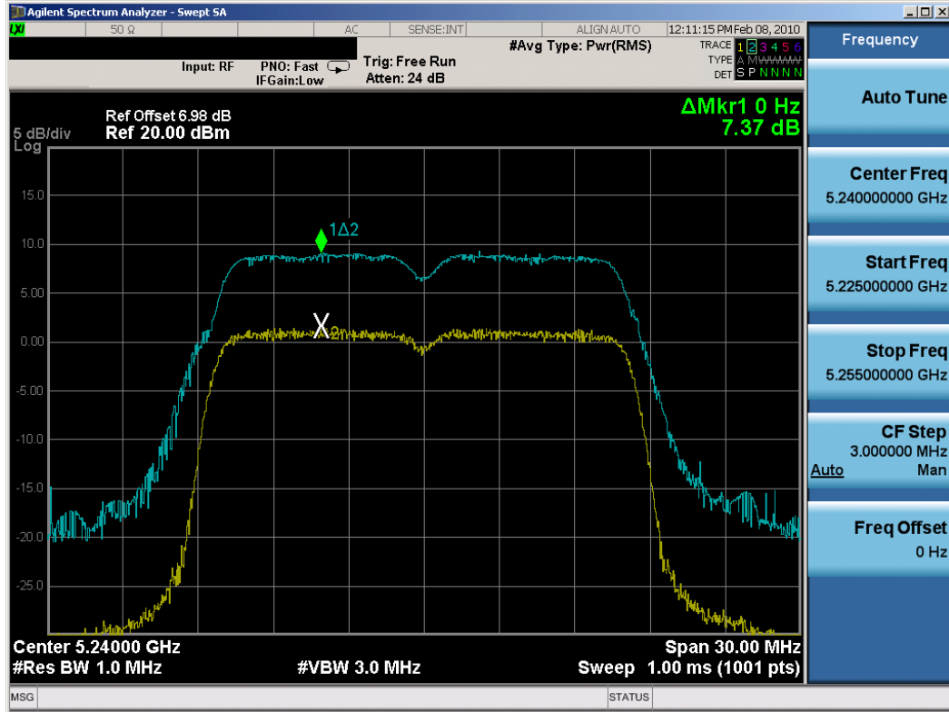
Plot 6-28. Peak Excursion Ratio Plot (802.11a (UNII) - Ch. 48) - Chain B
