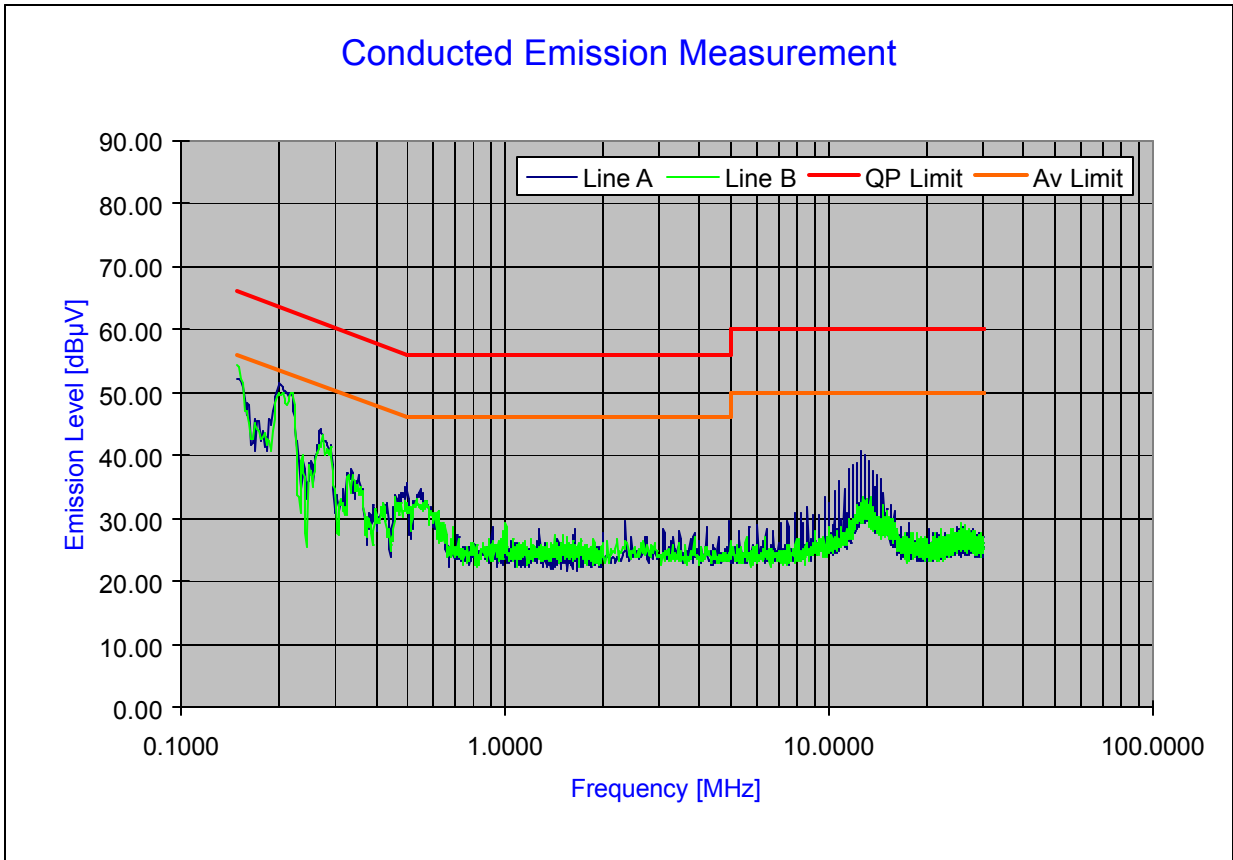
Plot 6-39. Line Conducted Plot with 802.11n (UNII Band III)
