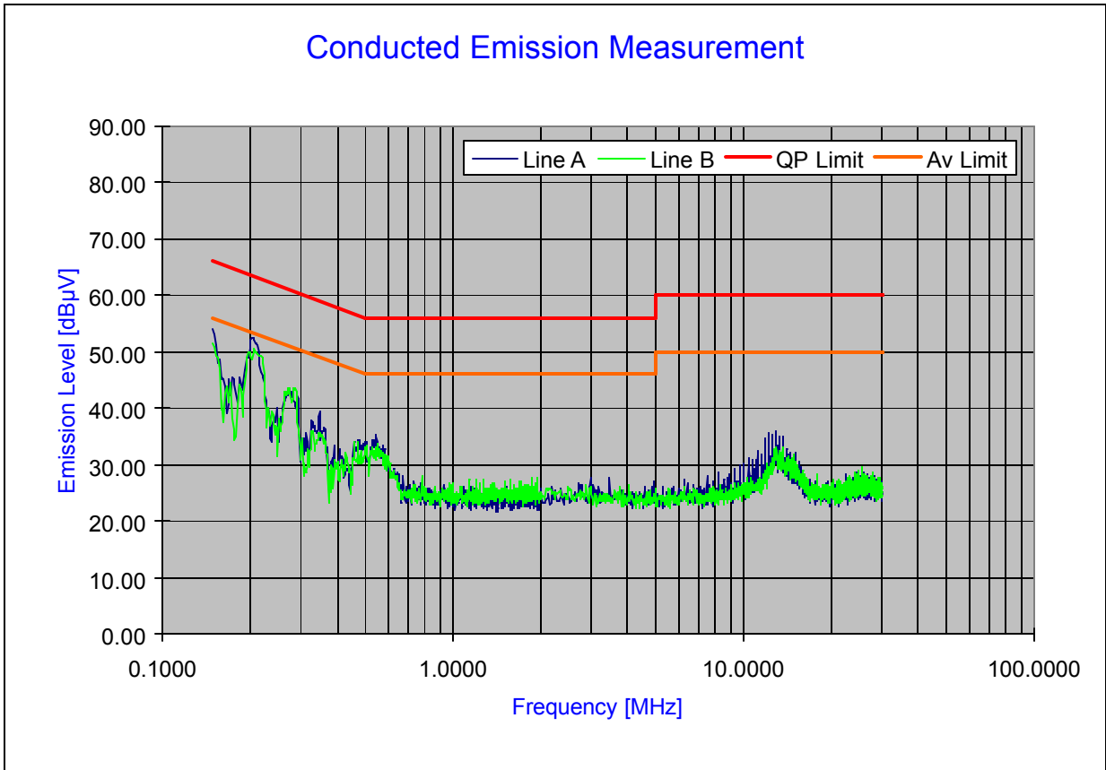
Plot 6-38. Line Conducted Plot with 802.11n (UNII Band II)
