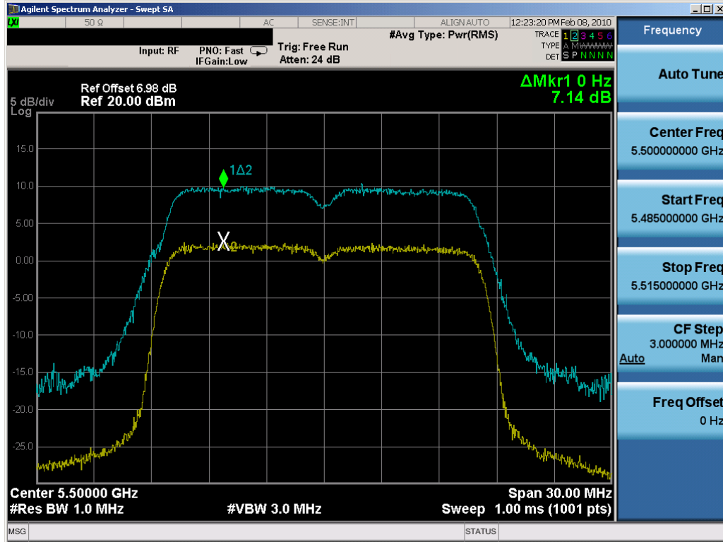
Plot 6-30. Peak Excursion Ratio Plot (802.11a (UNII) – Ch. 100) – Chain B
