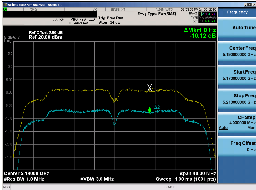
Plot 6-25. Peak Excursion Ratio Plot (802.11n (UNII) – Ch. 38) – Chain A
