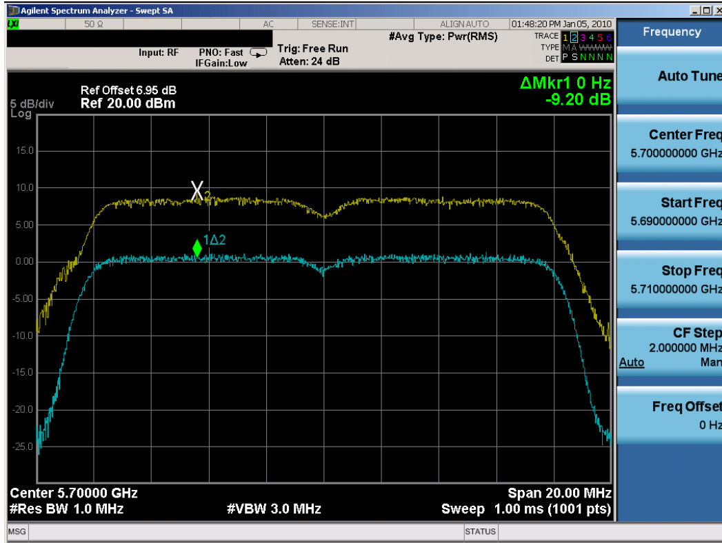
Plot 6-24. Peak Excursion Ratio Plot (802.11a (UNII) – Ch. 140) – Chain A
