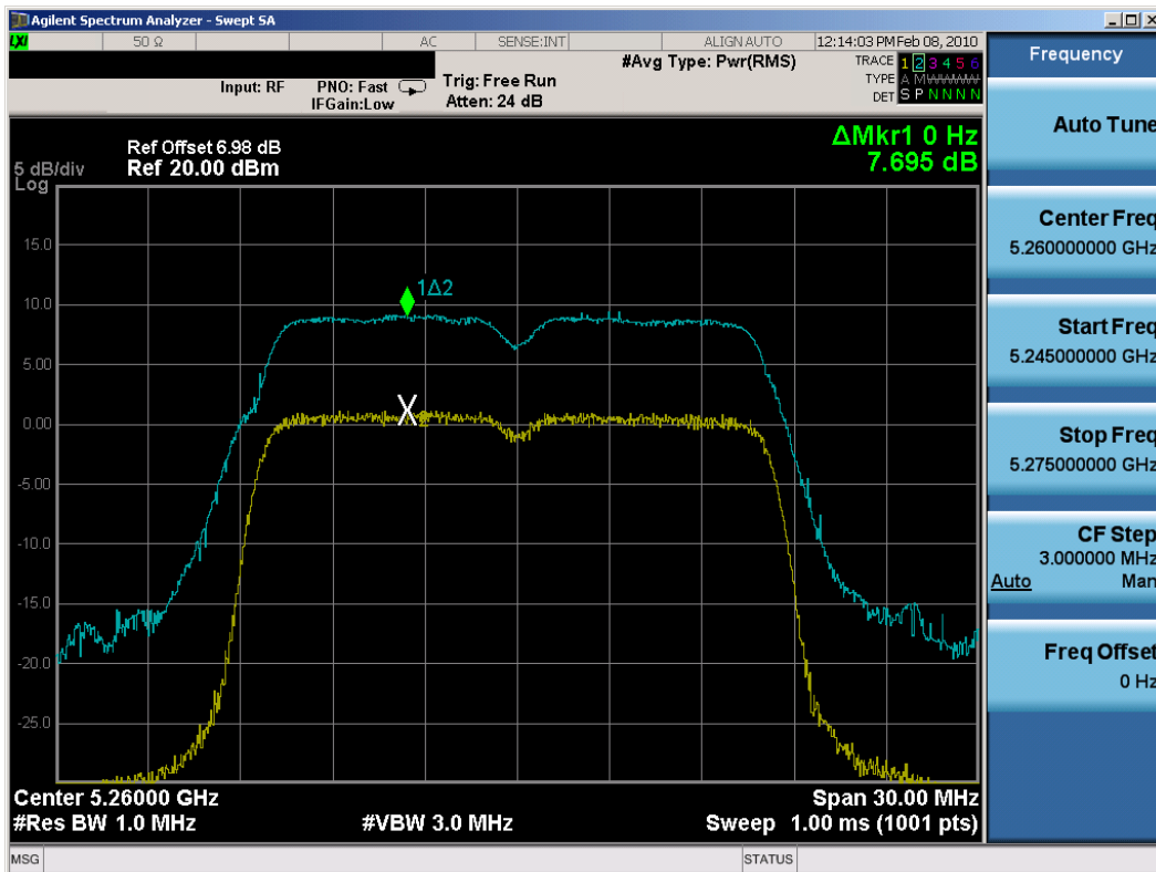
Plot 6-29. Peak Excursion Ratio Plot (802.11a (UNII) - Ch. 52) - Chain B
