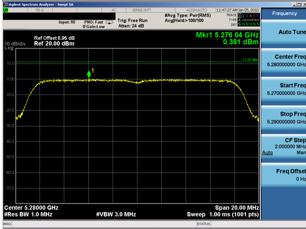
Plot 6-15. Peak Power Spectral Density Plot for UNII-Band2 (802.11a – Ch. 56) – Chain A
