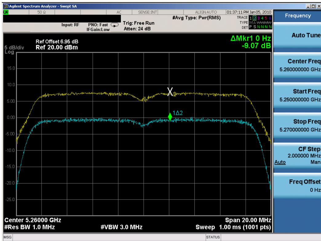
Plot 6-23. Peak Excursion Ratio Plot (802.11a (UNII) – Ch. 52) – Chain A
