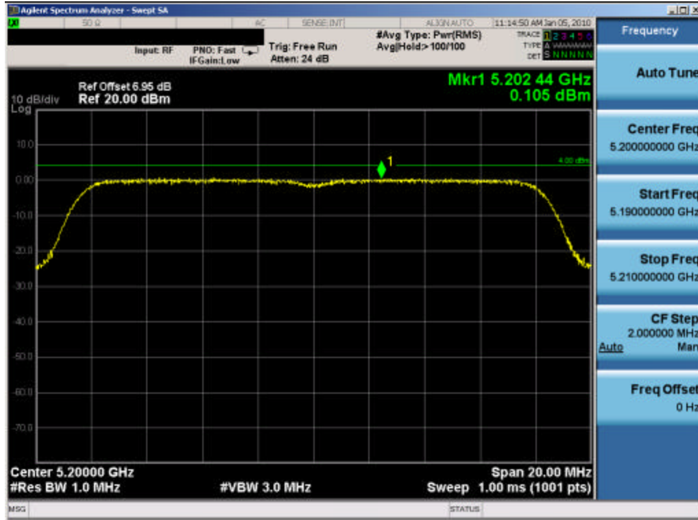
Plot 6-13. Peak Power Spectral Density Plot for UNII-Band1 (802.11a – Ch. 40) – Chain A
