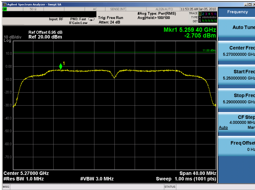
Plot 6-16. Peak Power Spectral Density Plot for UNII-Band2 (802.11n – Ch. 54) – Chain A
