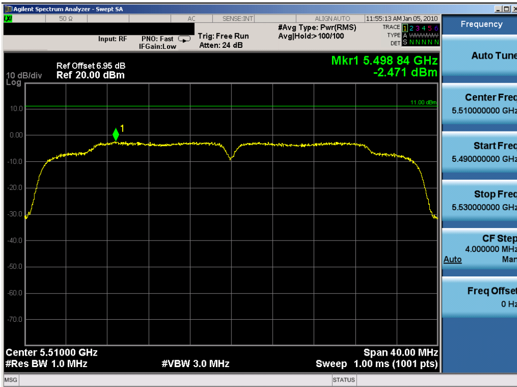
Plot 6-18. Peak Power Spectral Density Plot for UNII-Band3 (802.11n – Ch. 102) – Chain A
