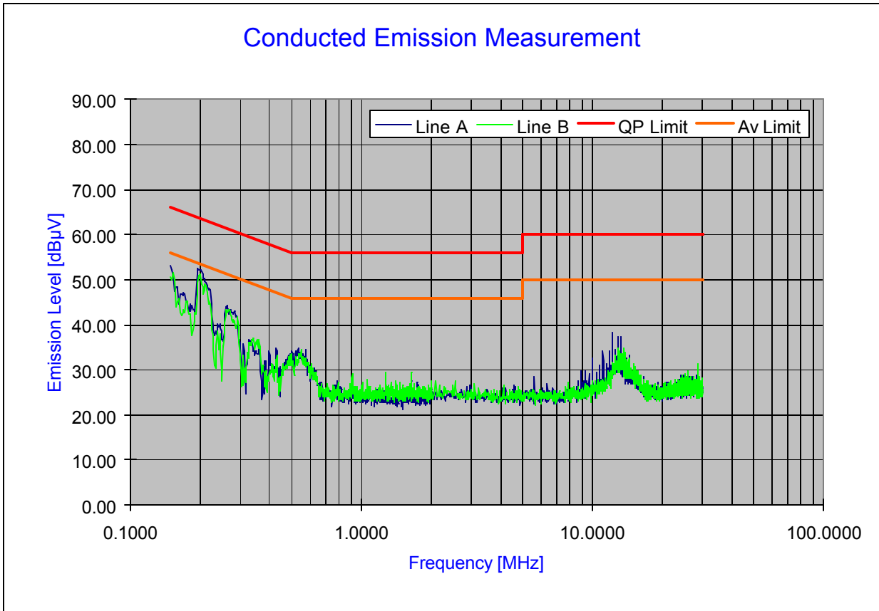
Plot 6-36. Line Conducted Plot with 802.11a (UNII Band III)
