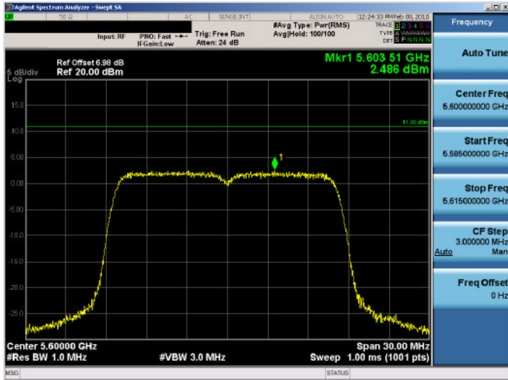
Plot 6-21. Maximum Peak Power Spectral Density Plot for UNII-Band3 (802.11a – Ch. 120) – Chain B
