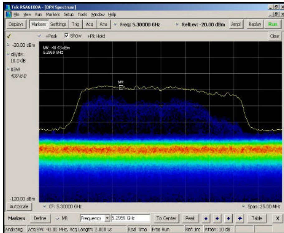
Figure 5-3. Real-Time Spectrum Display, No WLAN Traffic
