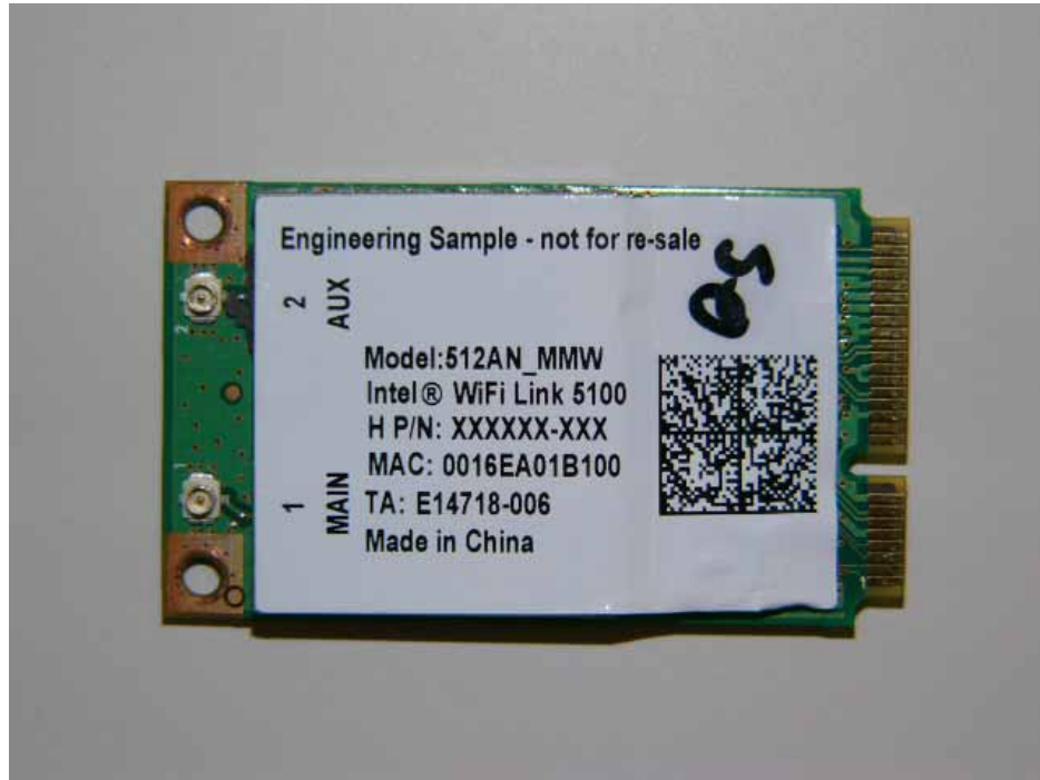
WLAN Exterior Top View
