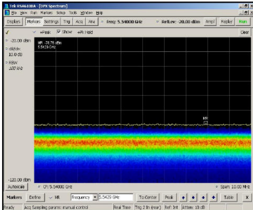
Figure 6-7 Non-occupancy Period - Monitoring live real time spectrum - Elapse time 30 minutes
