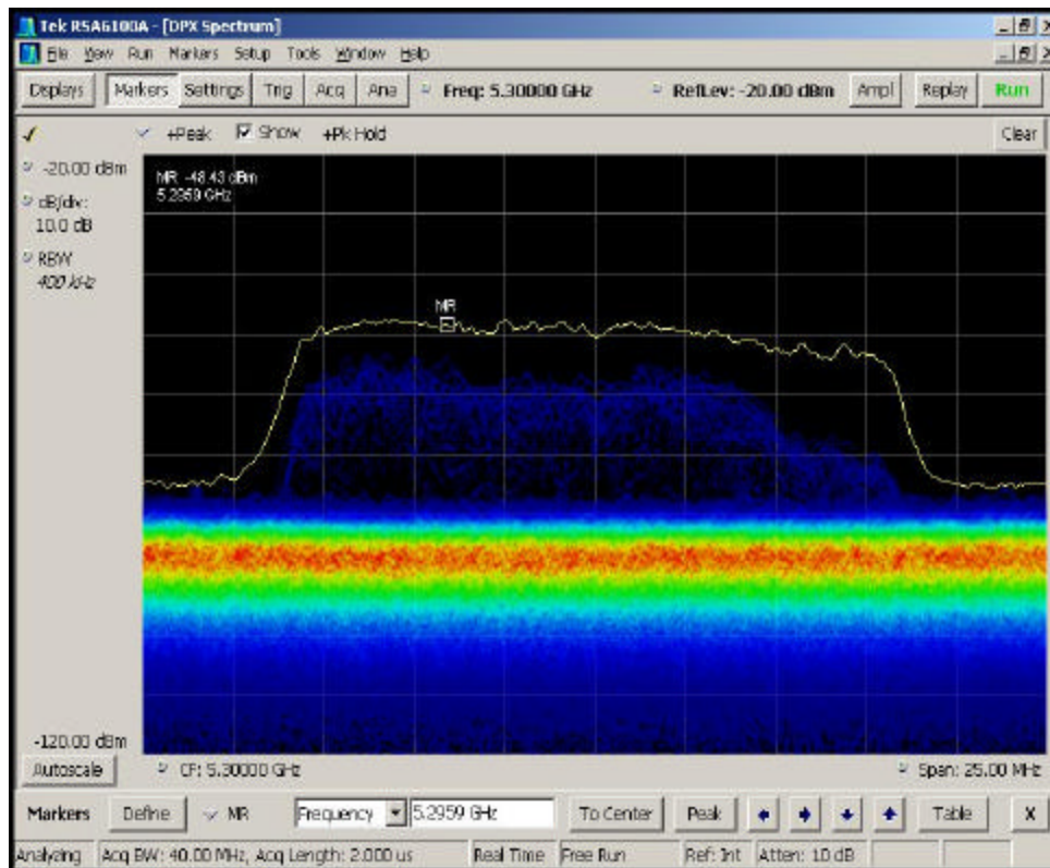
Figure 5-3. Real-Time Spectrum Display, No WLAN Traffic
