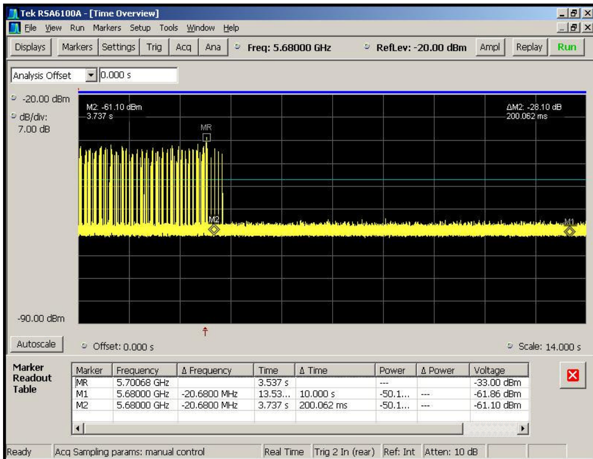
Figure 6-4. Channel Move Time (< 10sec)
