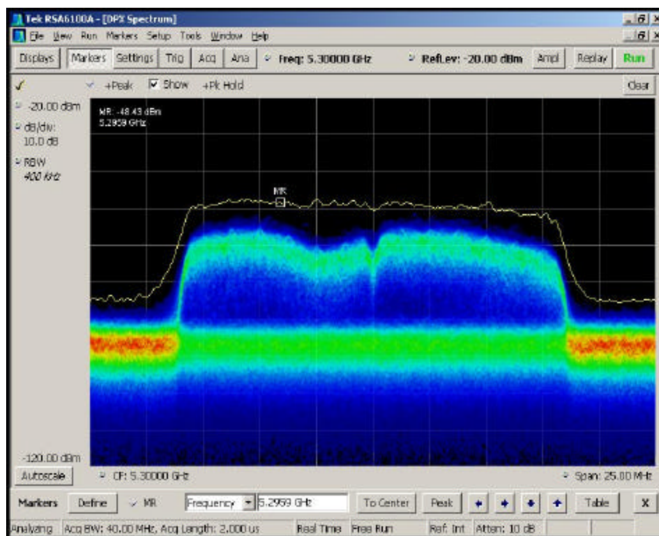
Figure 5-4. Real-Time Spectrum Display, WLAN Traffic (Streaming Video)
