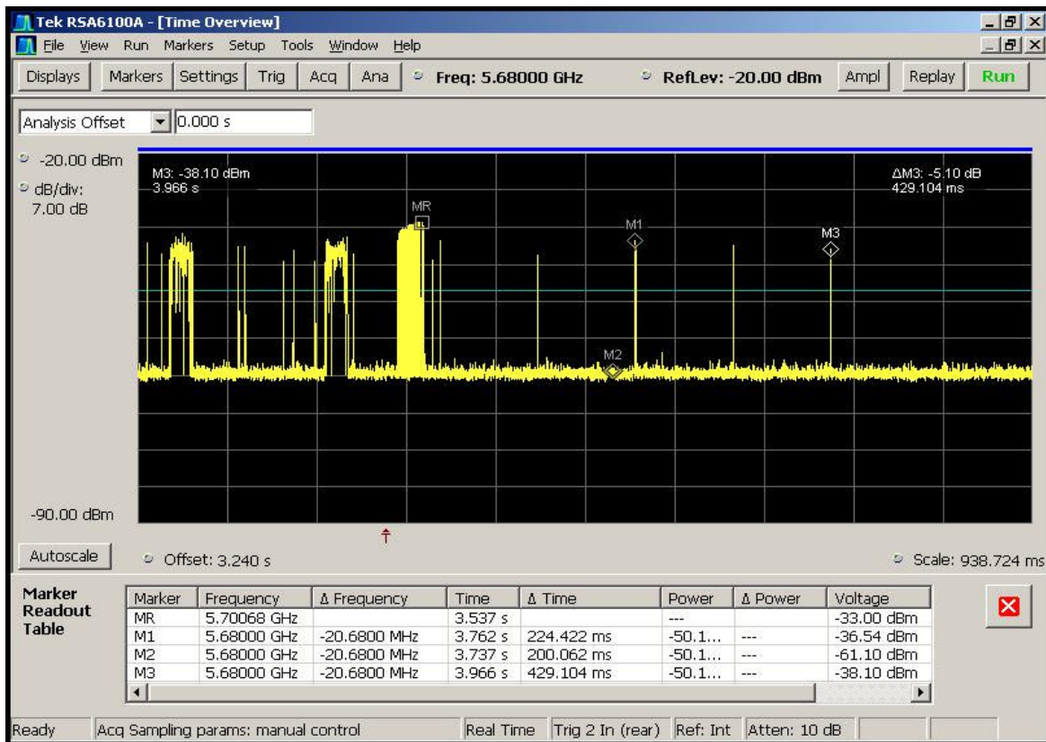
Figure 6-5. Channel Closing Transmission Time, Aggregate Time After 200ms
