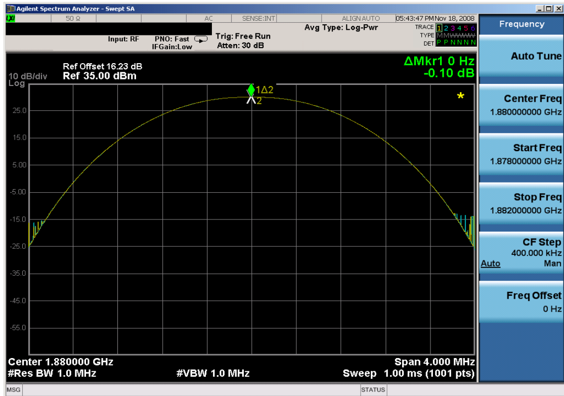
Plot 7-18. Peak-Average Ratio Plot (PCS EDGE Mode – Ch. 661)
