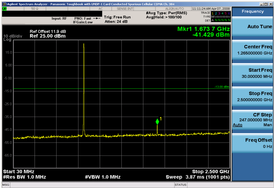
Plot 7-50. Conducted Spurious Plot (Cellular CDMA Mode – Ch. 384)
