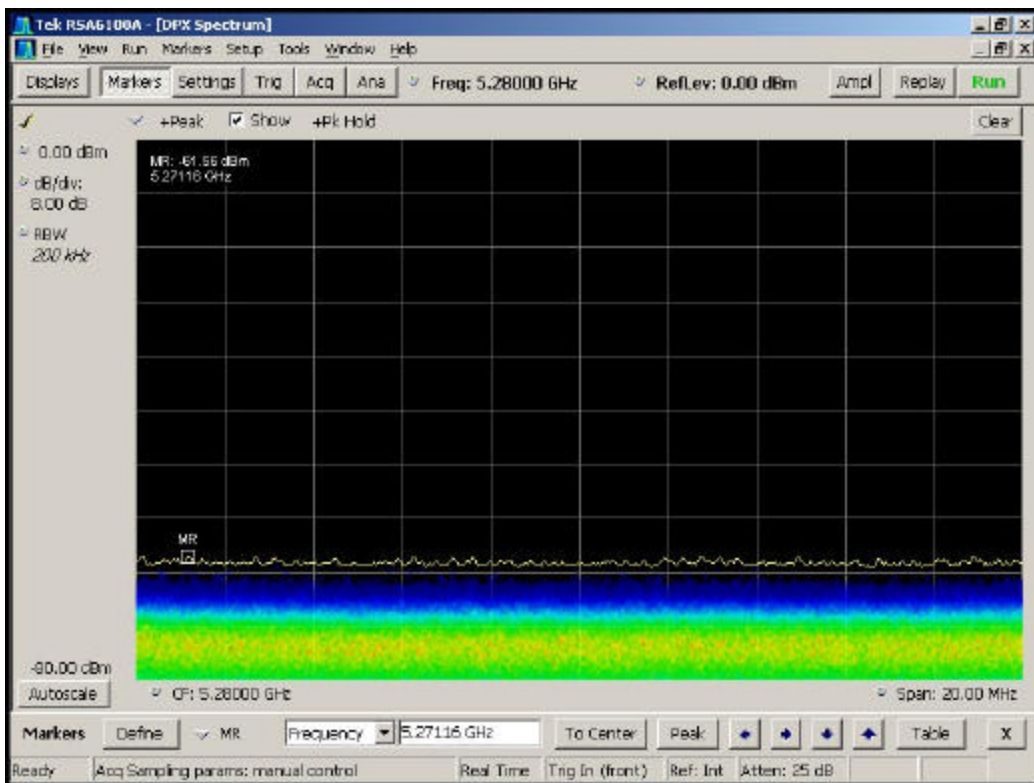
Figure 5-8 Non-occupancy Period – Monitoring live real time spectrum – elapsed time 30 minutes
