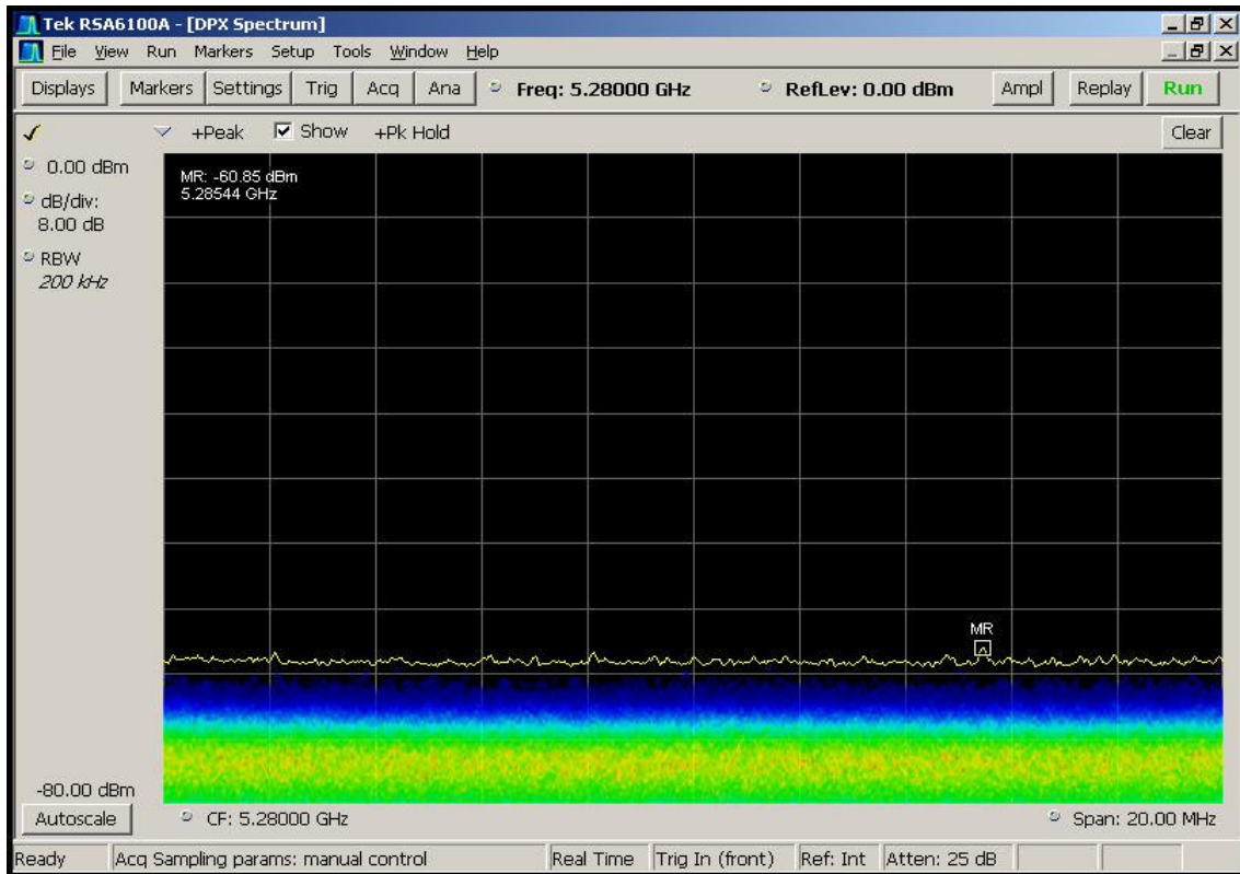
Figure 5-9 Non-occupancy Period After Startup – Monitoring live real time spectrum - elapsed time 30min
