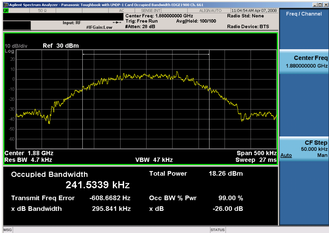
Plot 7-20. Occupied Bandwidth Plot (EDGE1900 Mode – Ch. 661)
