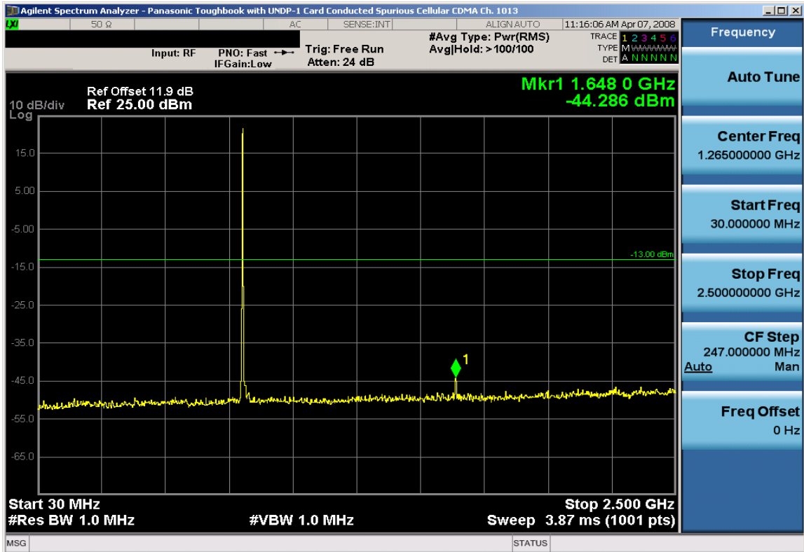
Plot 7-43. Conducted Spurious Plot (Cellular CDMA Mode – Ch. 1013)
