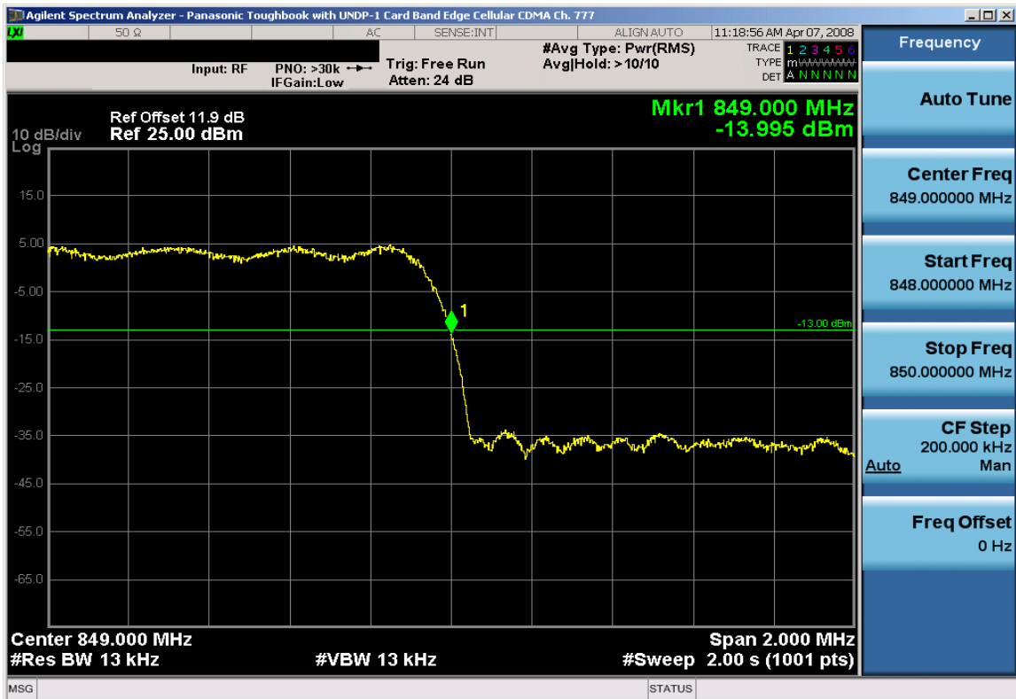
Plot 7-52. Band Edge Plot (Cellular CDMA Mode – Ch. 777)
