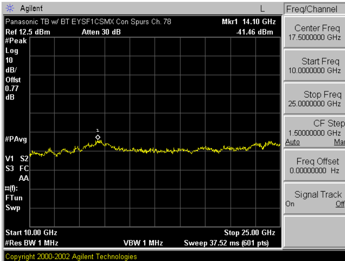
Plot 6-18. Conducted Spurious Plot (Bluetooth – Ch. 78)
