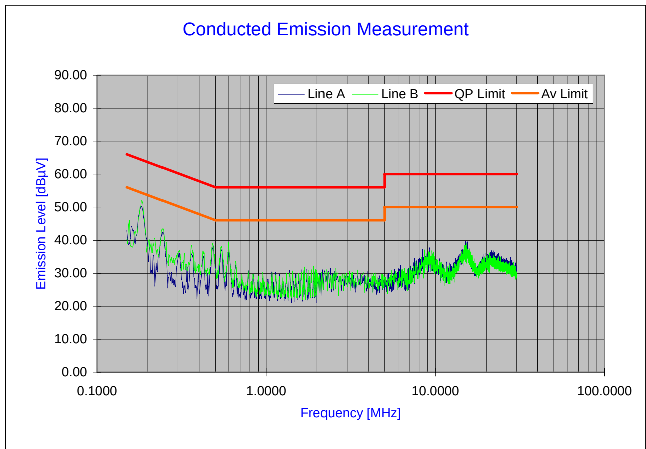
Plot 6-29. Line Conducted Plot with 802.11a
