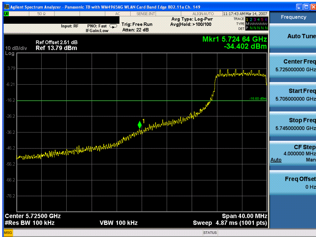
Plot 6-15. Band Edge Plot (802.11a – Ch. 149)
