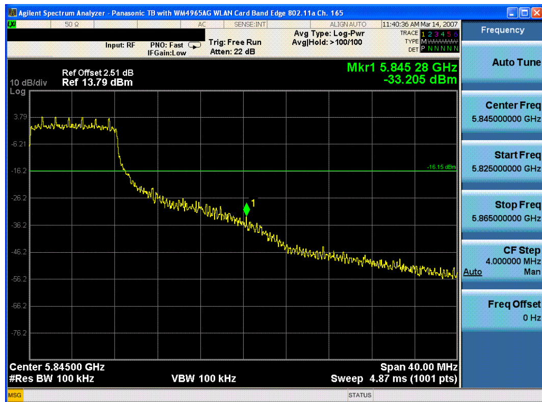
Plot 6-16. Band Edge Plot (802.11a – Ch. 165)
