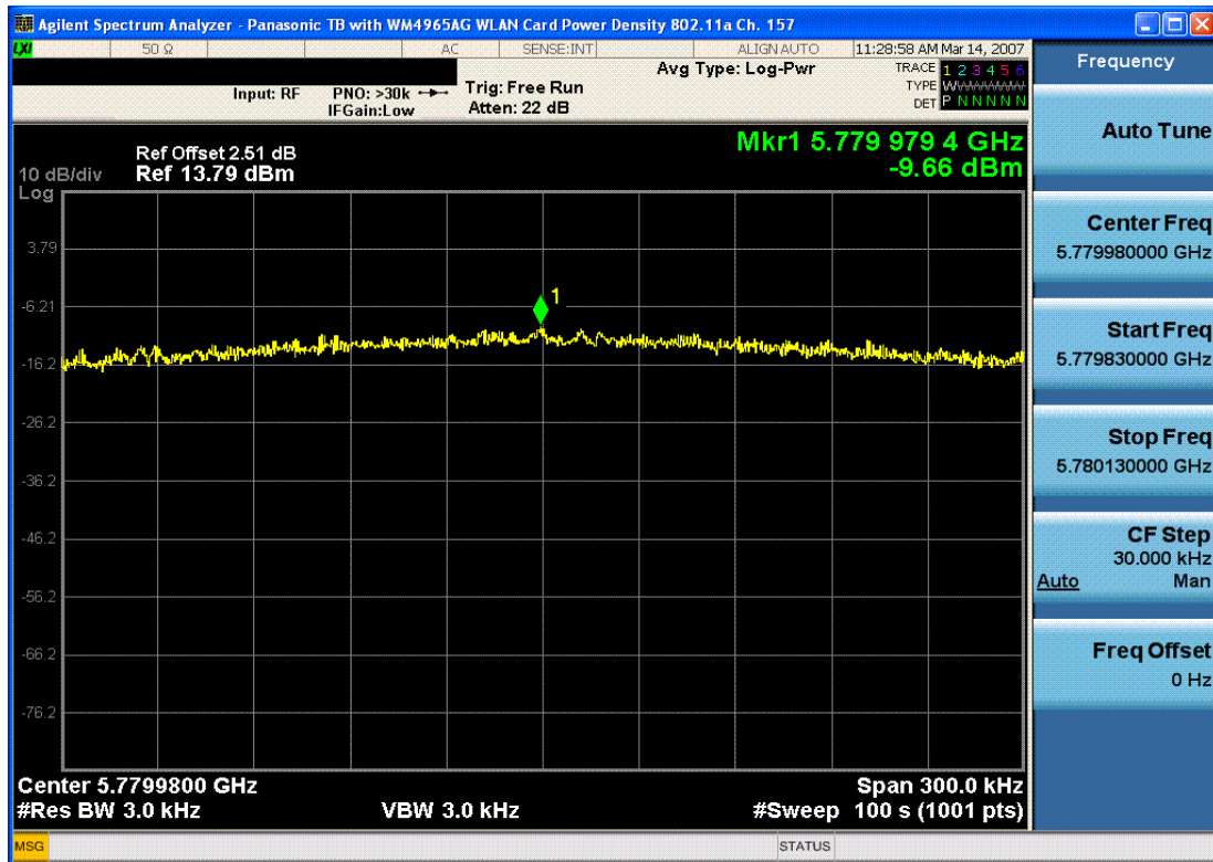
Plot 6-11. Power Spectral Density Plot (802.11a – Ch. 157)
