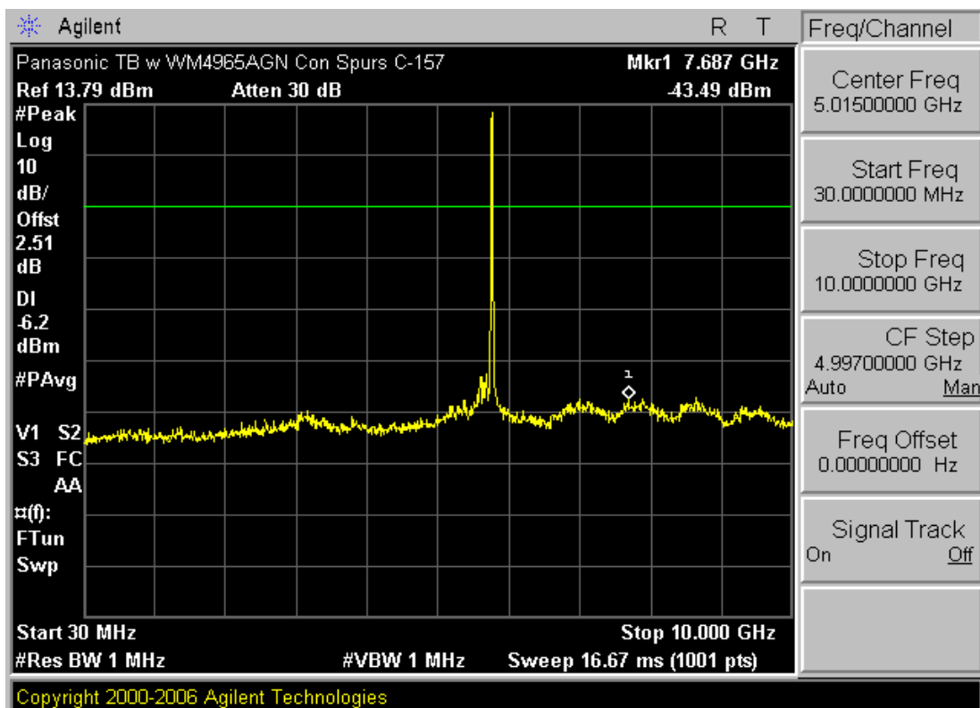
Plot 6-25. Conducted Spurious Plot (802.11a – Ch. 157)
