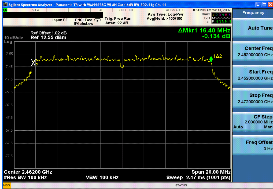
Plot 6-3. 6dB Bandwidth Plot (802.11g – Ch. 11)
