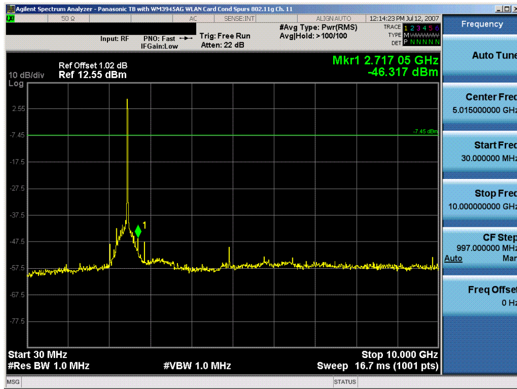
Plot 6-21. Conducted Spurious Plot (802.11g – Ch. 11)
