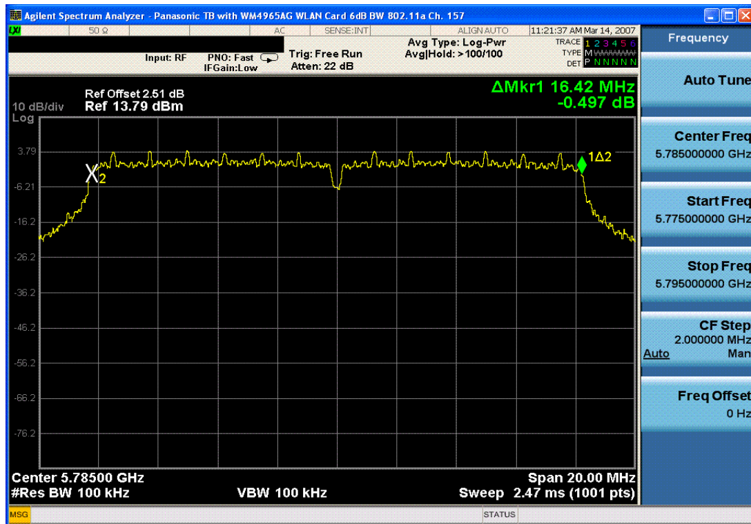
Plot 6-5. 6dB Bandwidth Plot (802.11a – Ch. 157)
