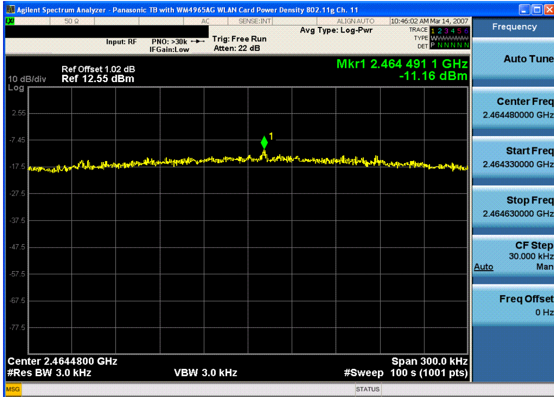
Plot 6-9. Power Spectral Density Plot (802.11g – Ch. 11)
