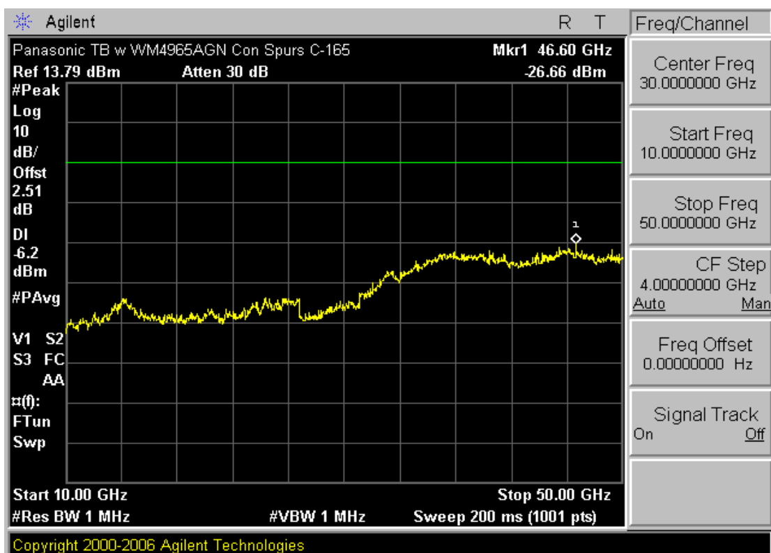
Plot 6-28. Conducted Spurious Plot (802.11a – Ch. 165)
