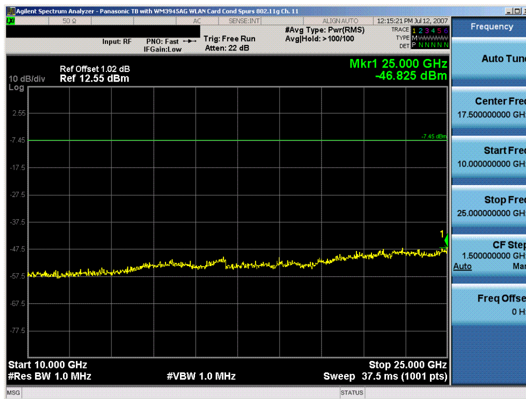
Plot 6-22. Conducted Spurious Plot (802.11g – Ch. 11)
