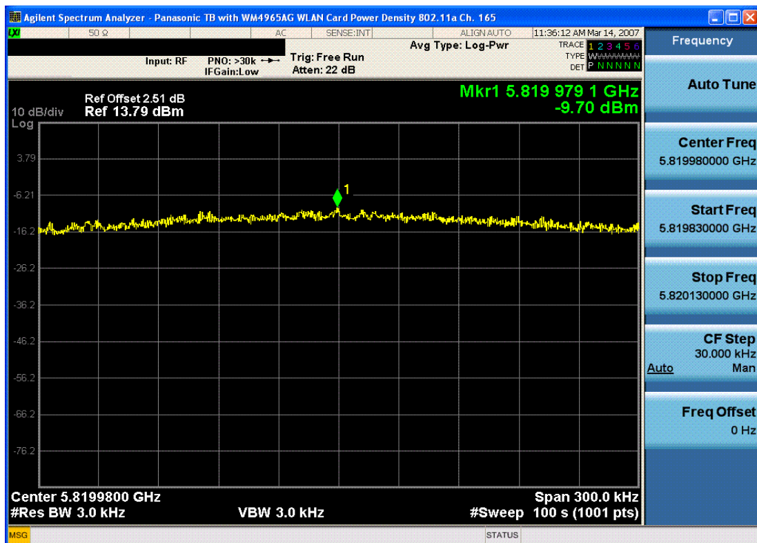
Plot 6-12. Power Spectral Density Plot (802.11a – Ch. 165)
