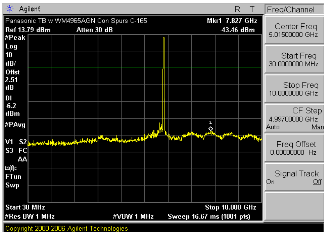
Plot 6-27. Conducted Spurious Plot (802.11a – Ch. 165)
