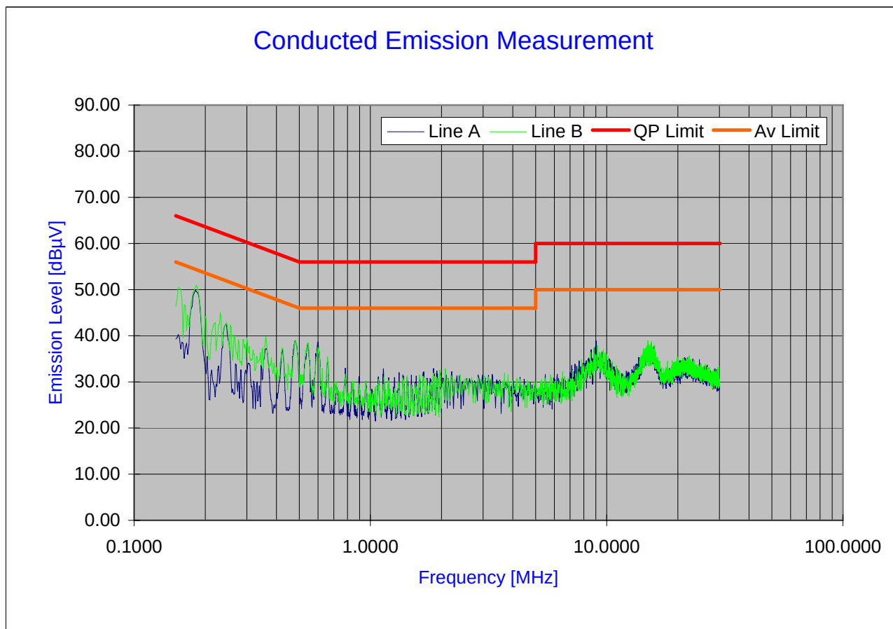
Plot 6-30. Line Conducted Plot with 802.11g
