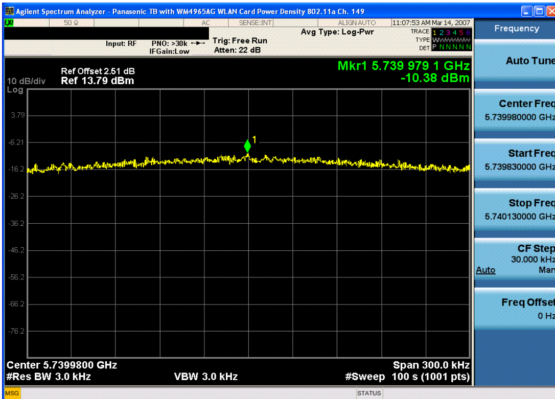
Plot 6-10. Power Spectral Density Plot (802.11a – Ch. 149)
