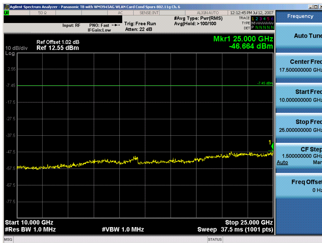
Plot 6-20. Conducted Spurious Plot (802.11g – Ch. 6)
