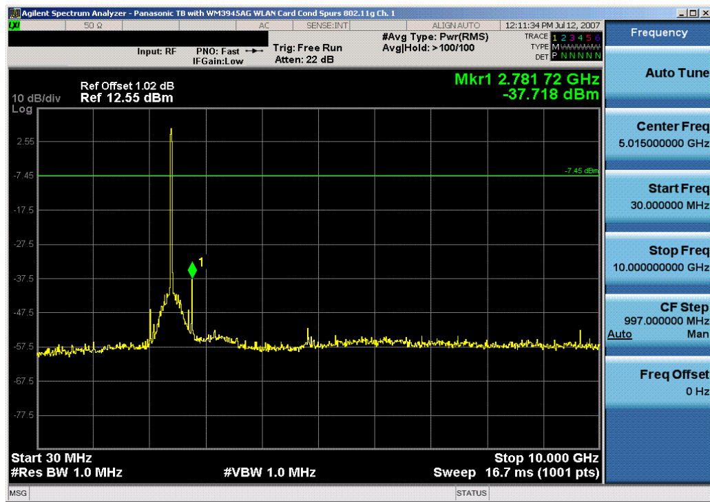
Plot 6-17. Conducted Spurious Plot (802.11g – Ch. 1)
