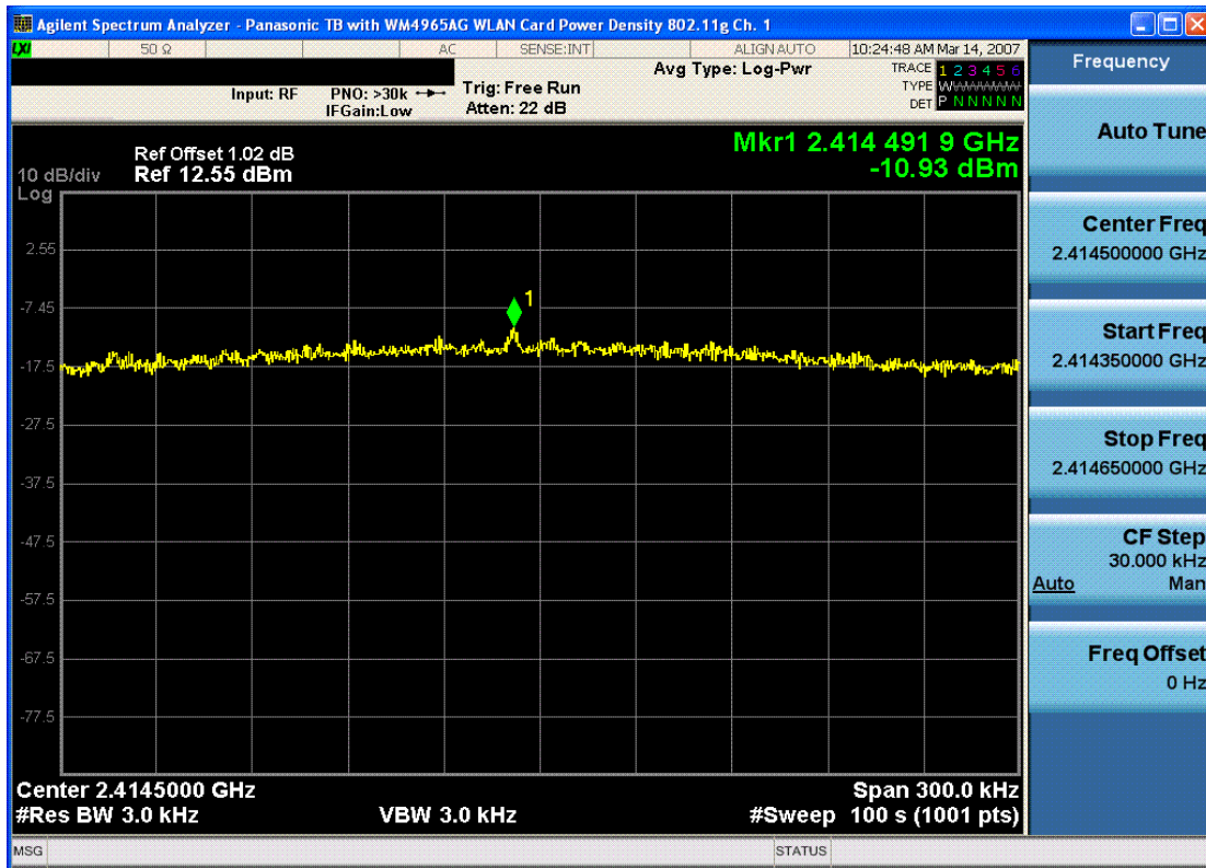
Plot 6-7. Power Spectral Density Plot (802.11g – Ch. 1)
