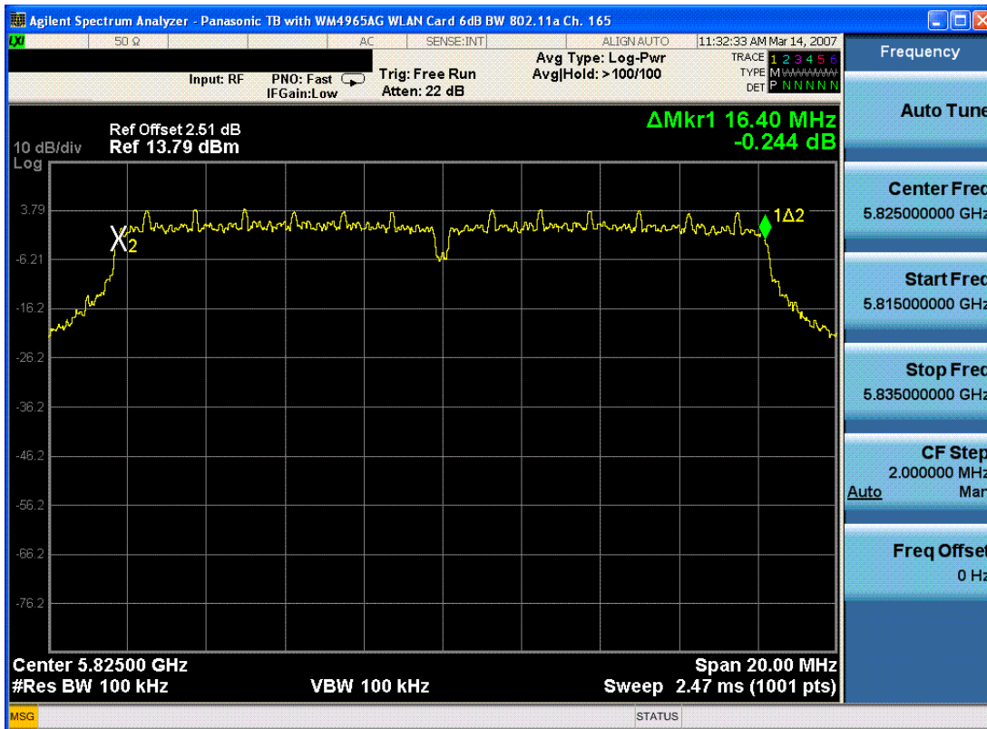
Plot 6-6. 6dB Bandwidth Plot (802.11a – Ch. 165)
