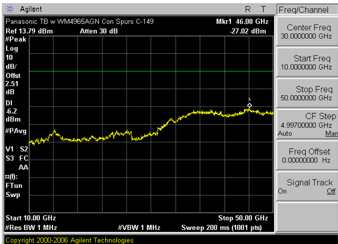
Plot 6-24. Conducted Spurious Plot (802.11a – Ch. 149)
