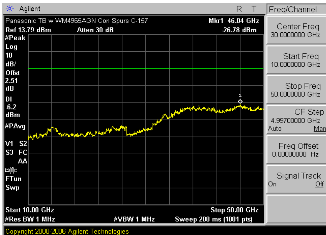
Plot 6-26. Conducted Spurious Plot (802.11a – Ch. 157)
