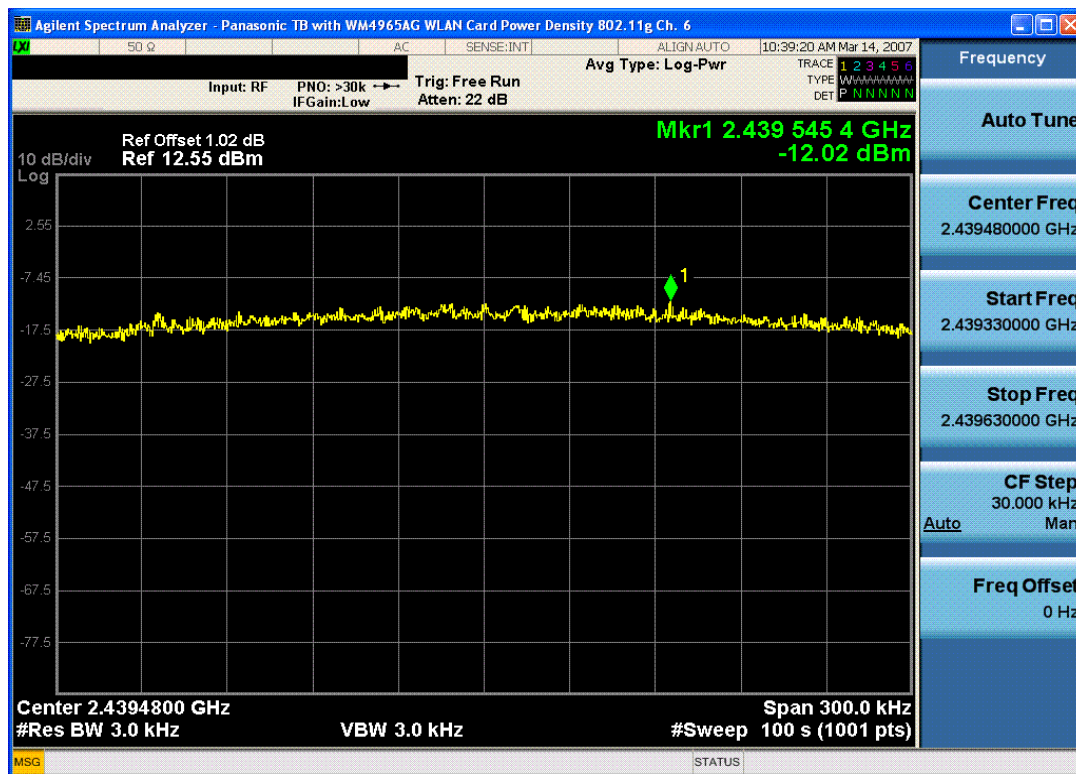
Plot 6-8. Power Spectral Density Plot (802.11g – Ch. 6)
