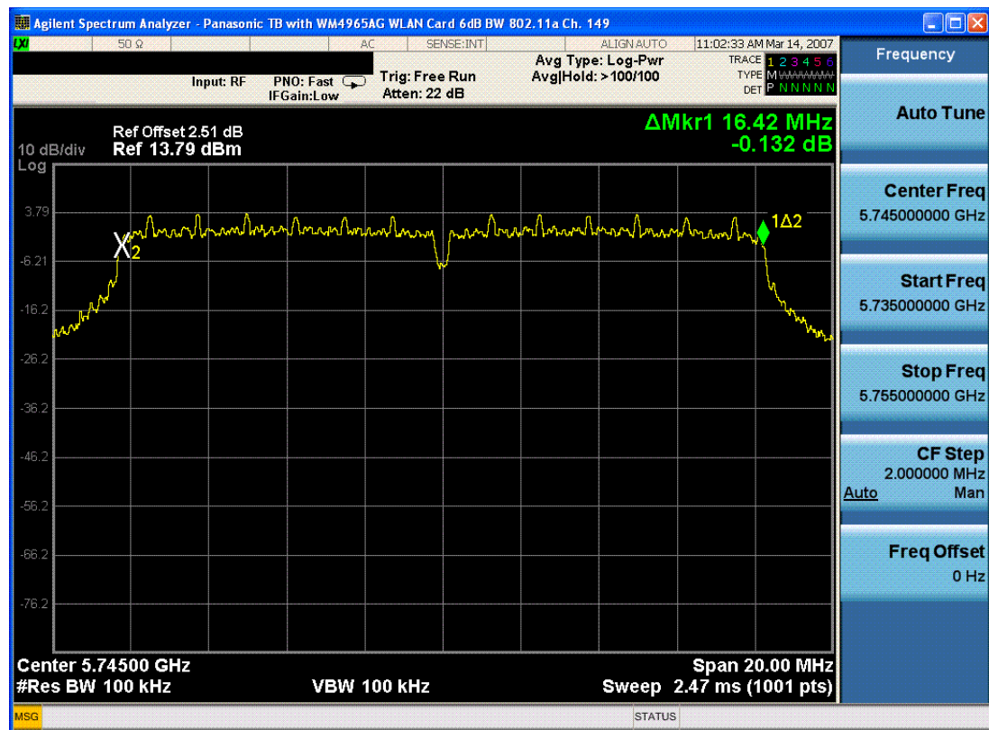
Plot 6-4. 6dB Bandwidth Plot (802.11a – Ch. 149)
