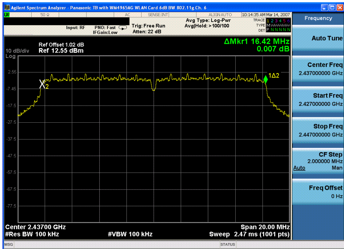
Plot 6-2. 6dB Bandwidth Plot (802.11g – Ch. 6)
