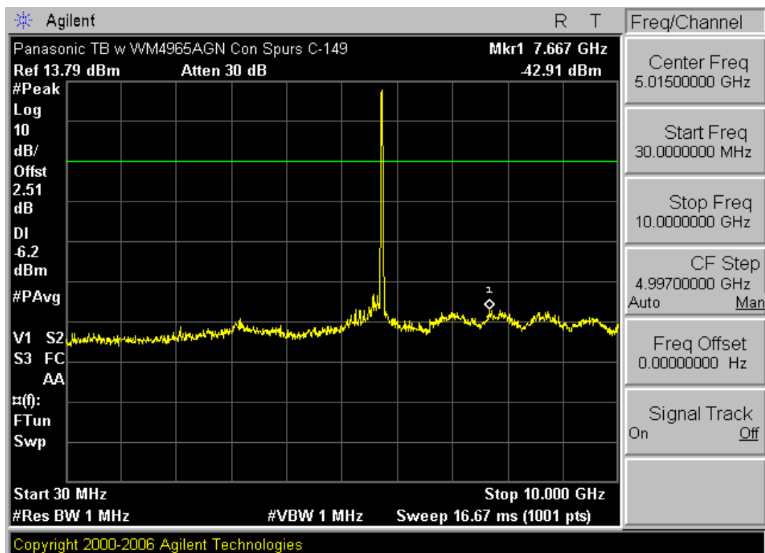
Plot 6-23. Conducted Spurious Plot (802.11a – Ch. 149)
