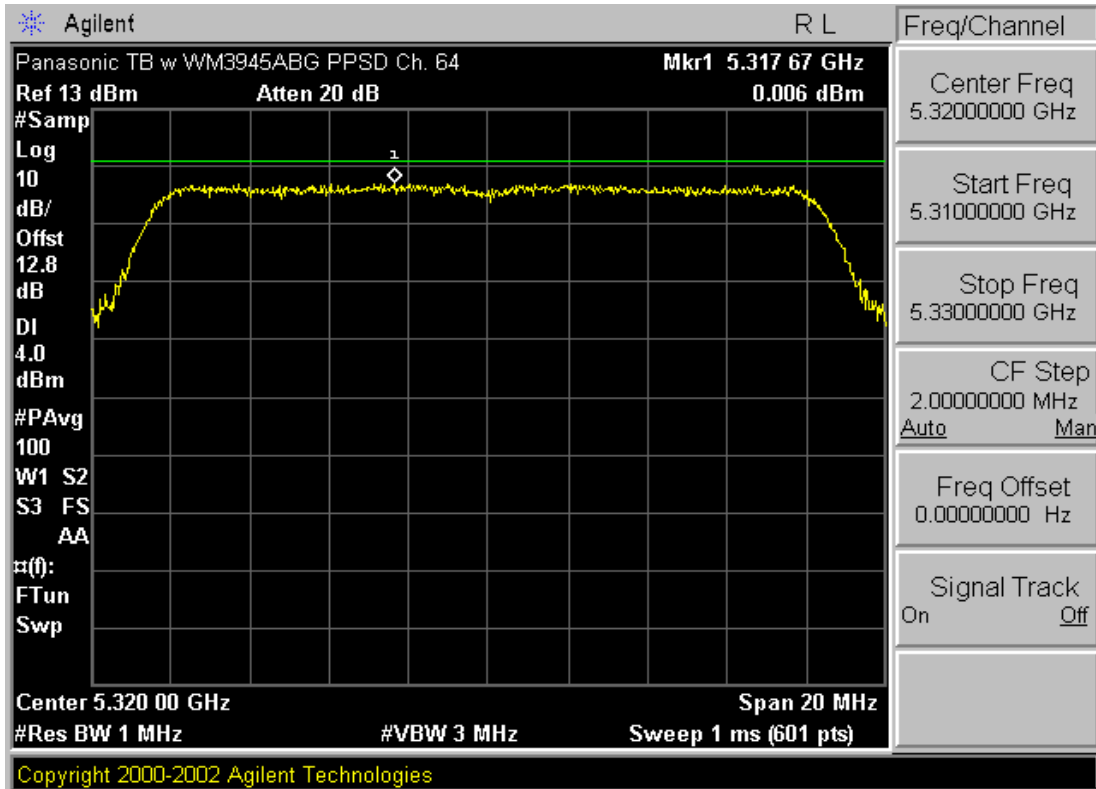
Plot 6-8. Peak Power Spectral Density Plot (802.11a (UNII) – Ch. 64)
