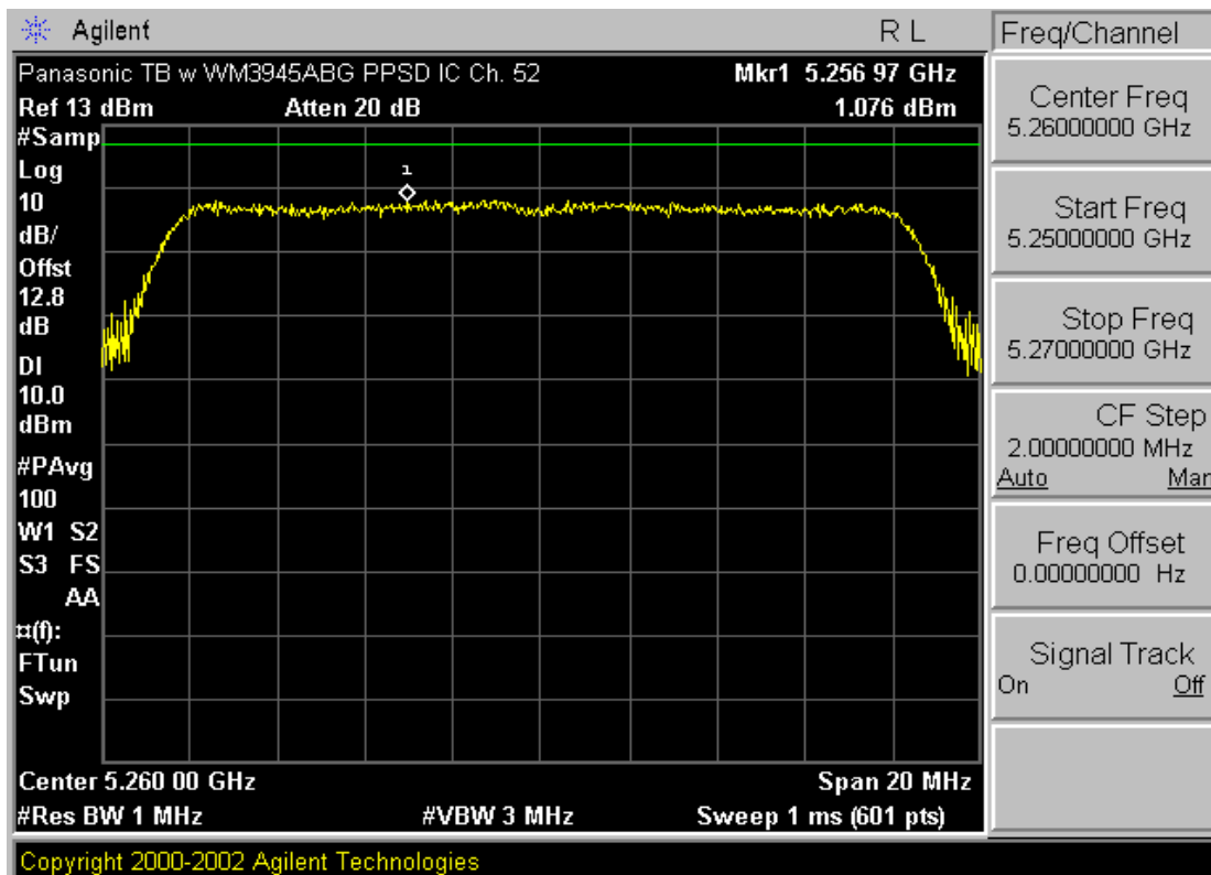
Plot 6-7. Peak Power Spectral Density Plot [Industry Canada] (802.11a (UNII) – Ch. 52)
