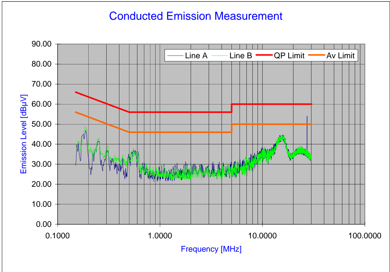
Plot 6-13. Line Conducted Plot with 802.11a (UNII Band)
