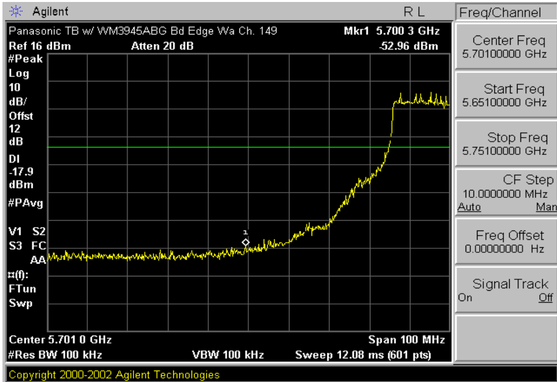
Plot 6-23. Band Edge Plot (802.11a – Ch. 149)
