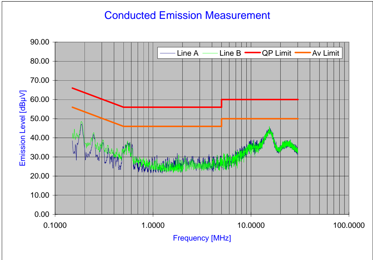
Plot 6-26. Line Conducted Plot with 802.11g
