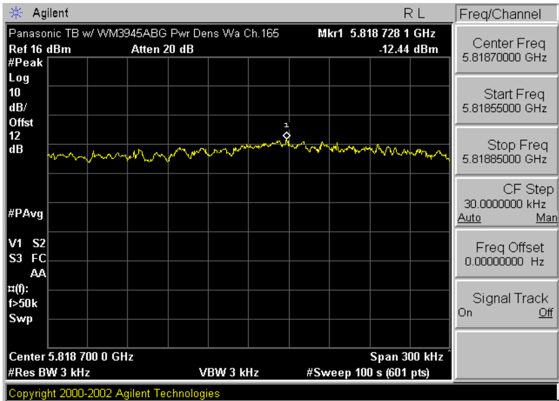
Plot 6-18. Power Spectral Density Plot (802.11a – Ch. 165)
