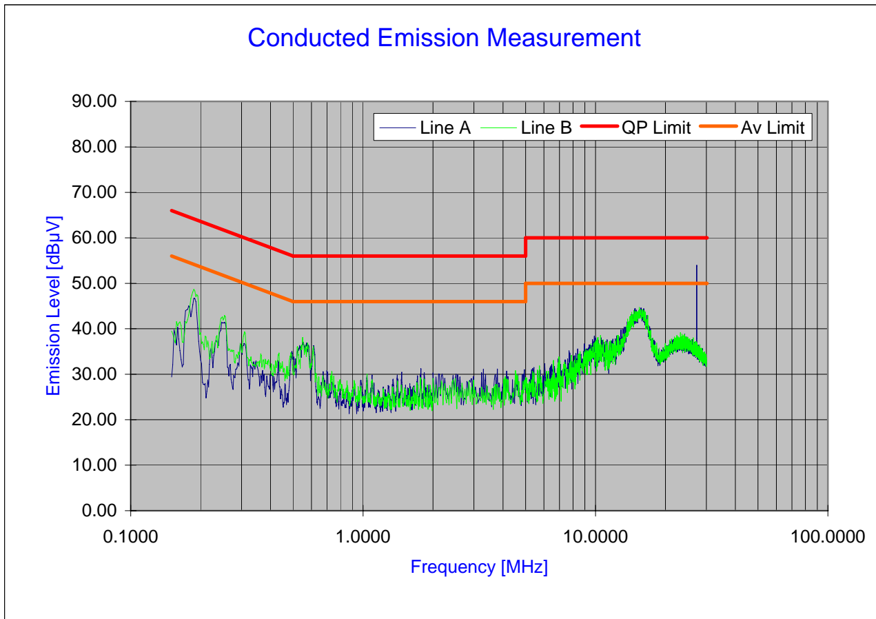
Plot 6-27. Line Conducted Plot with 802.11a
