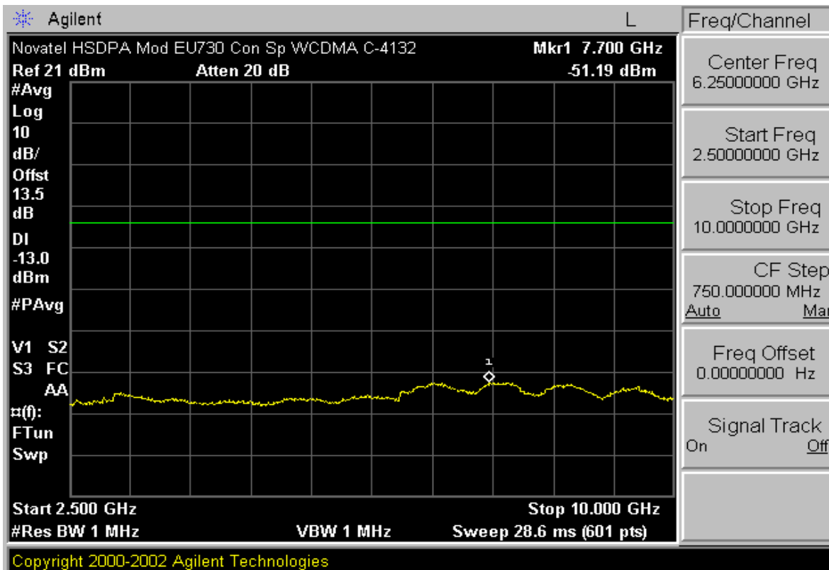
Plot A-2. Conducted Spurious Plot (Cellular WCDMA Mode – Ch. 4132)
