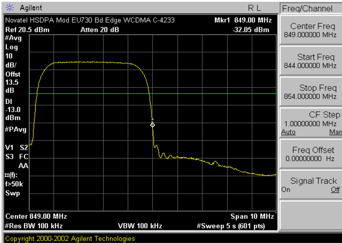
Plot A-11. Band Edge Plot (Cellular WCDMA Mode – Ch. 4233)
