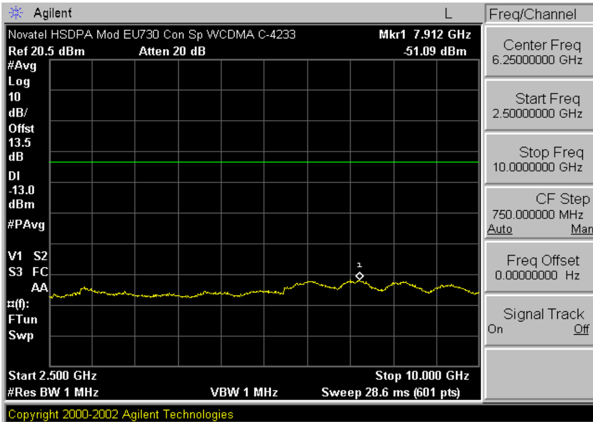
Plot A-10. Conducted Spurious Plot (Cellular WCDMA Mode – Ch. 4233)
