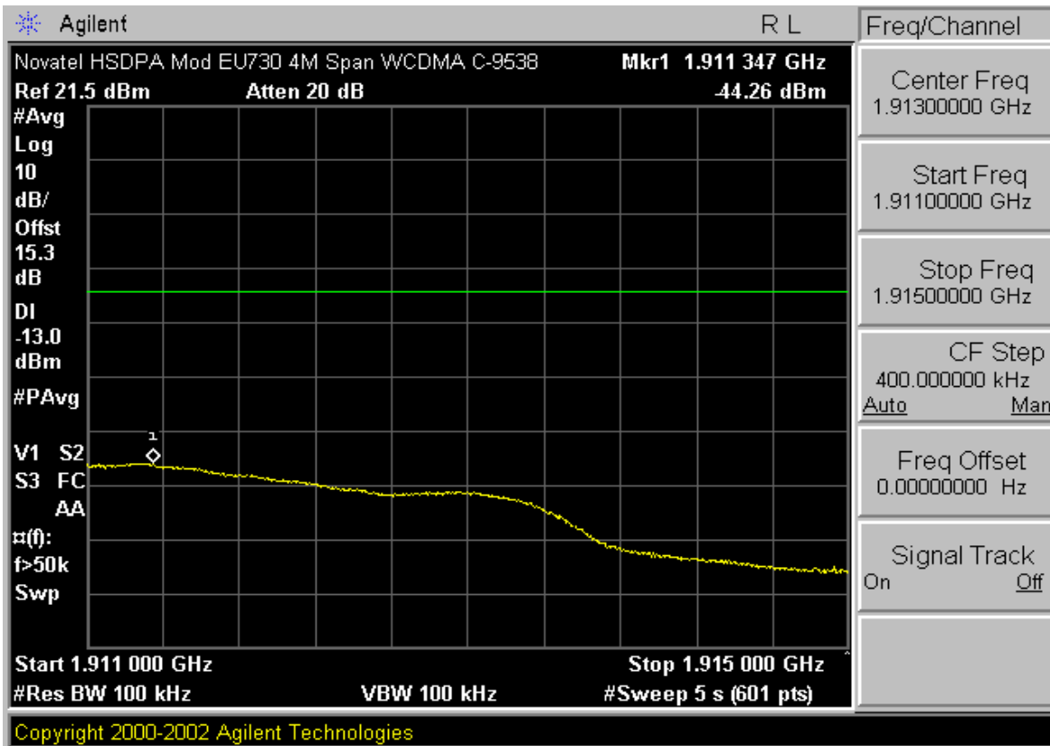
Plot A-24. 4MHz Span Plot (PCS WCDMA Mode – Ch. 9538)
