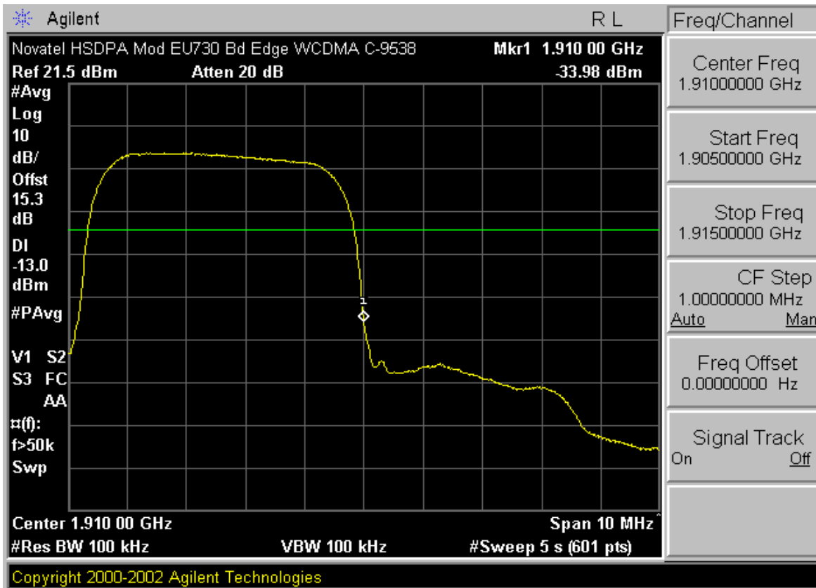
Plot A-23. Band Edge Plot (PCS WCDMA Mode – Ch. 9538)
