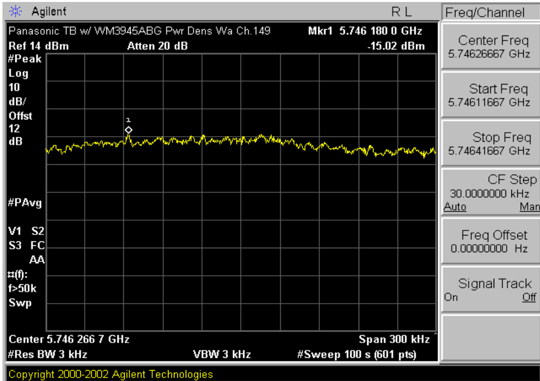
Plot 6-16. Power Spectral Density Plot (802.11a – Ch. 149)
