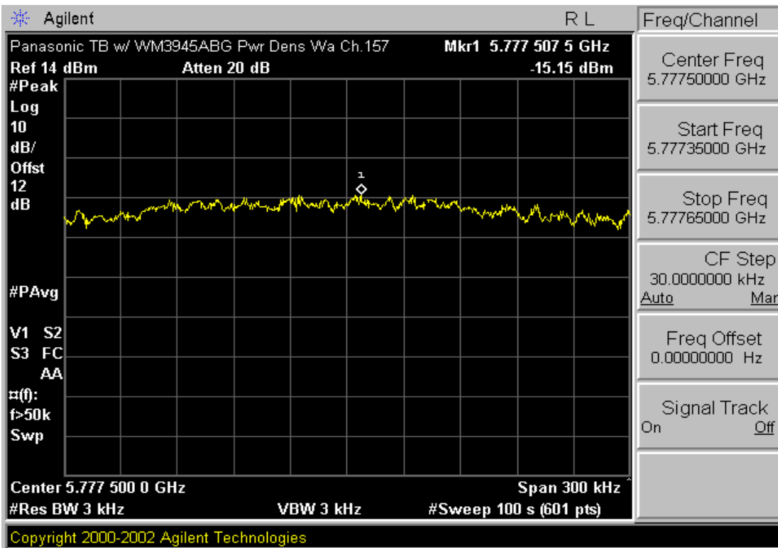
Plot 6-17. Power Spectral Density Plot (802.11a – Ch. 157)
