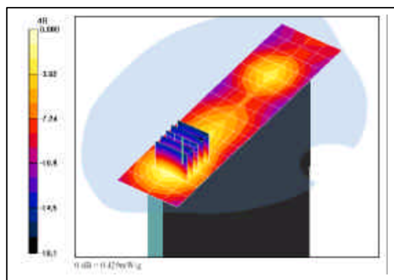
Bystander Position, LCD Flip, Ch. 661 w/ WLAN 802.11b, Ch. 06, 5.5 Mbps
