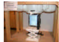
Figure 14.14 Body SAR Test Setup -- 802.11a, Bystander, LCD Open --
