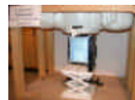
Figure 14.8 Body SAR Test Setup -- 802.11b, Bystander, LCD Open--
