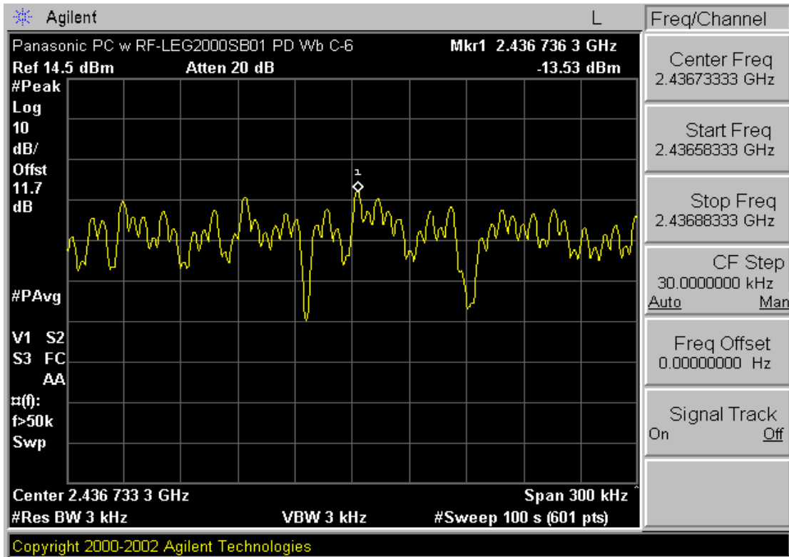
Plot 6-8. Power Spectral Density Plot (802.11b – Ch. 6)
